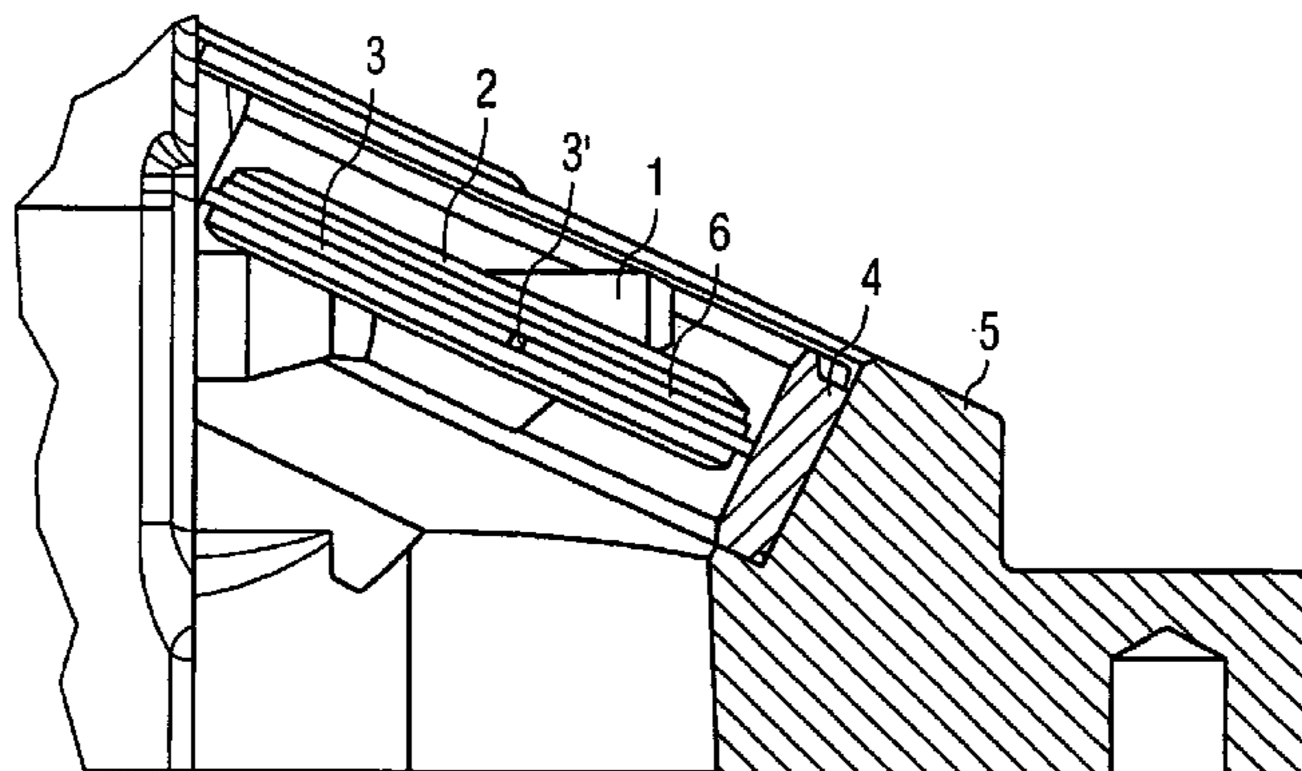
Detail A
