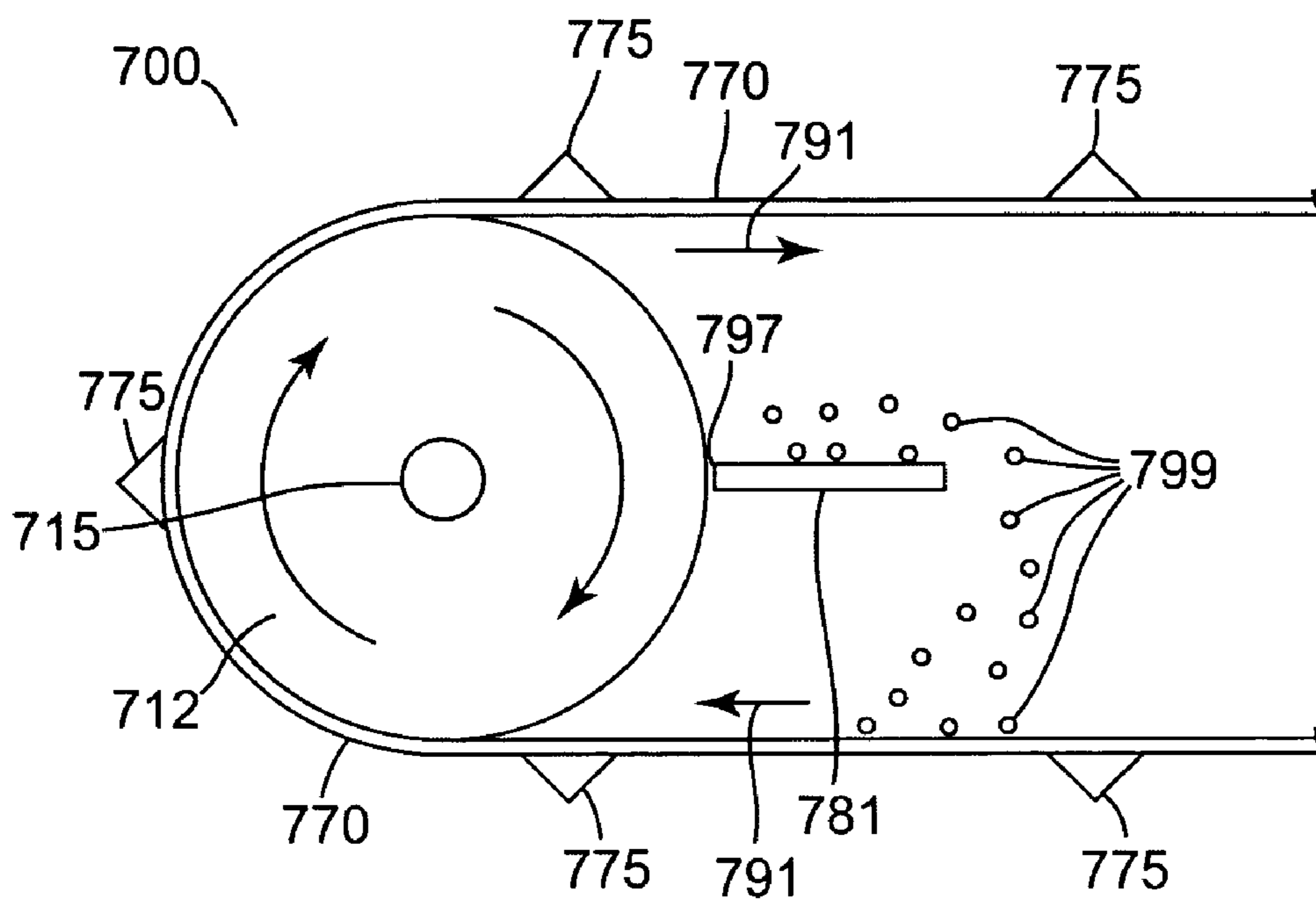
Fig. 7 PRIOR ART
