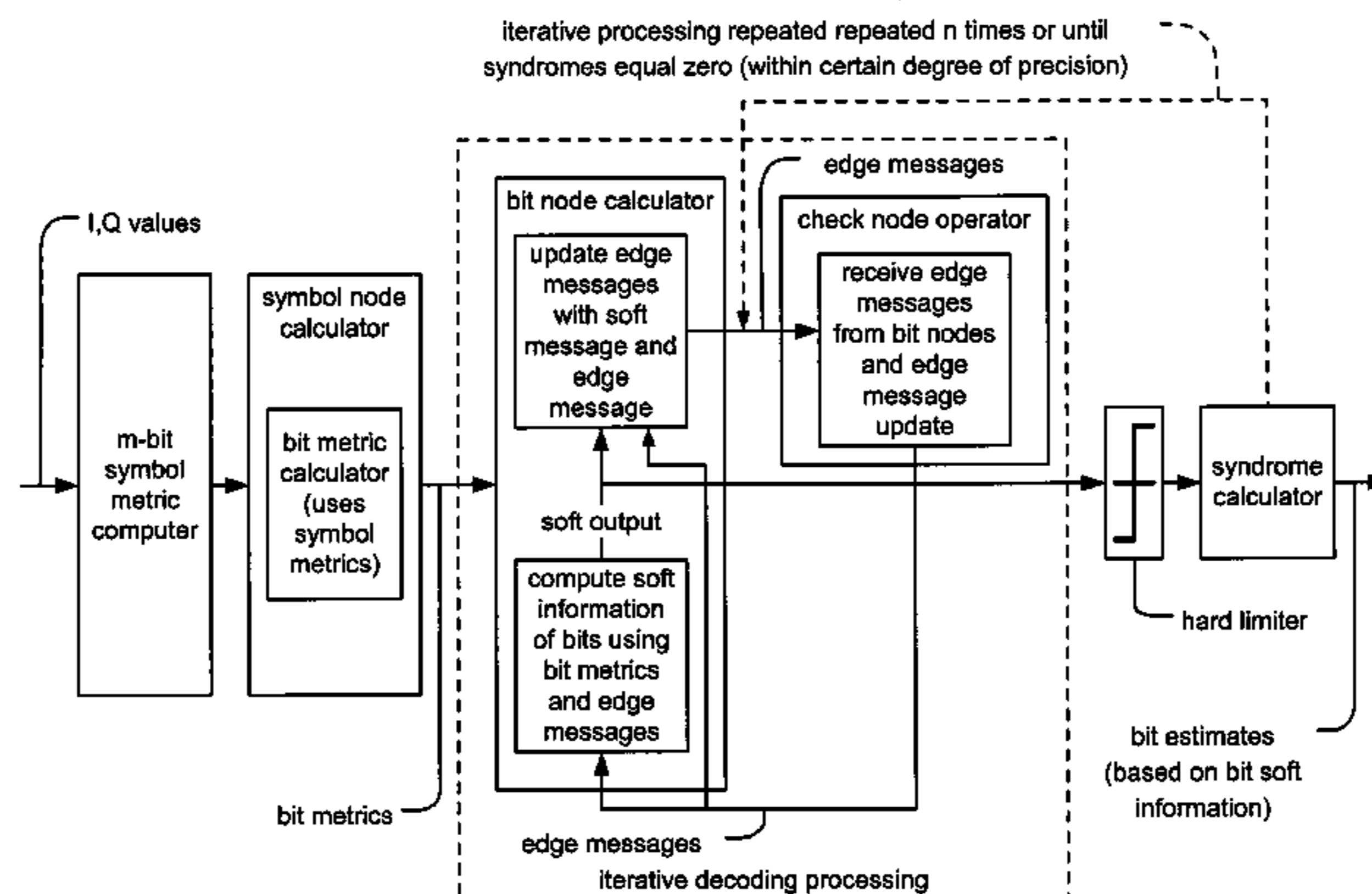
LDPC (Low Density Parity Check) coded modulation decoding functionality using bit metric
