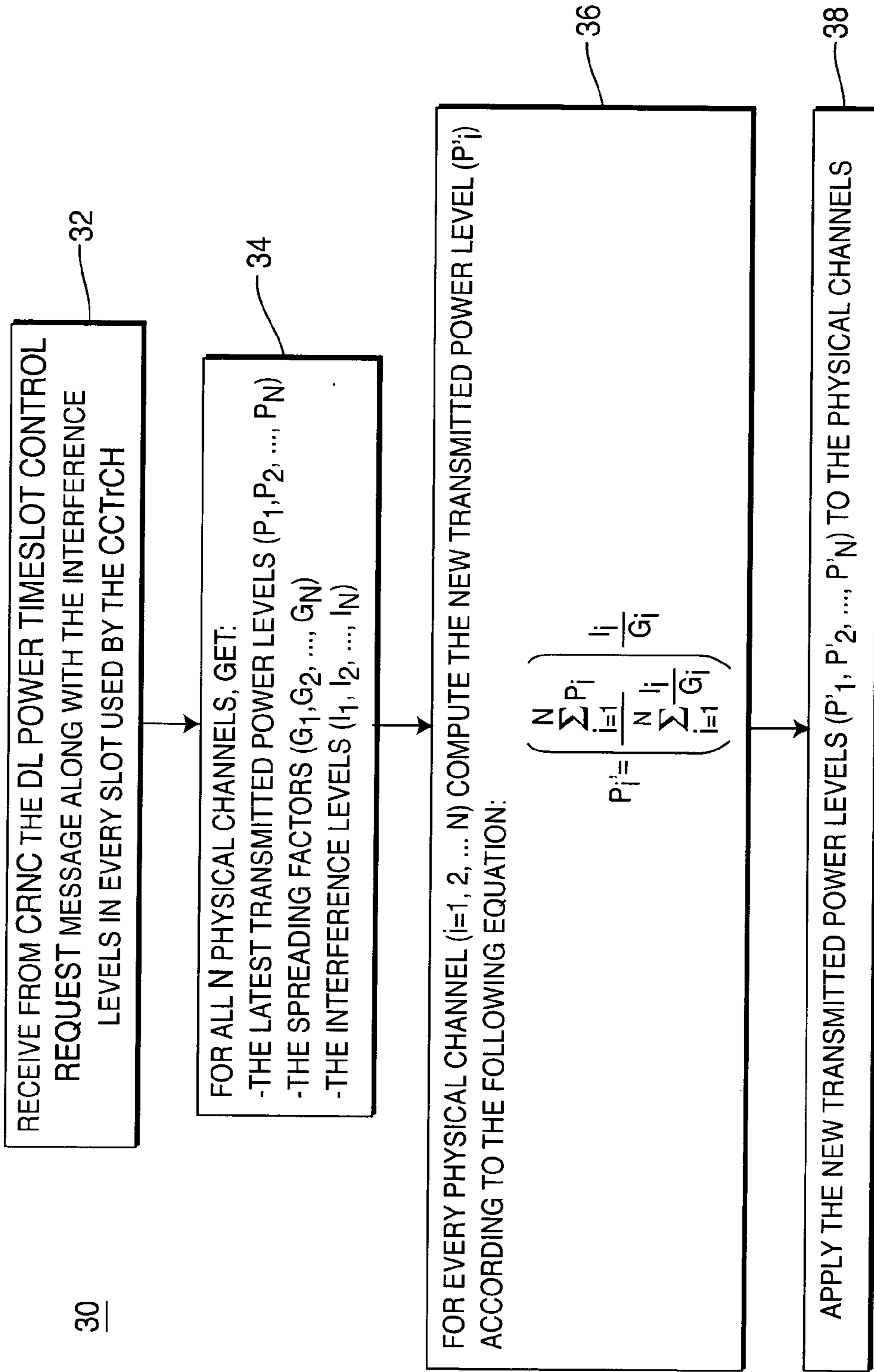
FIG. 4 PRIOR ART
