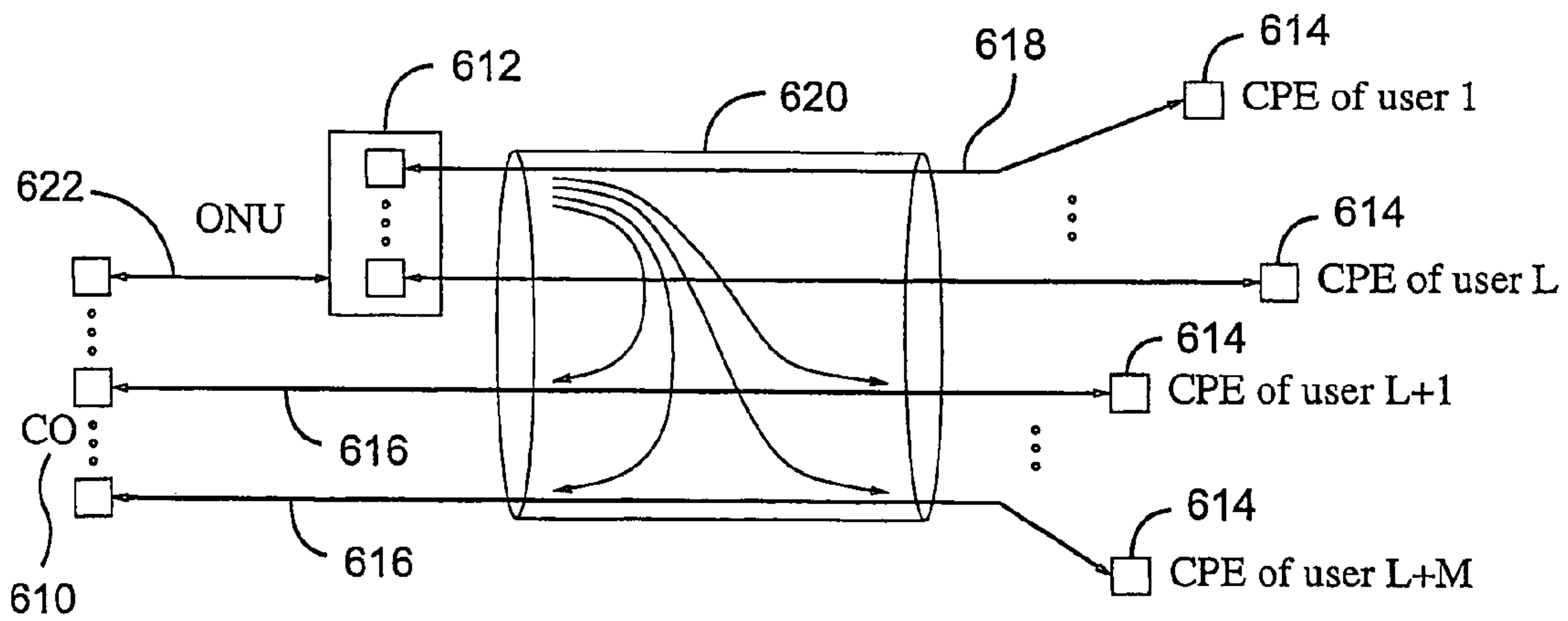
FIG. 6 Prior Art
