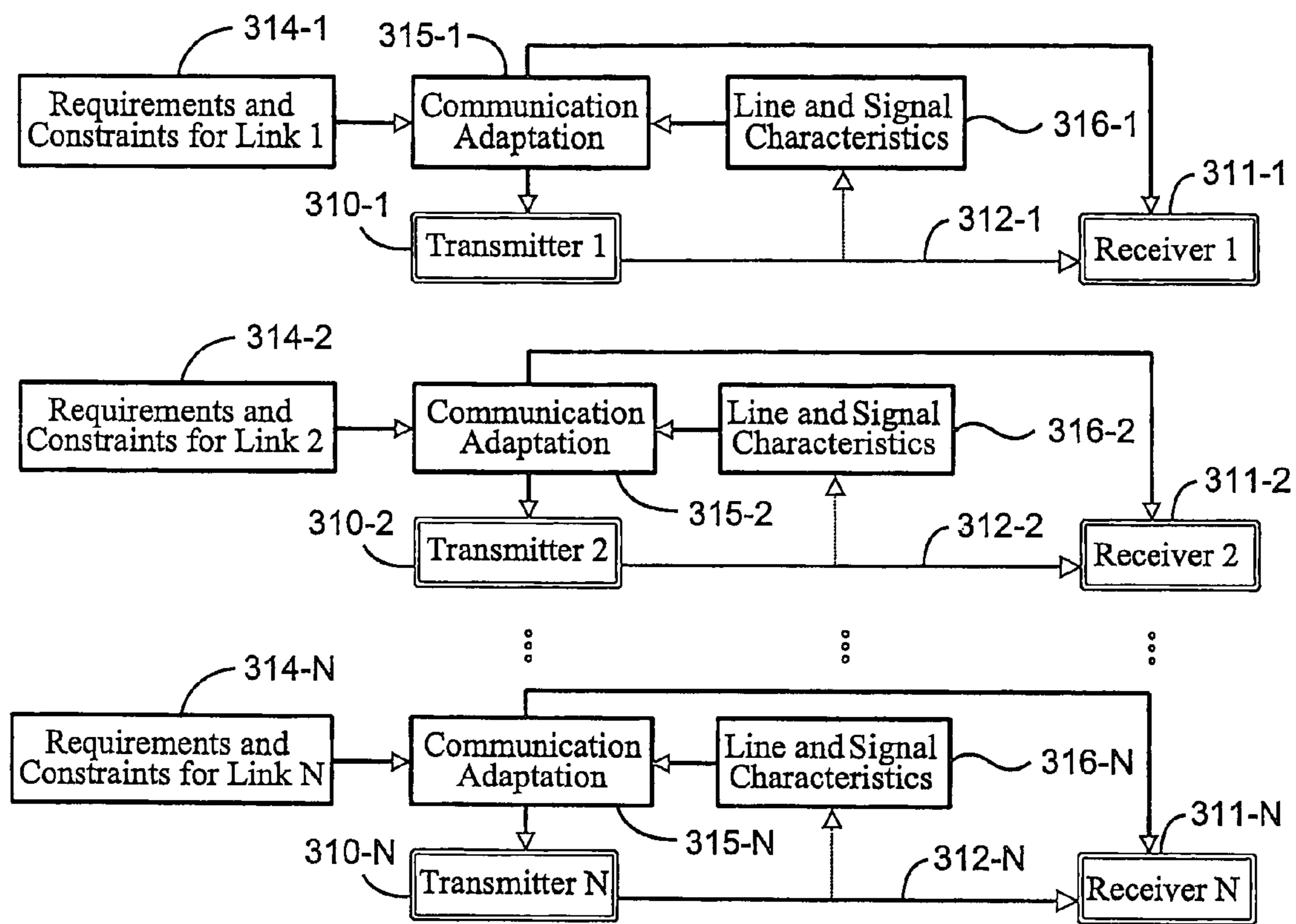
FIG. 3 Prior Art
