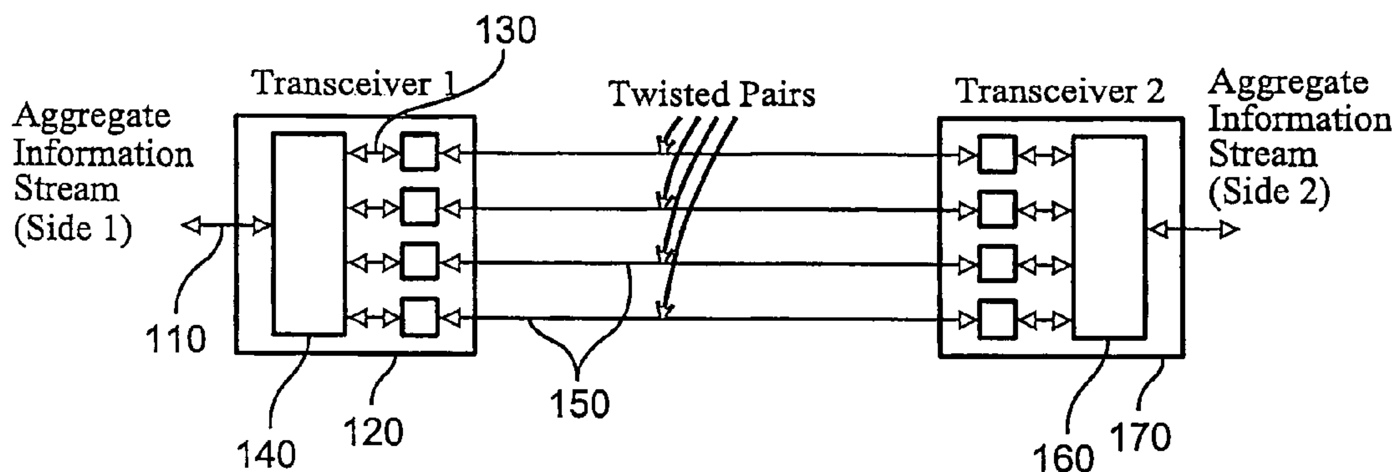
FIG. 1 Prior Art
