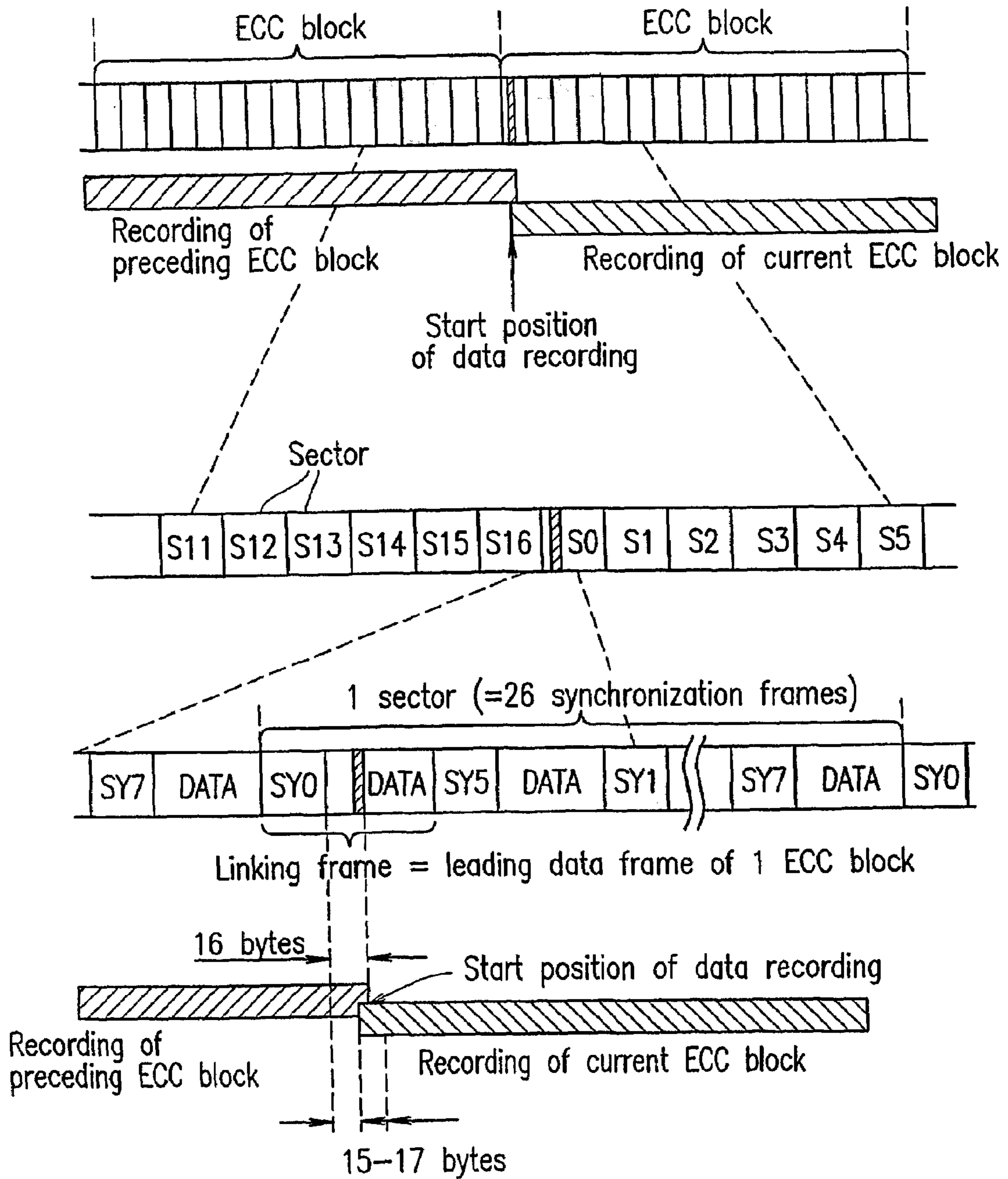
FIG. 44 CONVENTIONAL ART
