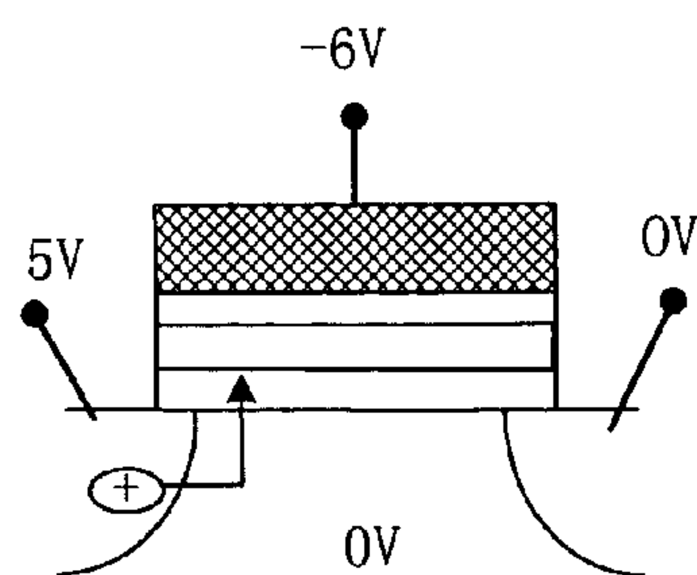
DATA PROGRAM (LEFT BIT)
