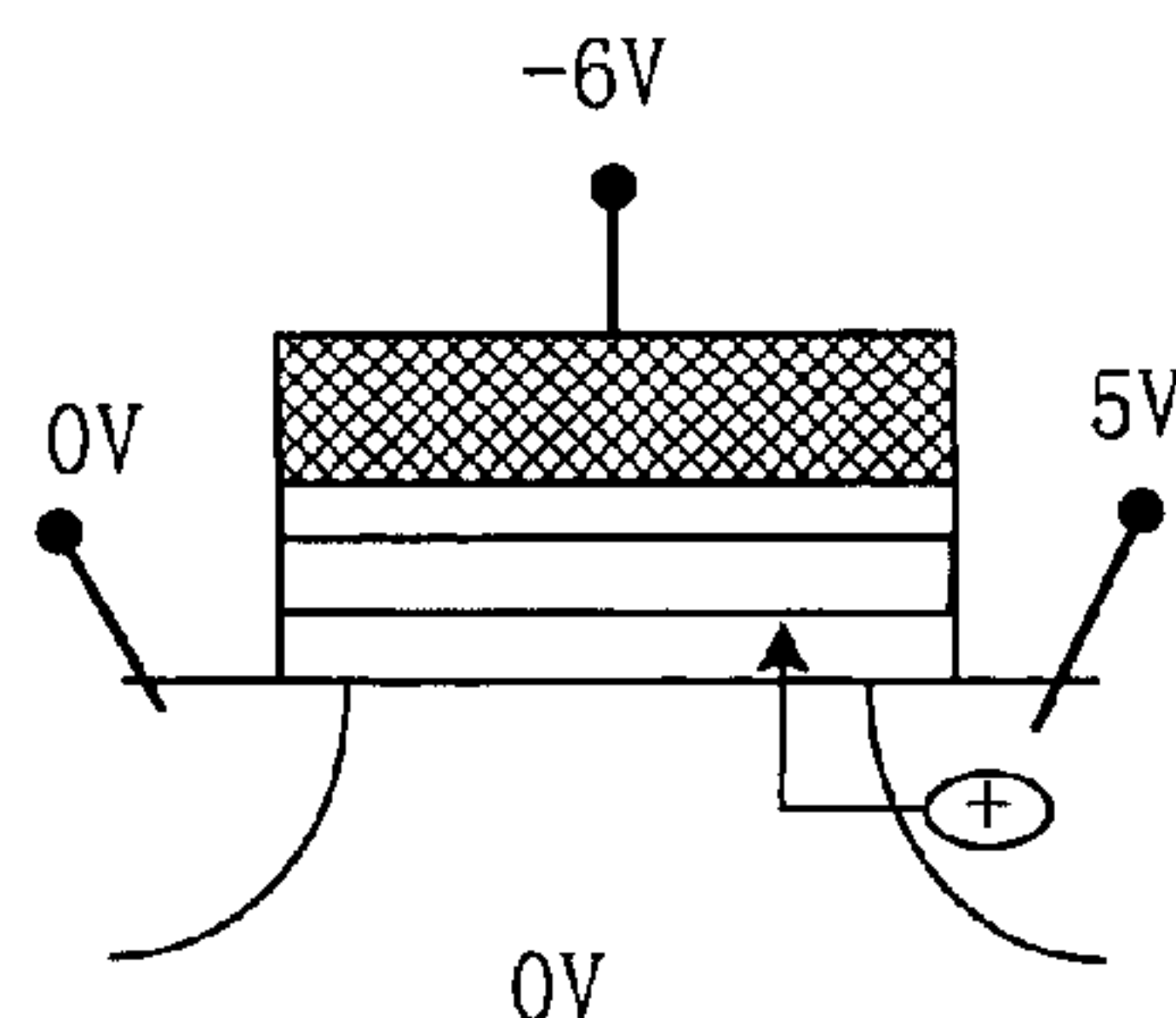
DATA PROGRAM (RIGHT BIT)
