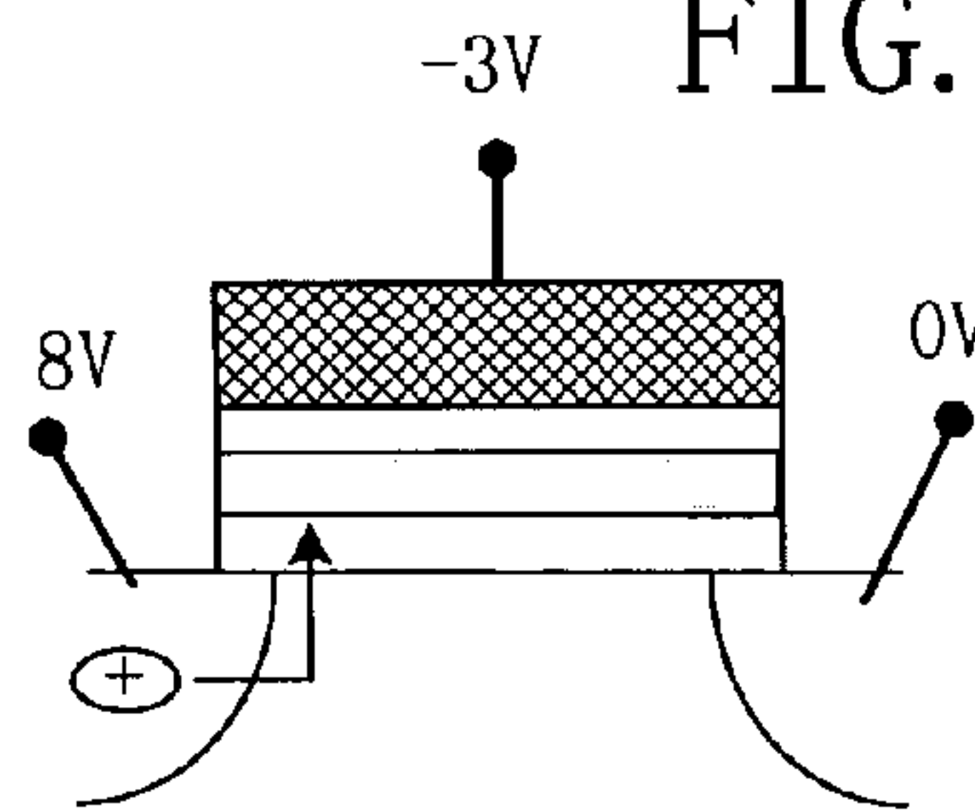
CODE ERASE (LEFT BIT)
