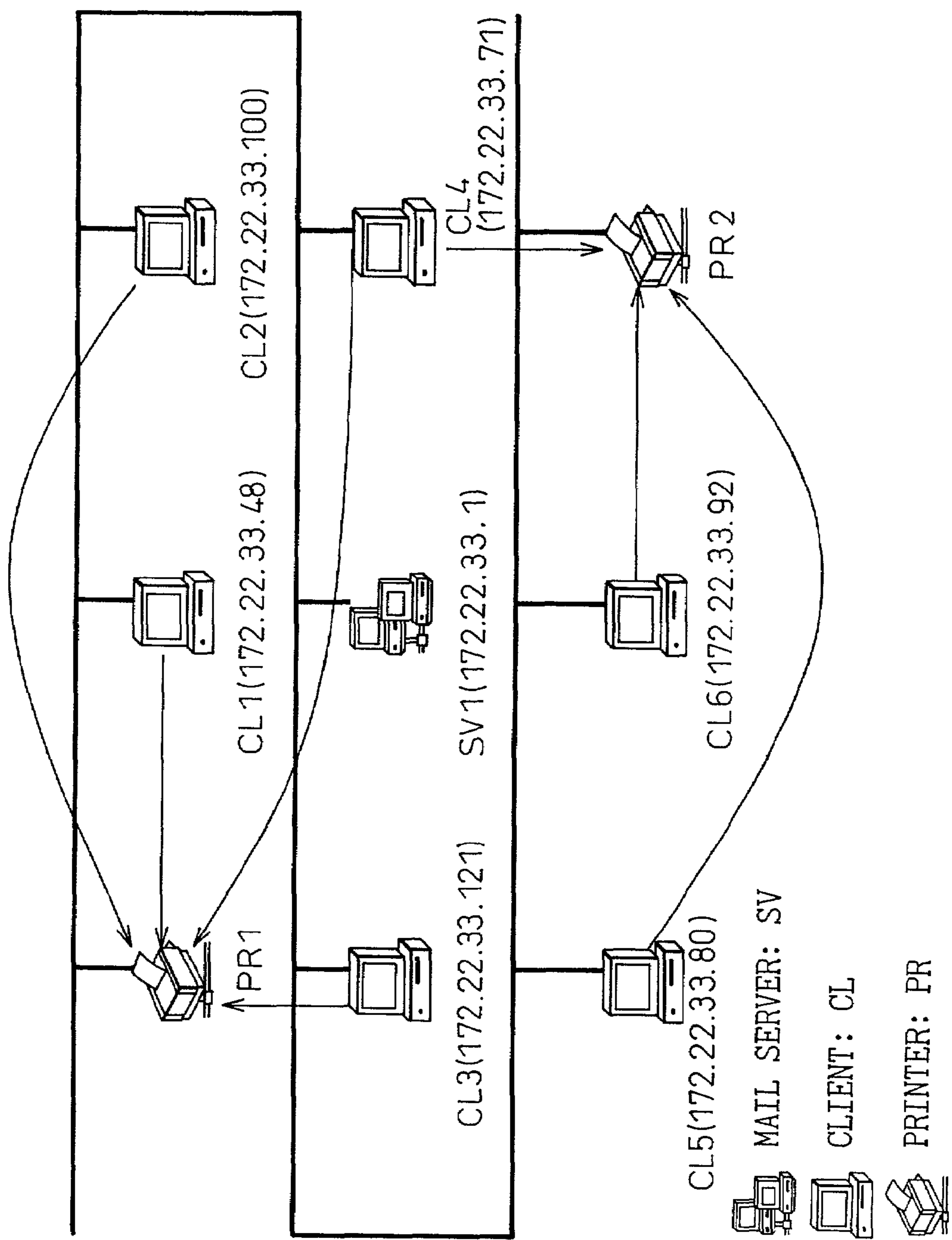
Fig.4 PRIOR ART
