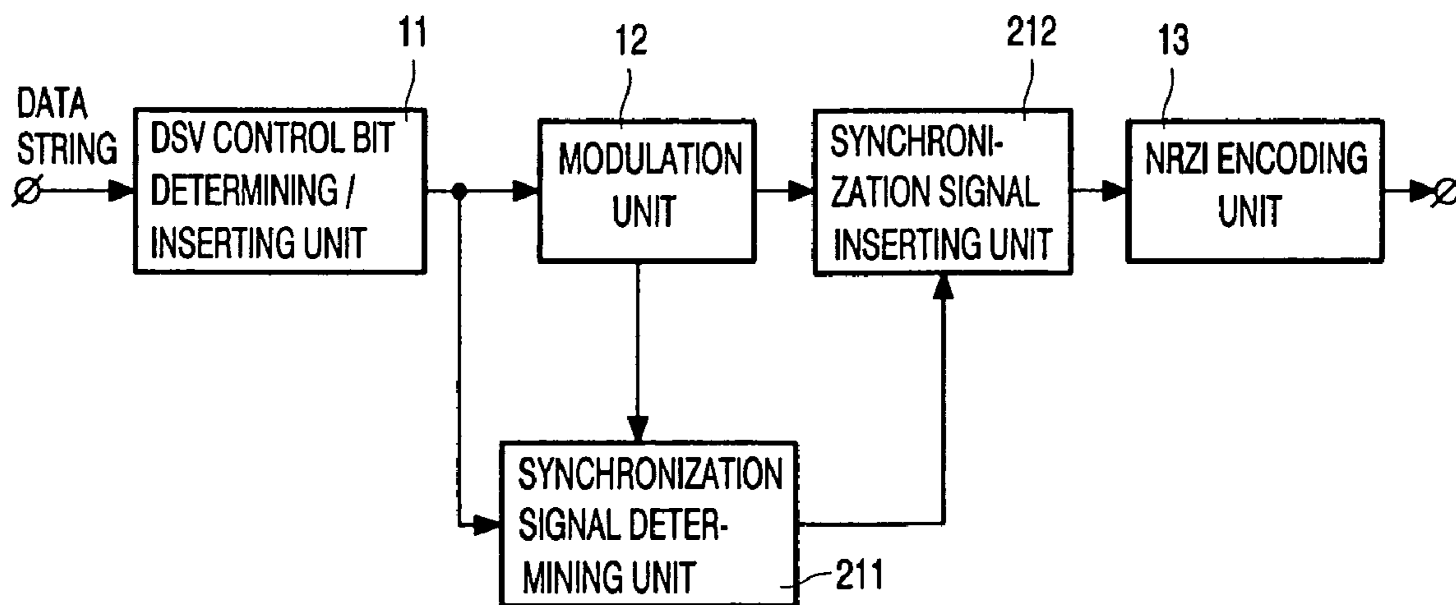
MODULATION APPARATUS 1
