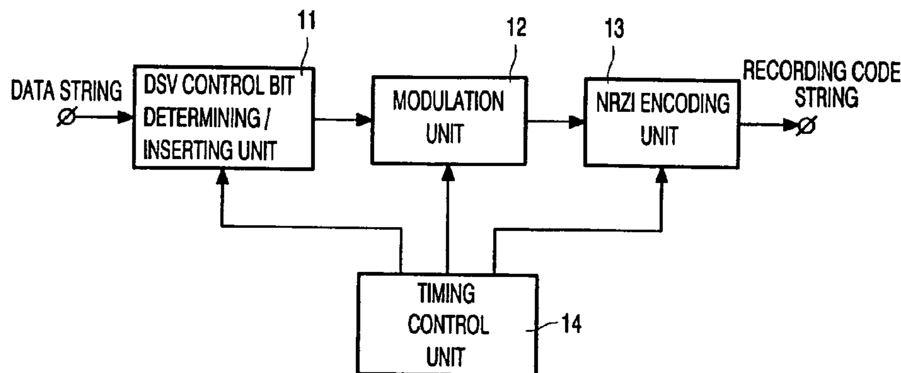
MODULATION APPARATUS 1
