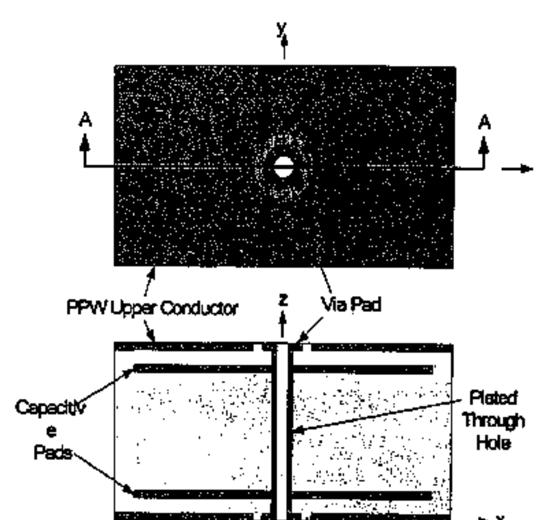
Plated through holes may be used in the fabrication of resonant vias as illustrated here for an internal I resonant via.
