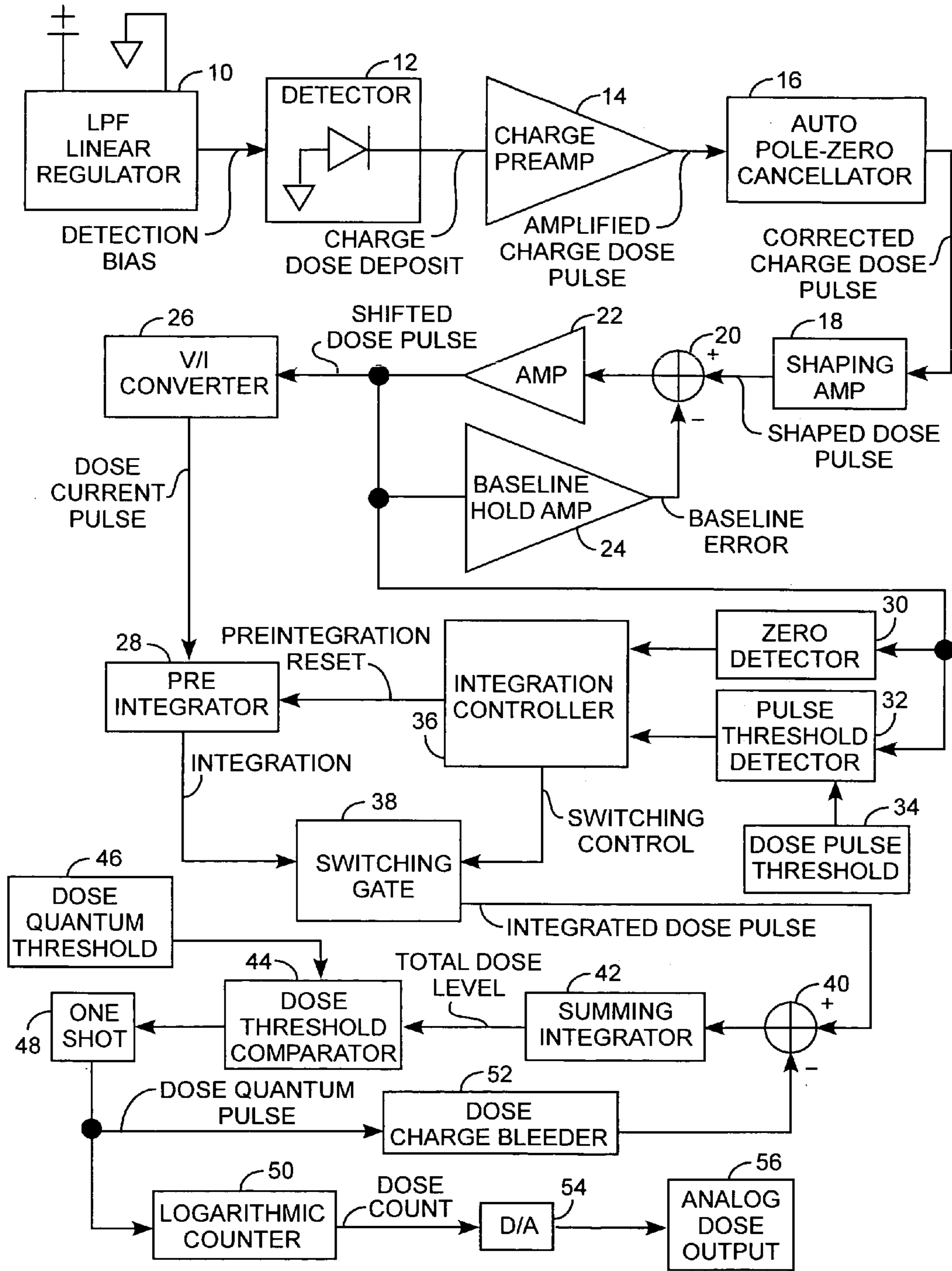
RADIATION DOSIMETER
