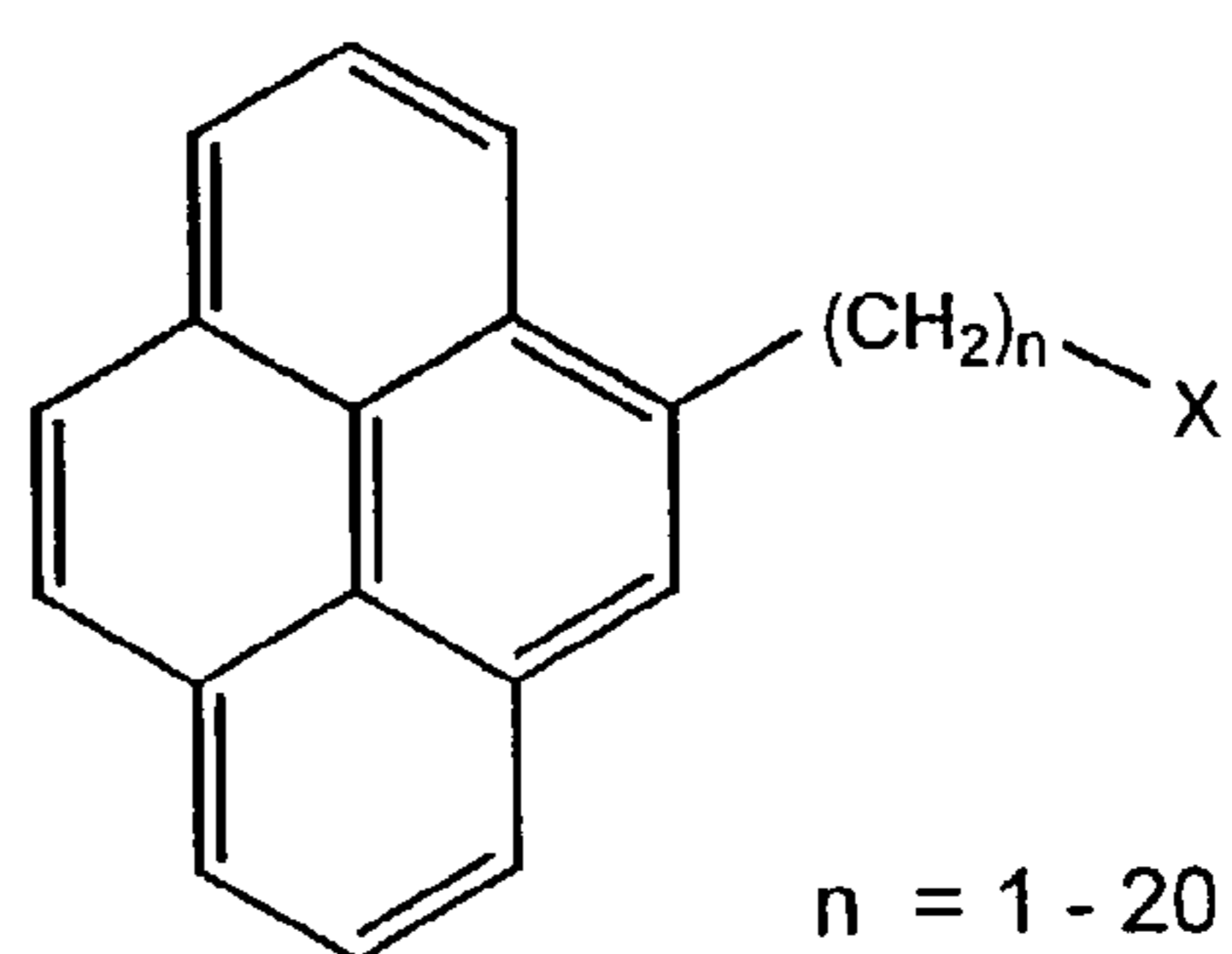
DYE126
