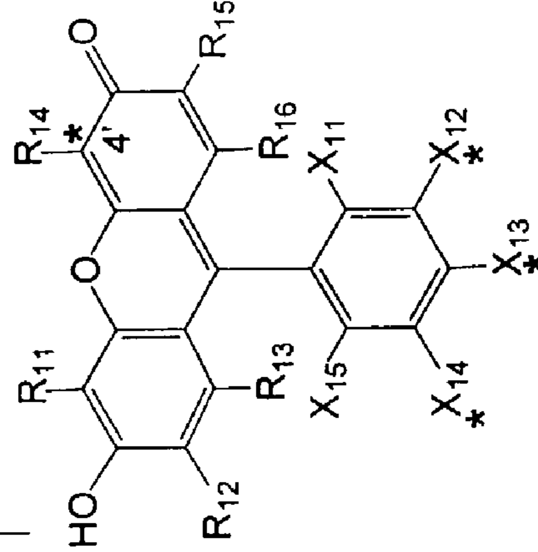
FLUORESCHEIN
