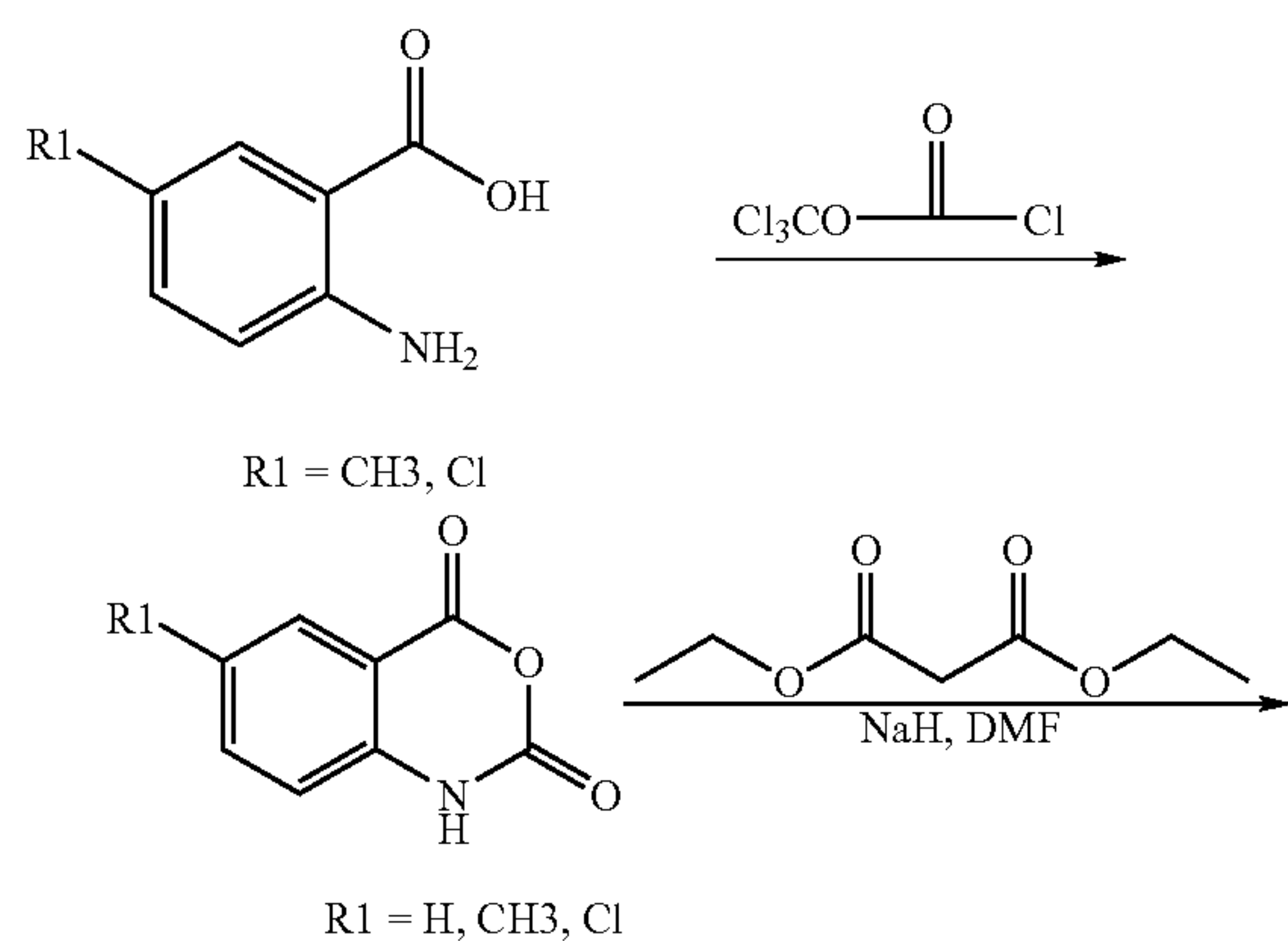
Reaction Scheme 21
