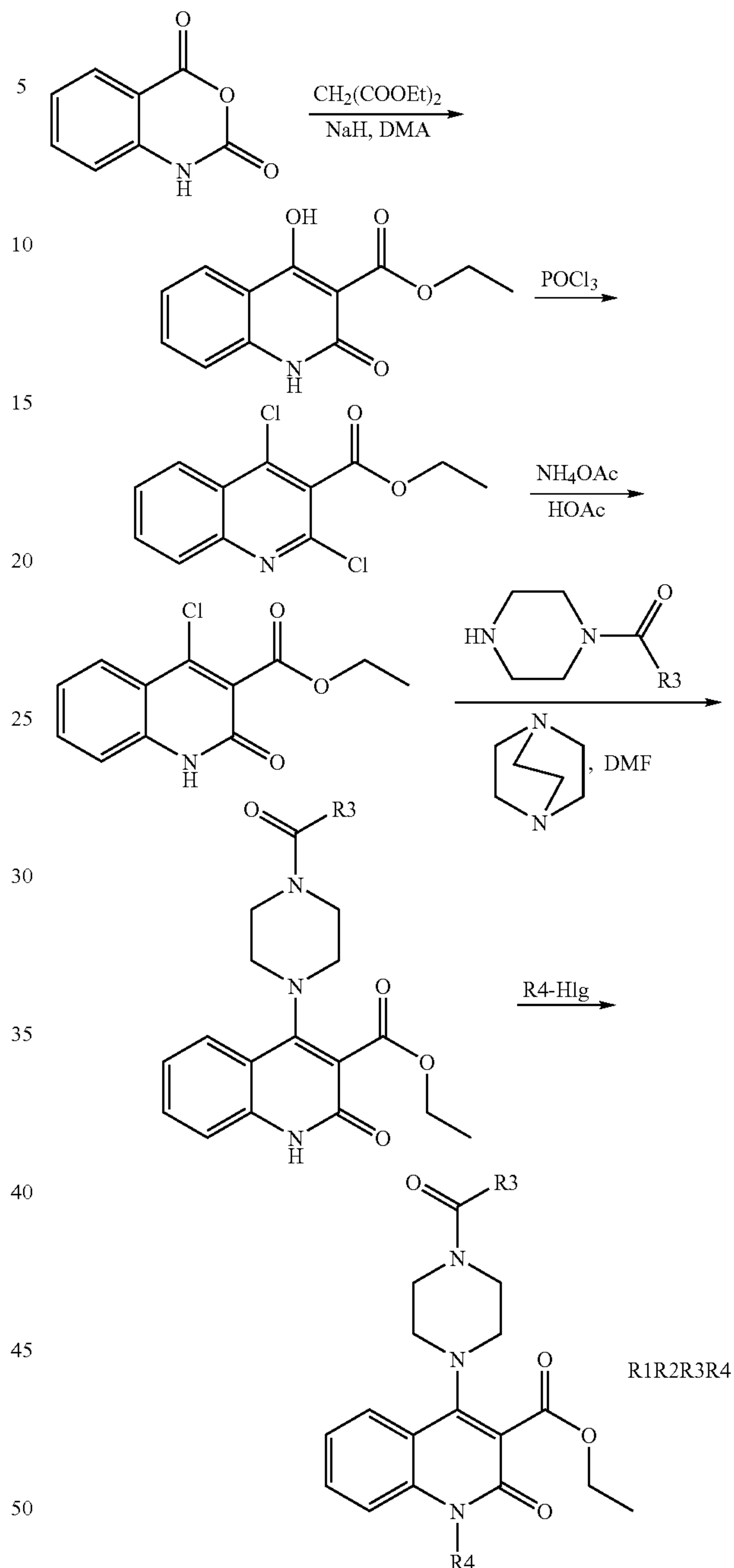
Compound 343
