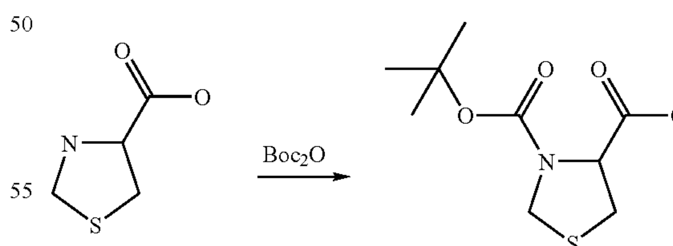
Reaction Scheme 20
