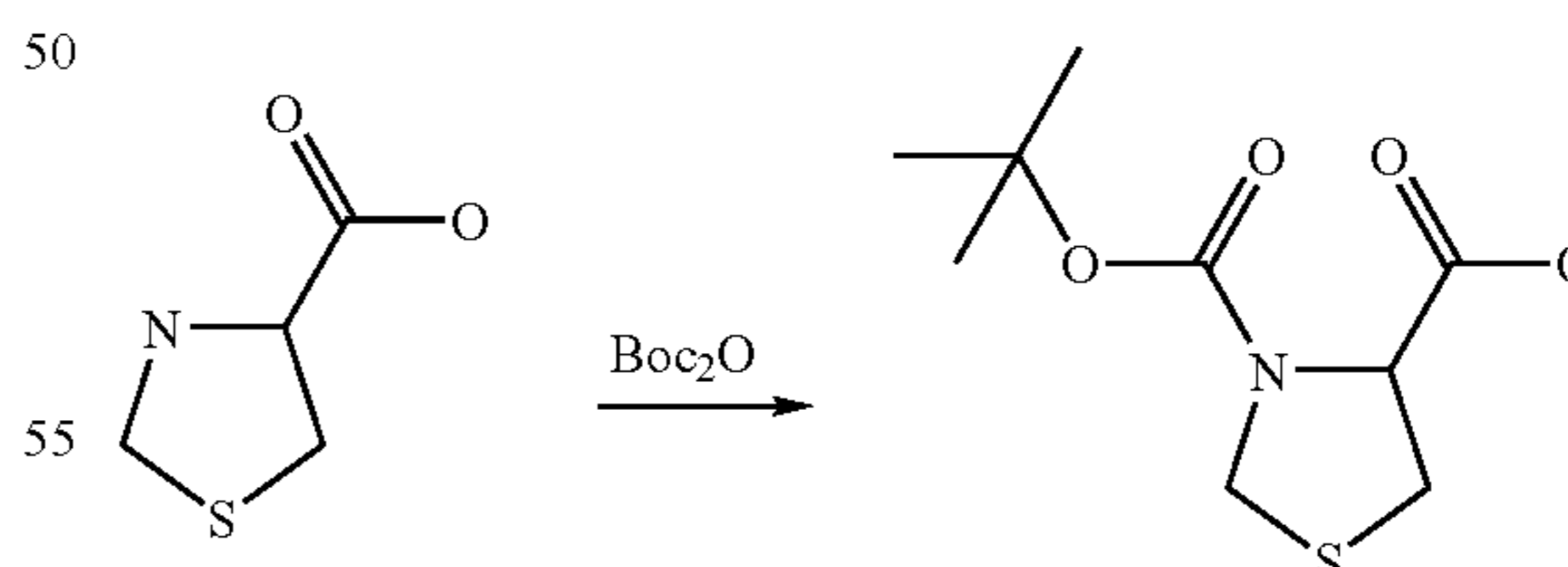
Reaction Scheme 20
