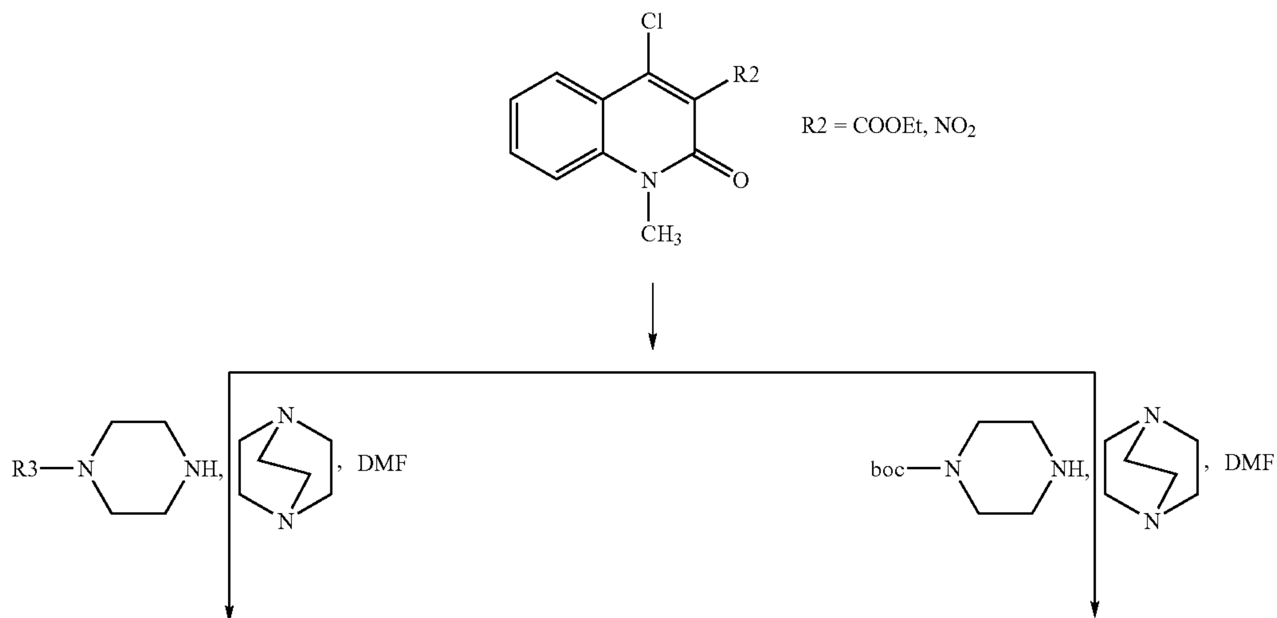
Reaction Scheme 10
