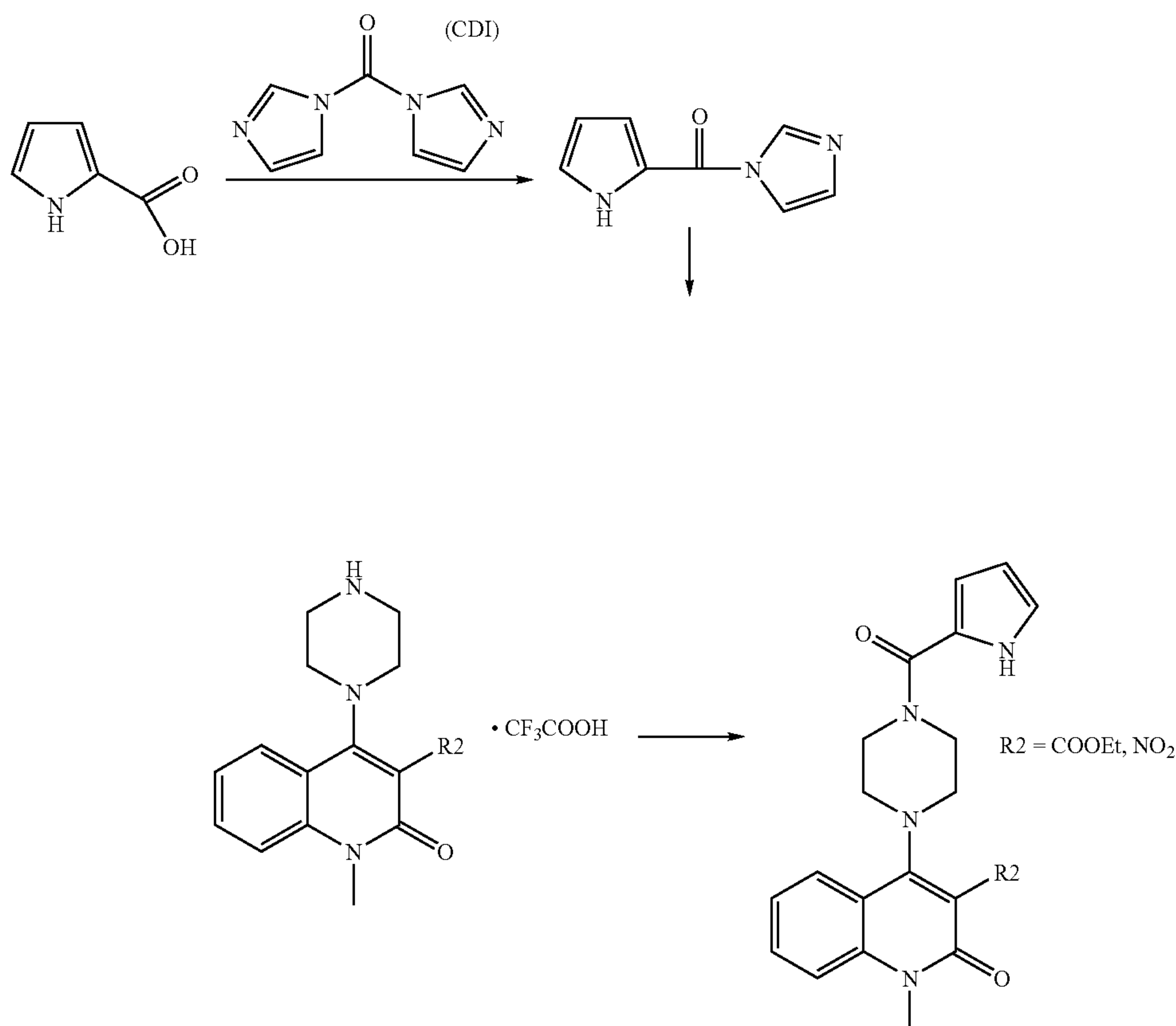
Reaction Scheme 17
