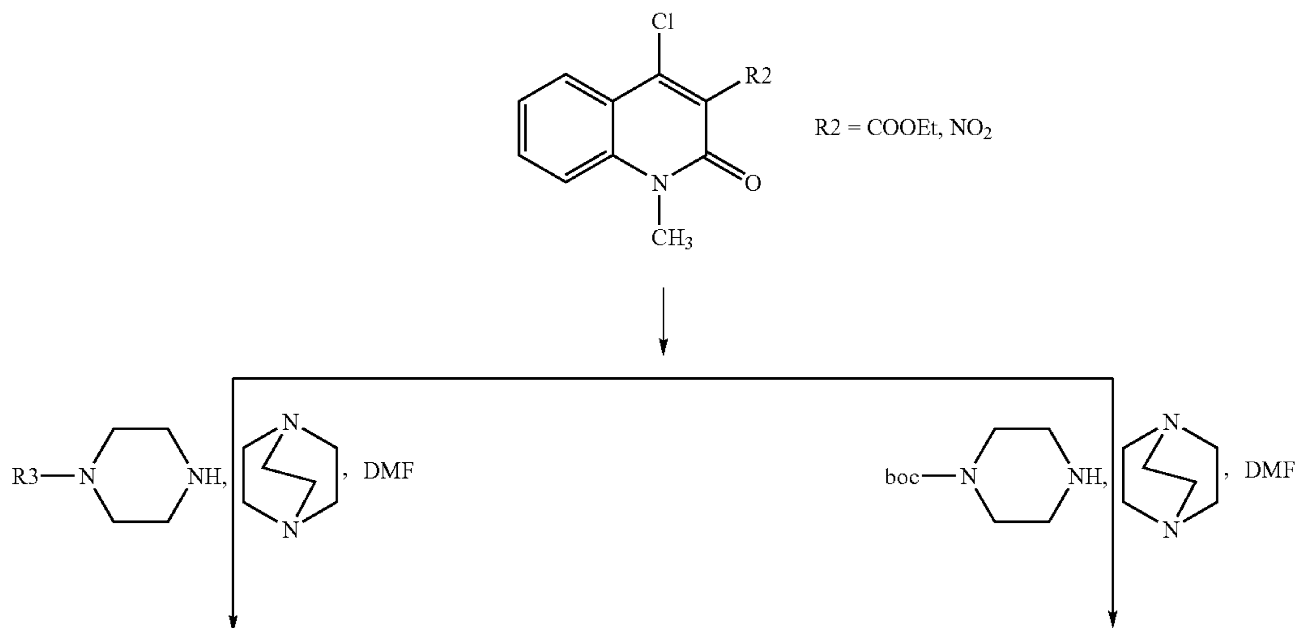
Reaction Scheme 10
