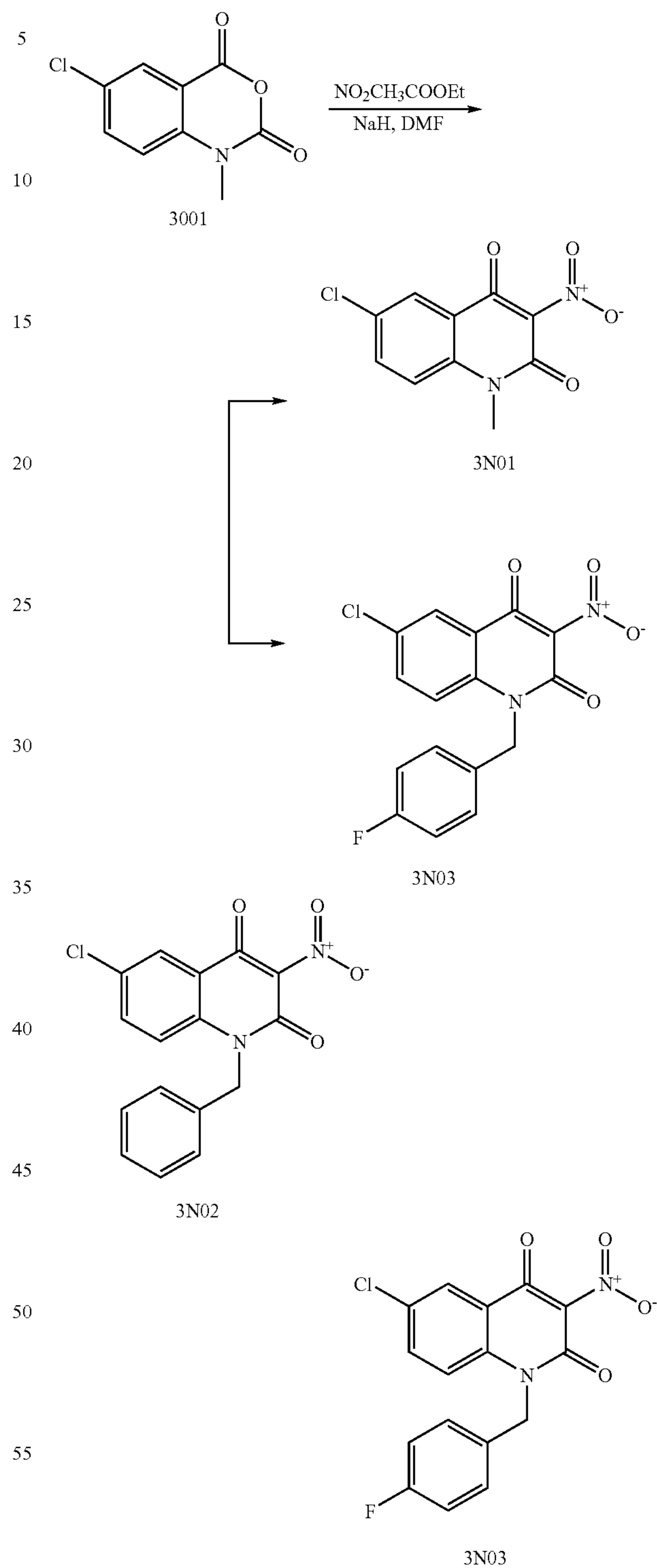
Reaction Scheme 26
