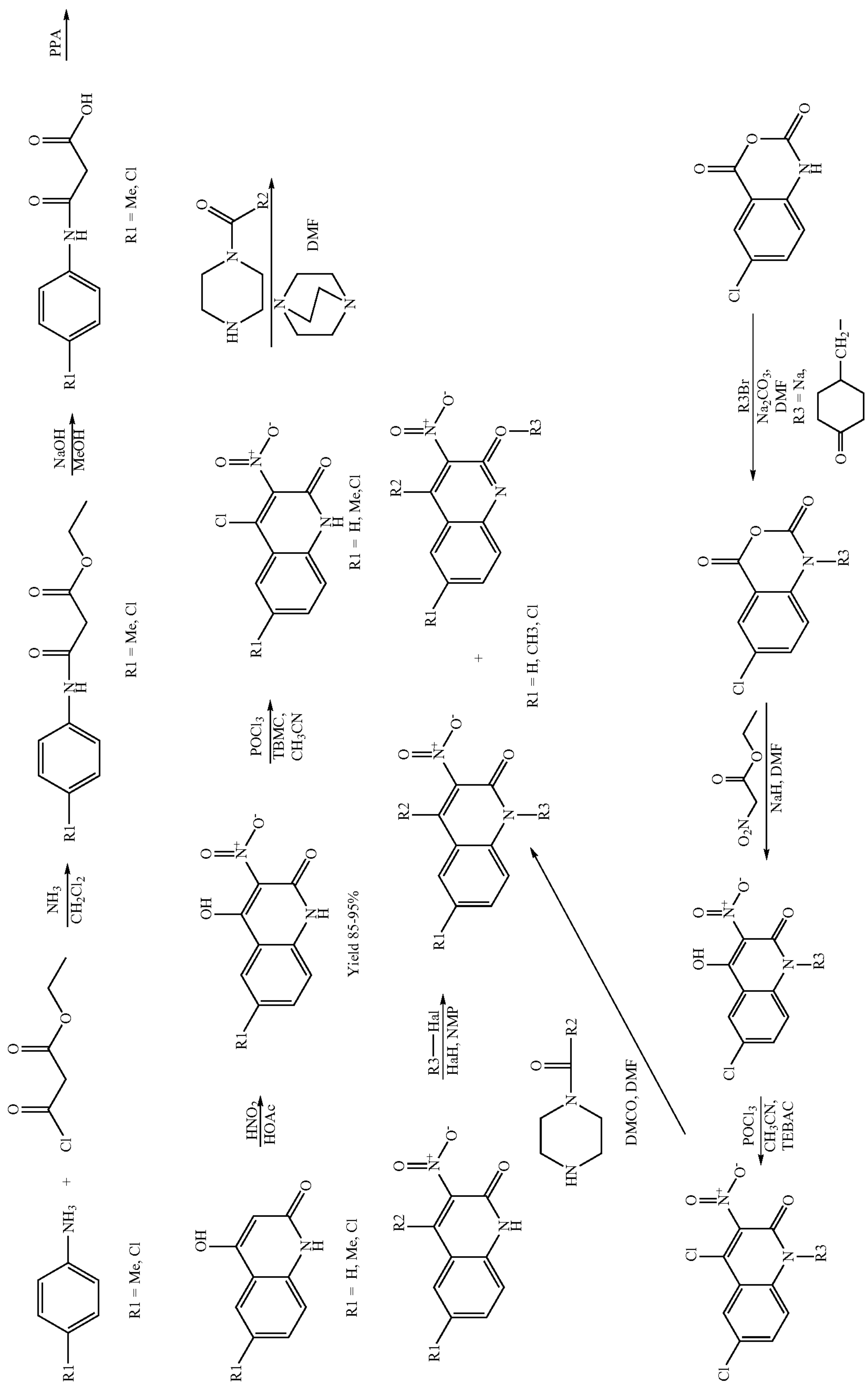
Reaction Scheme 22
