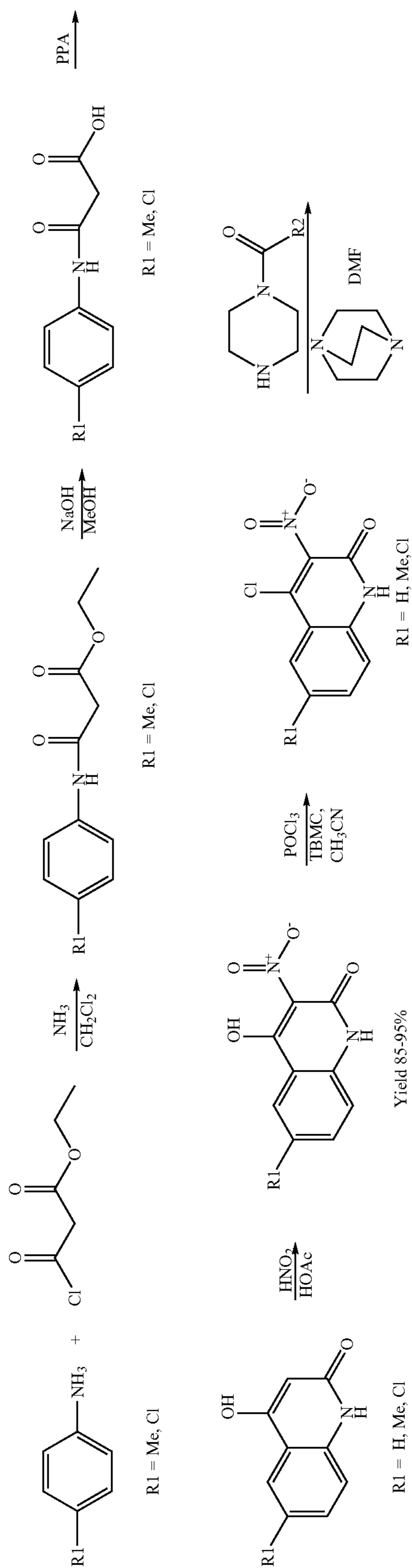
Reaction Scheme 22
