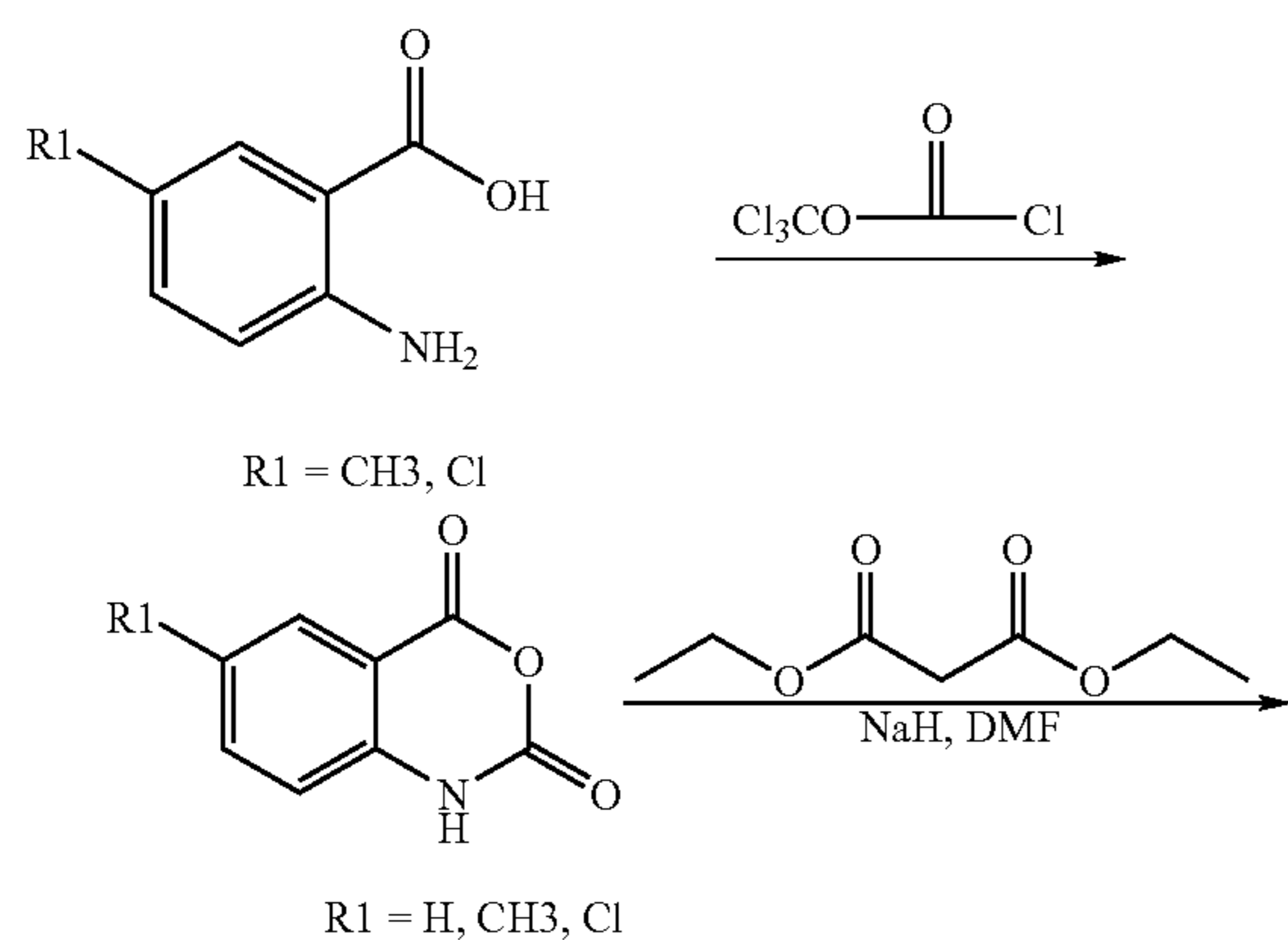
Reaction Scheme 21
