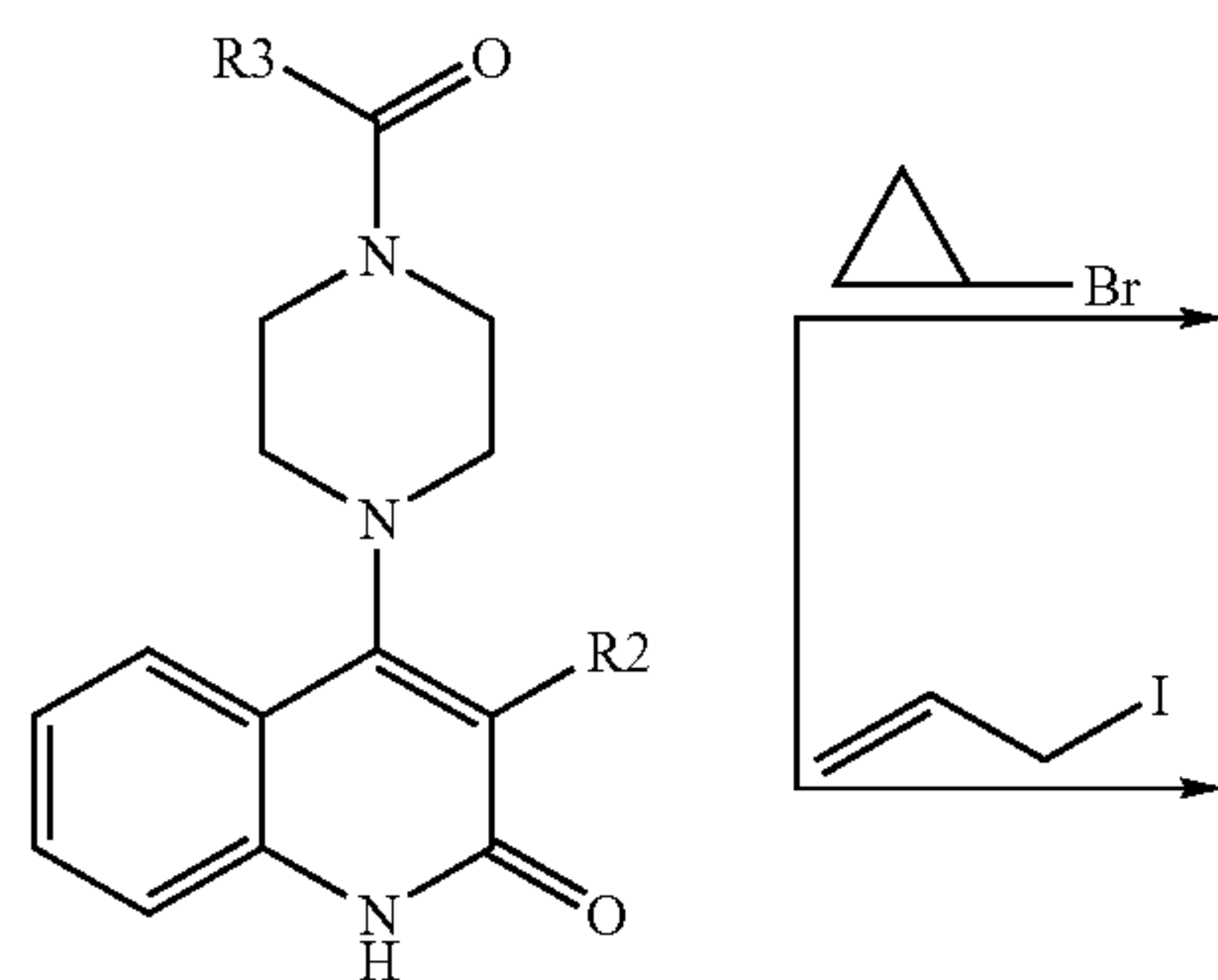
Reaction Scheme 8
