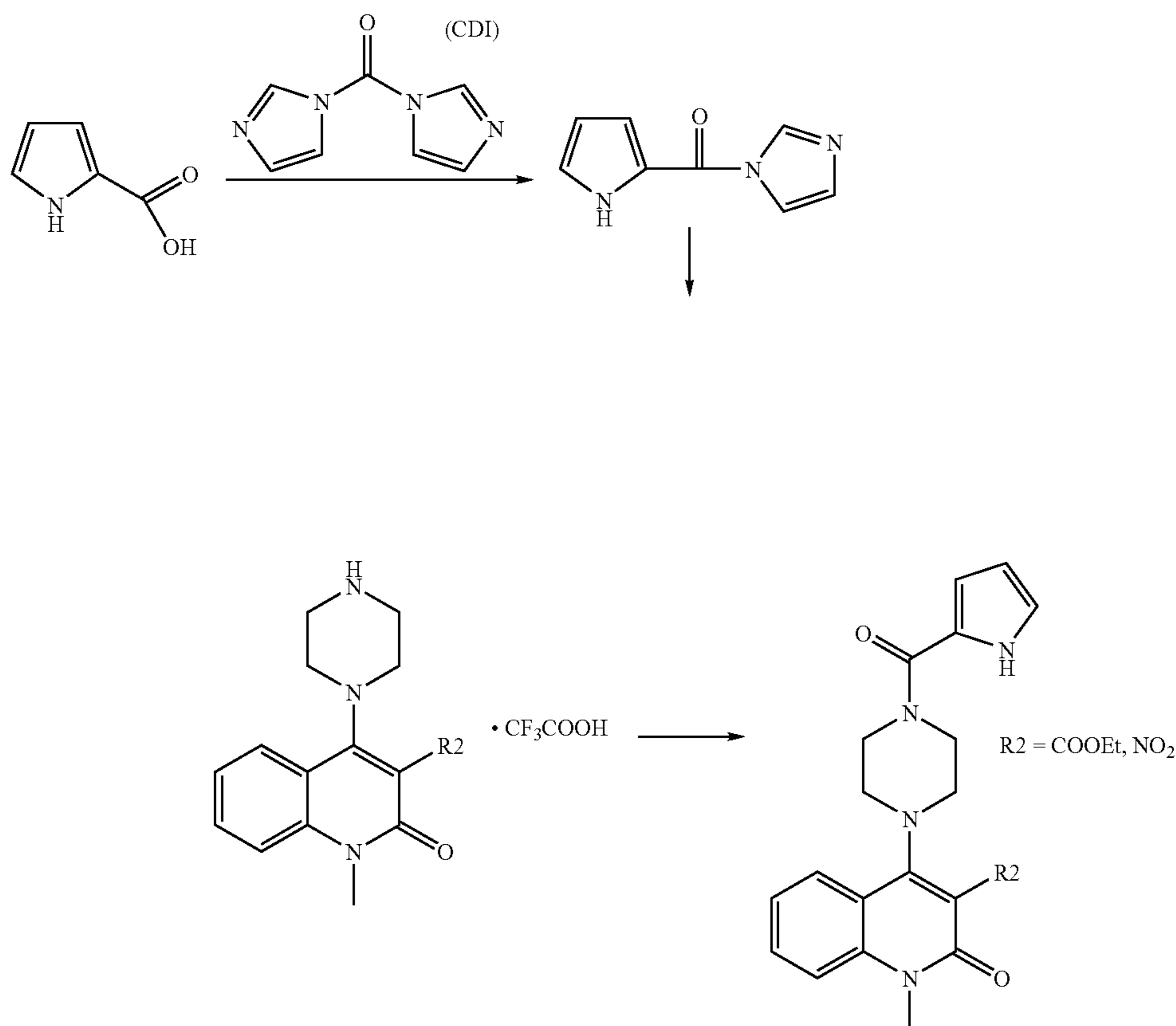
Reaction Scheme 17
