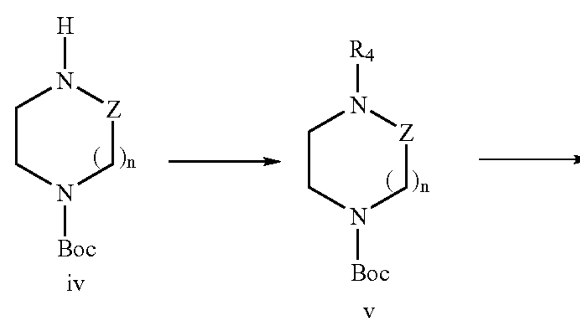
Reaction Scheme 2
