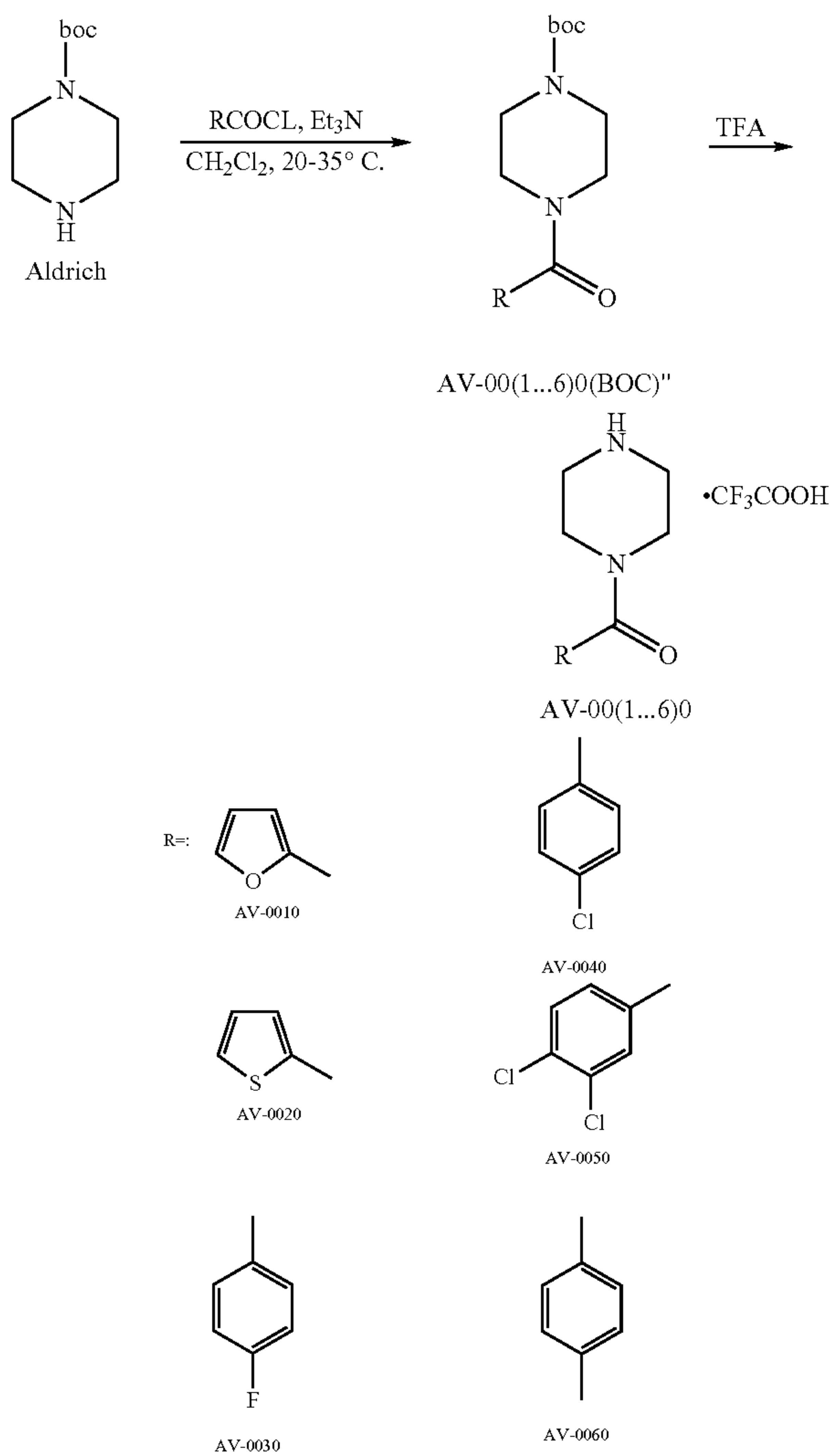
Reaction Scheme 23
