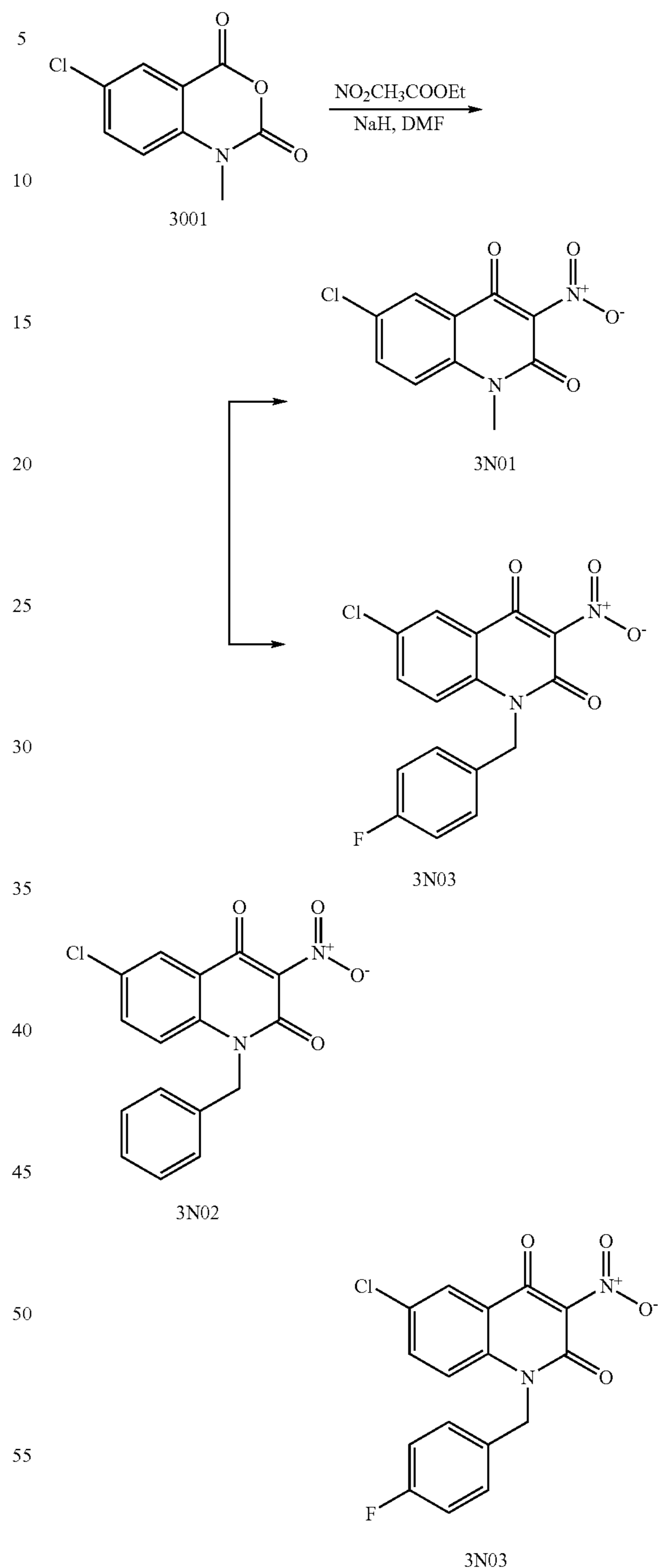
Reaction Scheme 26
