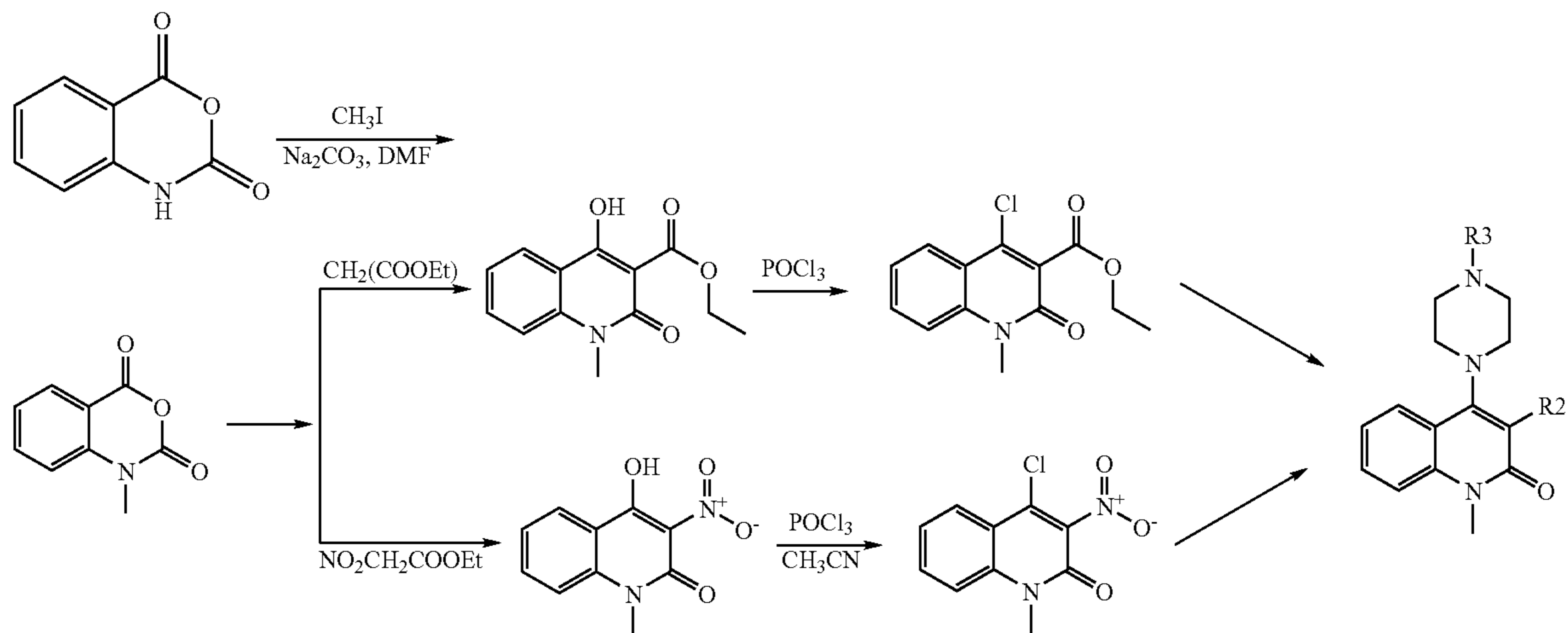
Reaction Scheme 9
