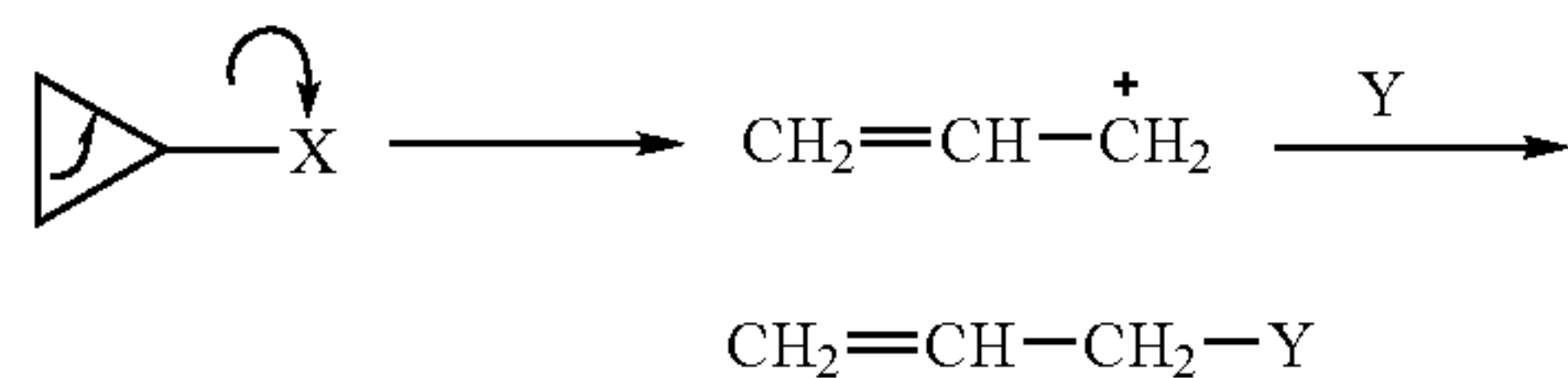
Reaction Scheme 7
