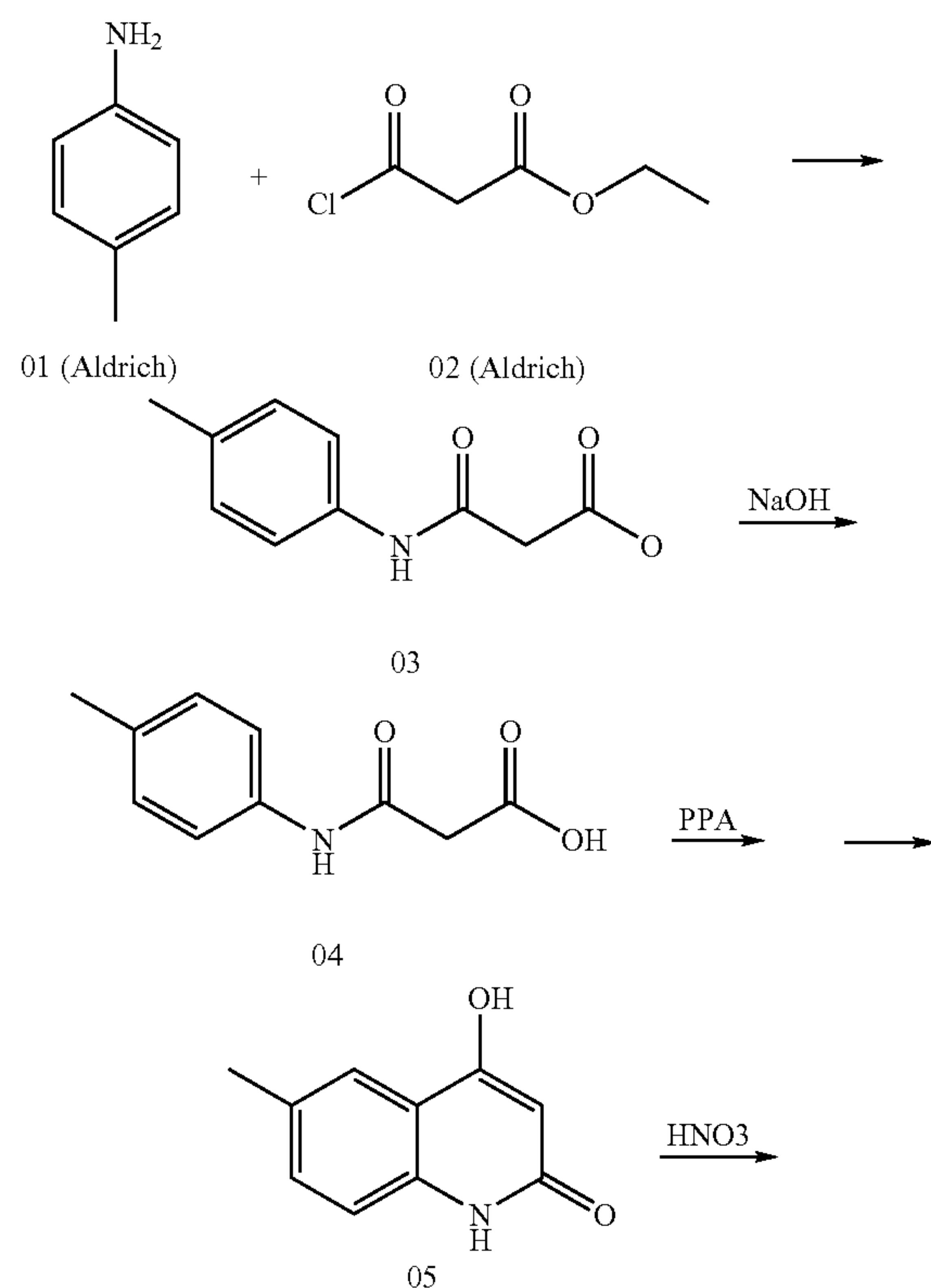
Reaction Scheme 25
