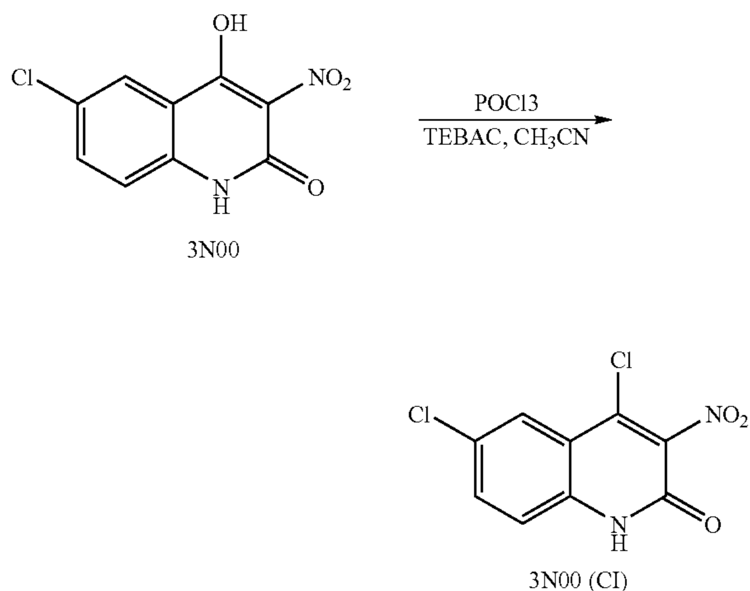
Reaction Scheme 27
