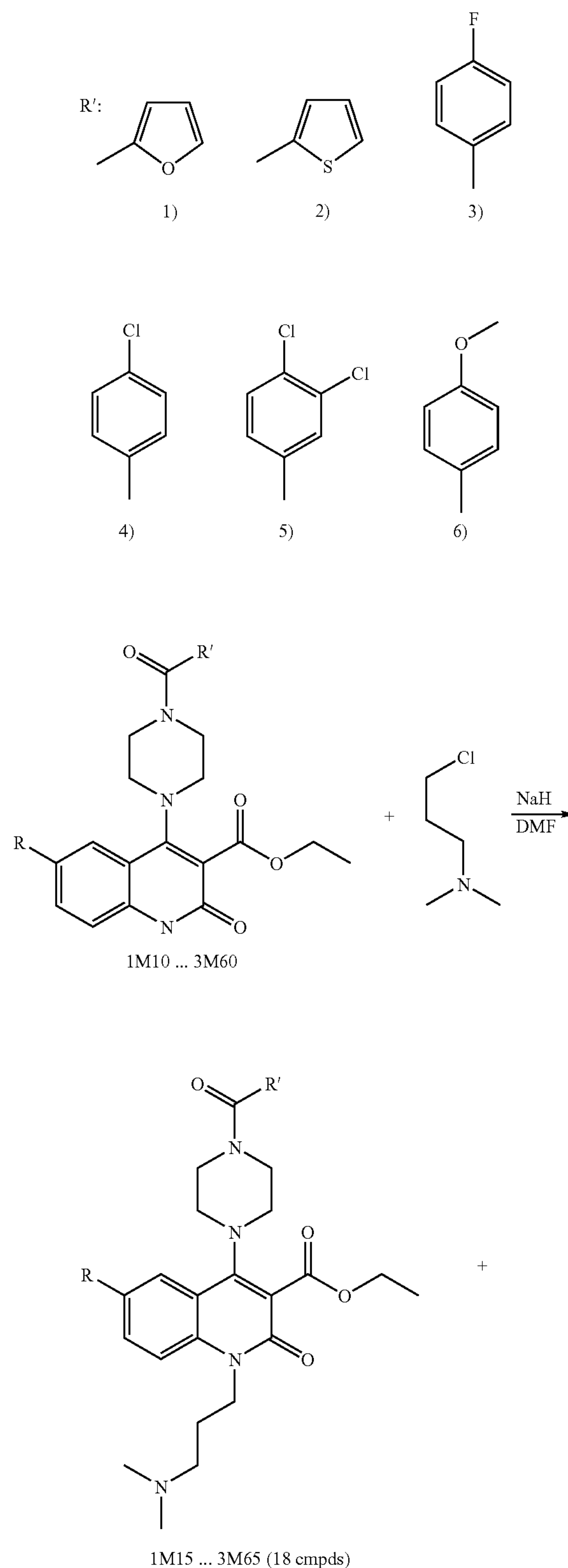
Reaction Scheme 24
