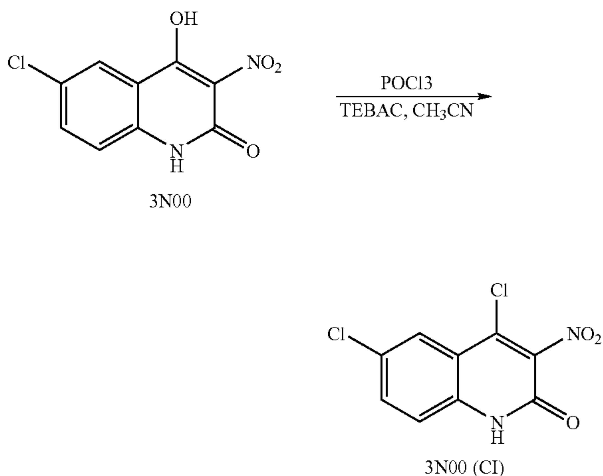
Reaction Scheme 27
