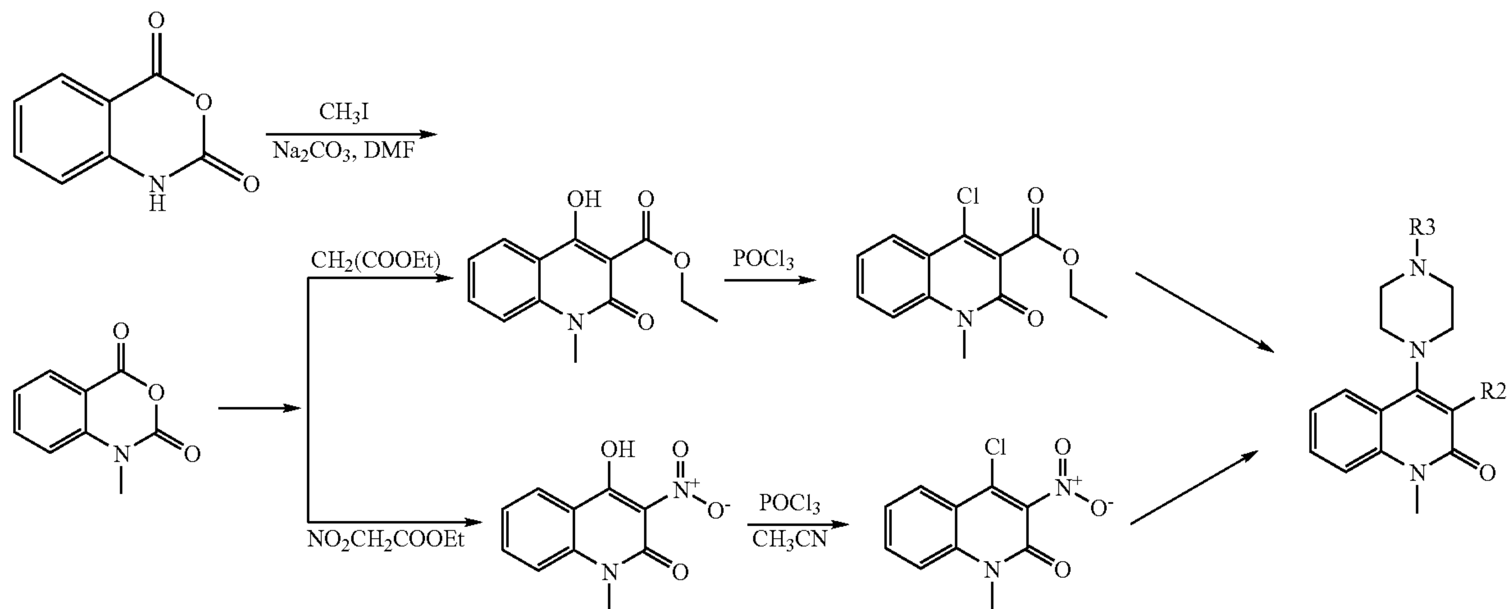
Reaction Scheme 9
