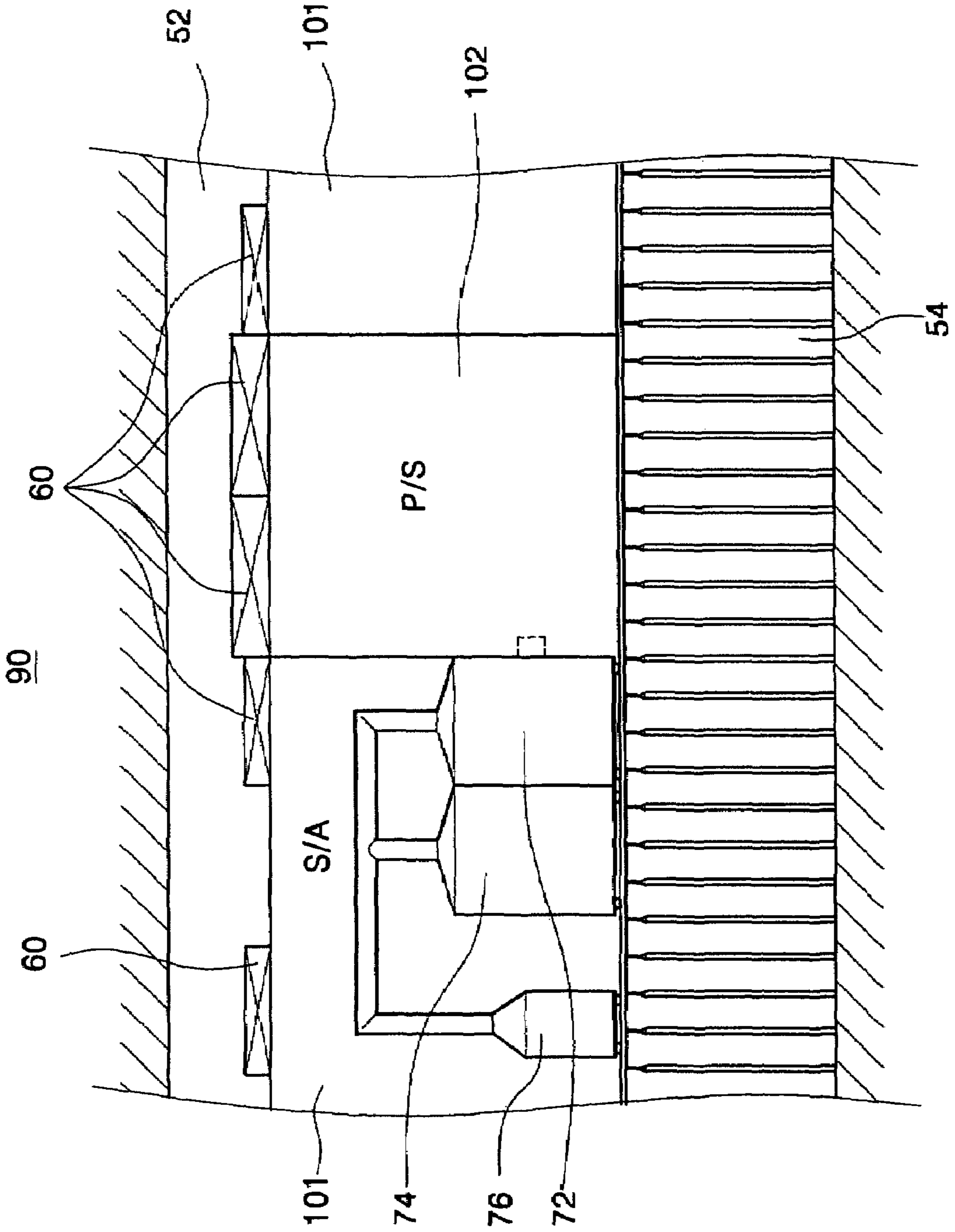
FIG. 2 (PRIOR ART)
