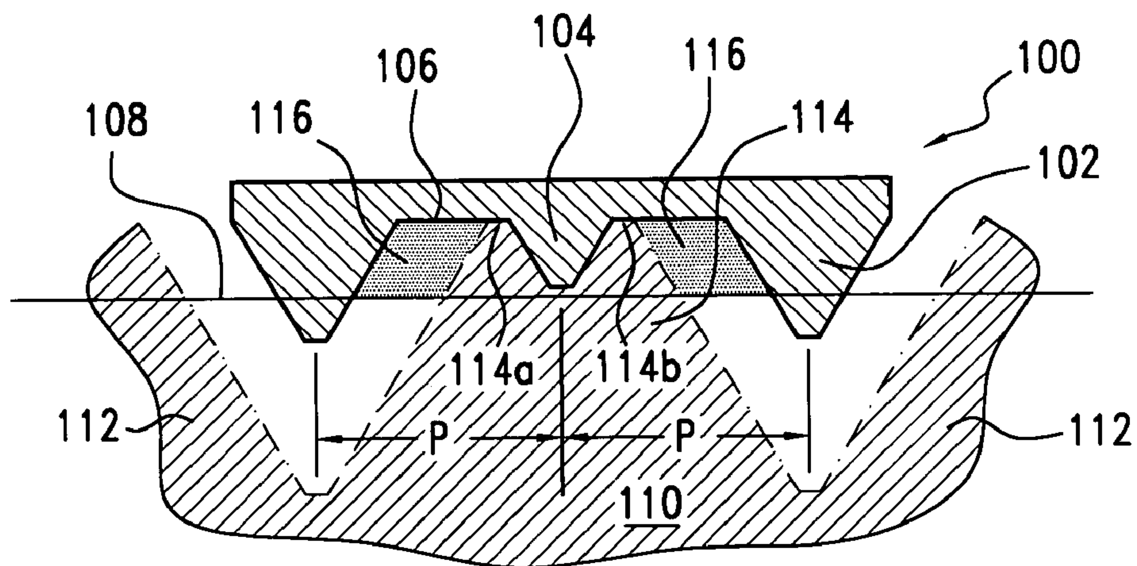
FIG. 18 (PRIOR ART)
