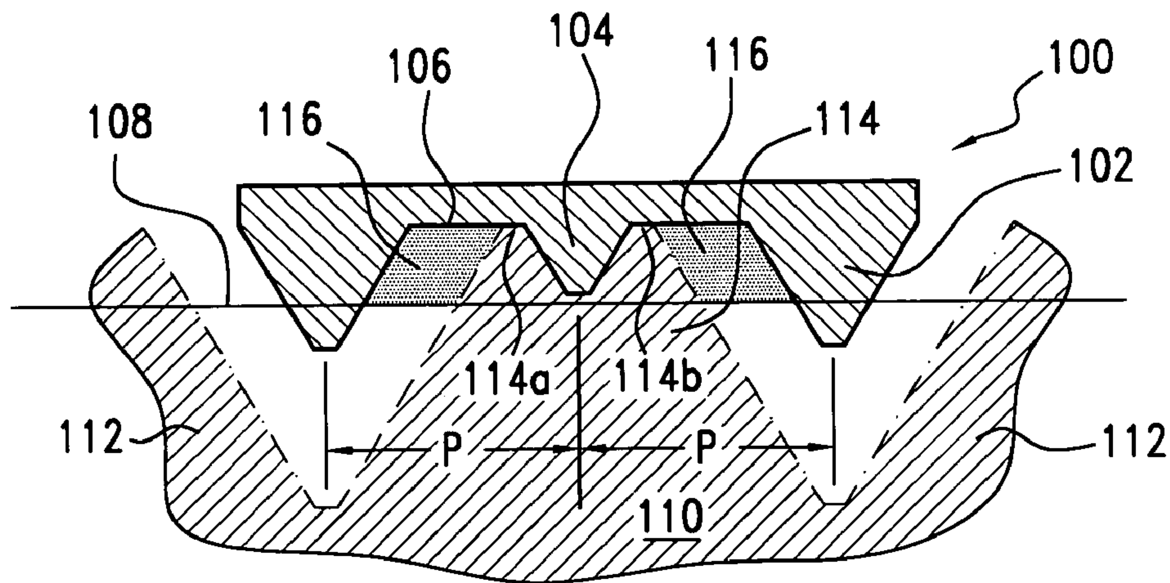
FIG. 18 (PRIOR ART)
