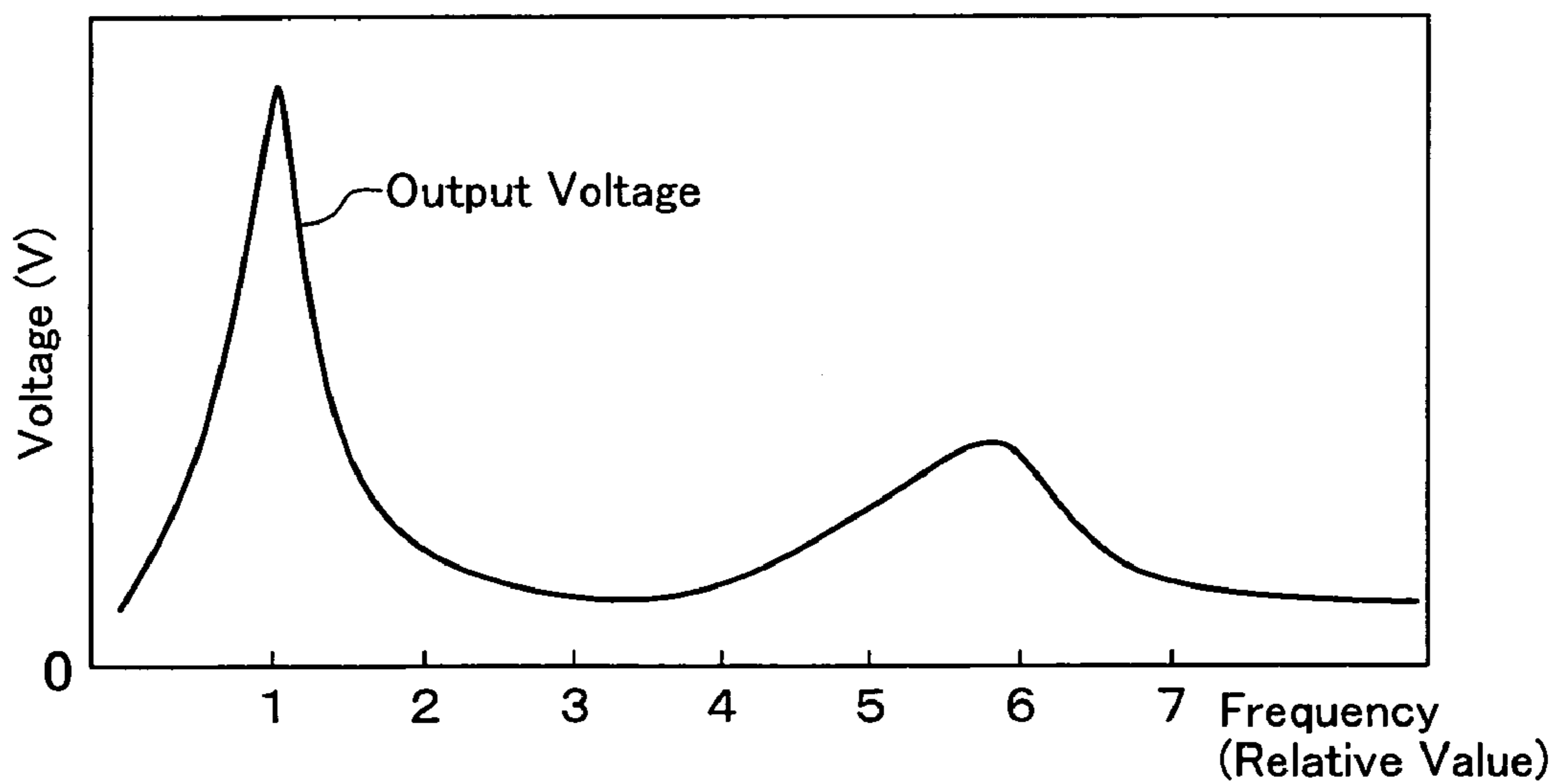
Output Voltage of Sensor in Frequency Domain
