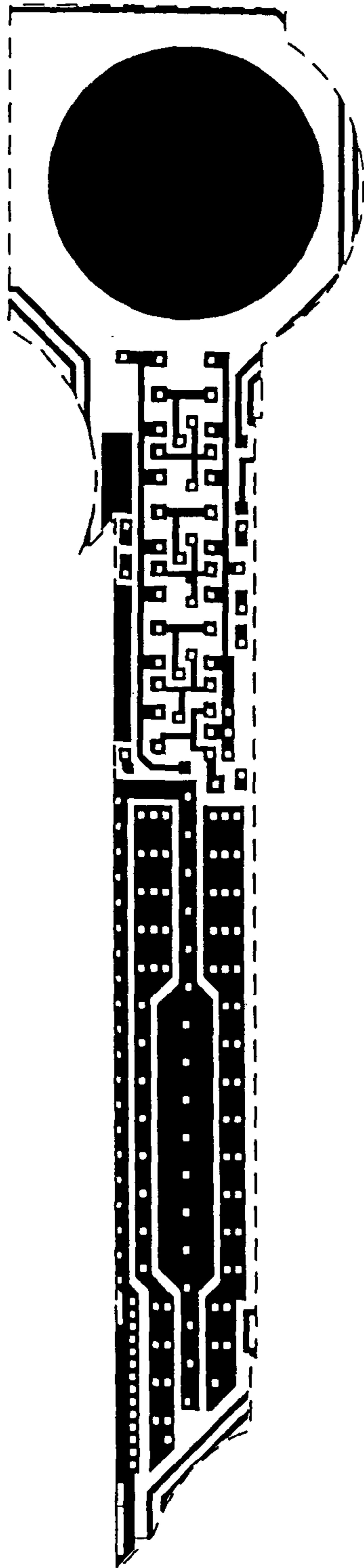
Metal 1 mask
