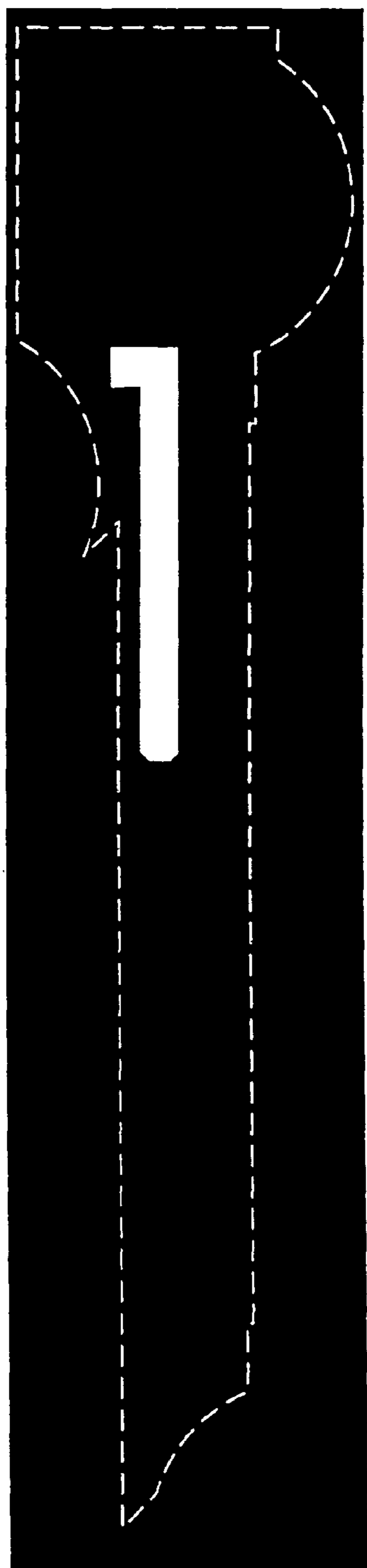
N-Well mask
