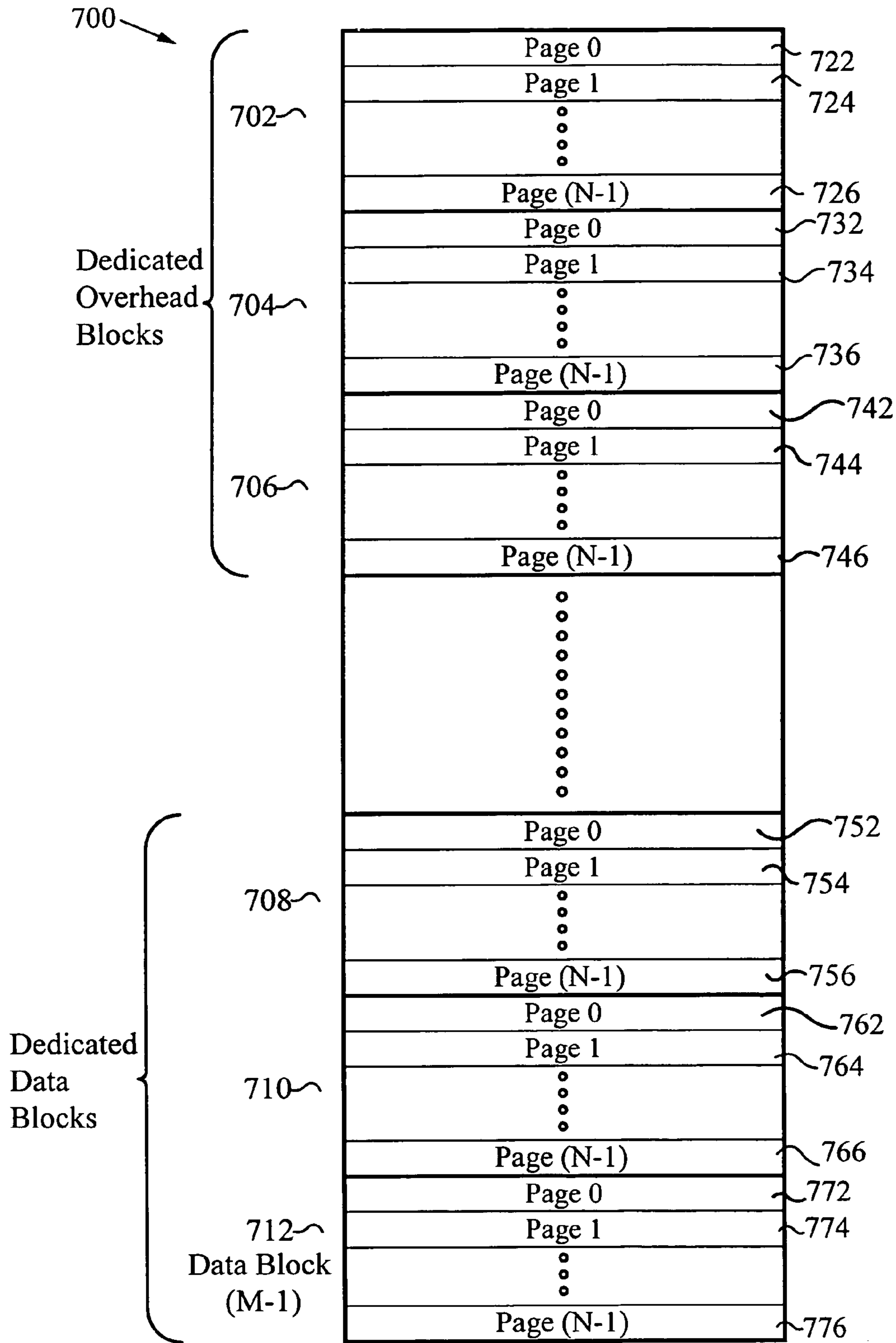
Flash Memory Array
