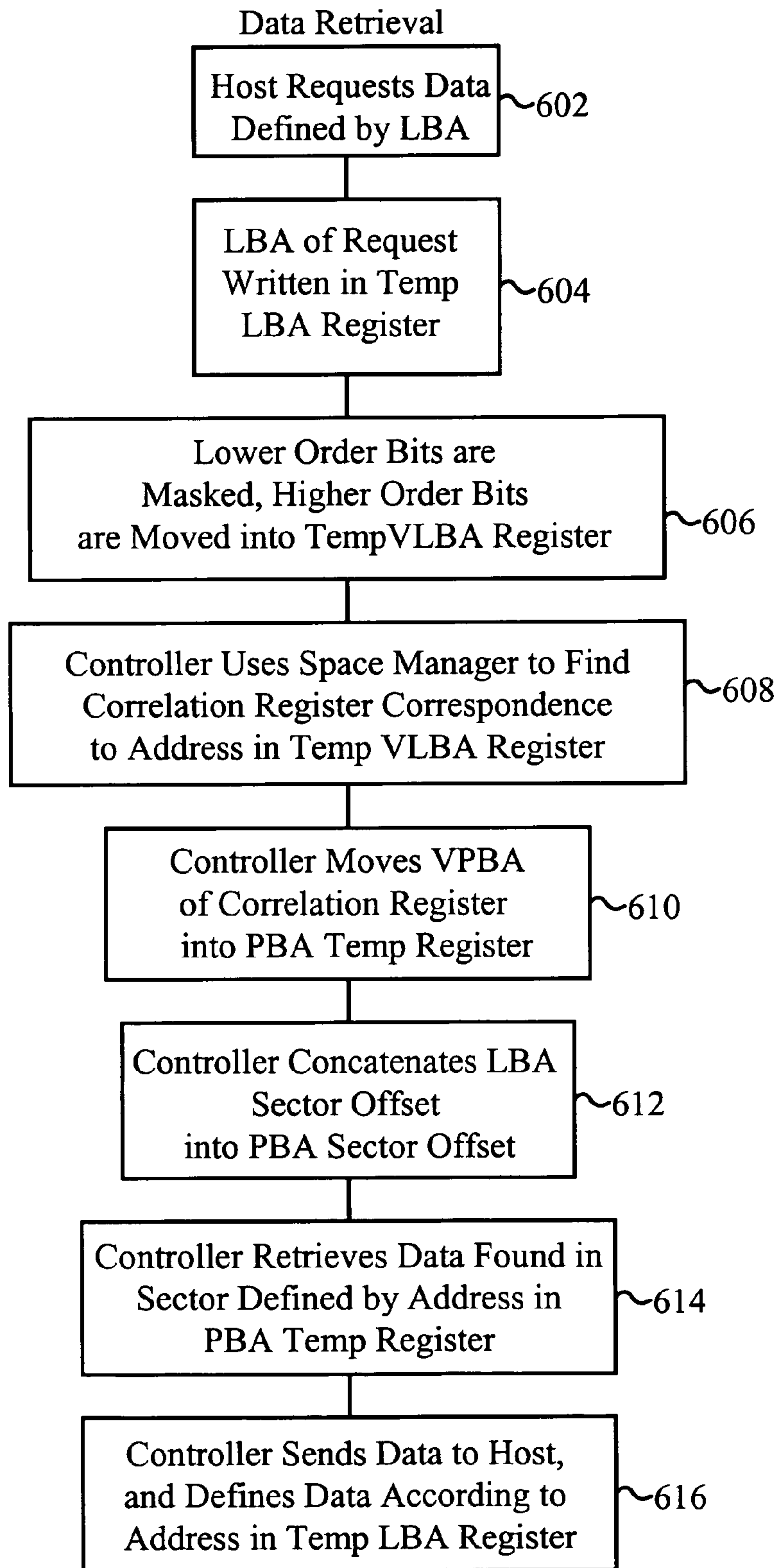
Fig. 6 (PRIOR ART)
