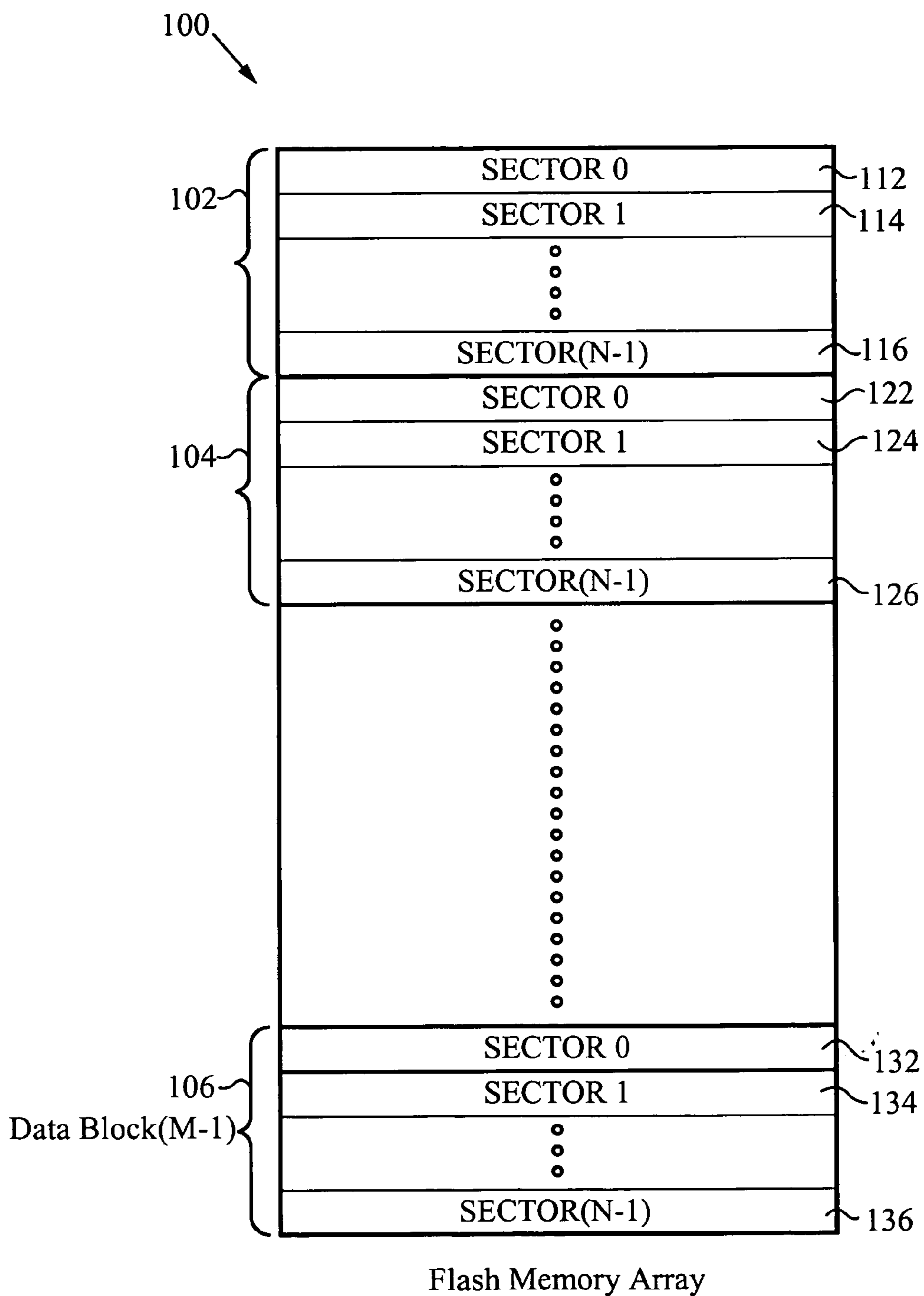
Flash Memory Array Fig. 1 (PRIOR ART)
