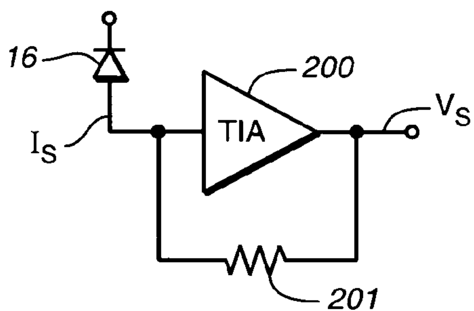
FIG. 48 (PRIOR ART)
