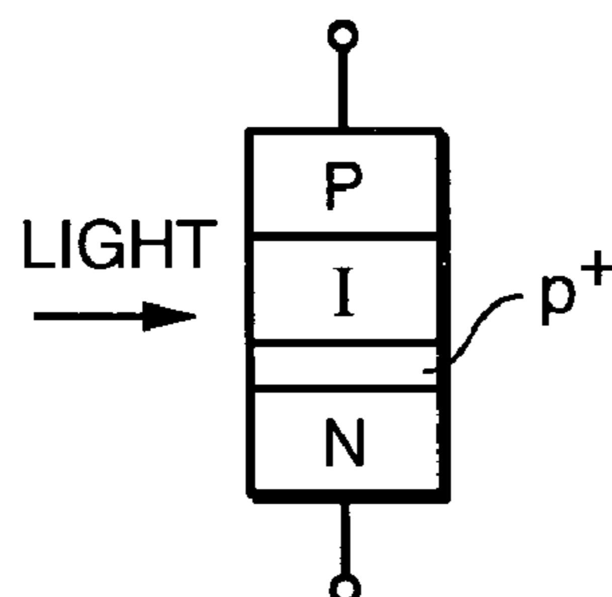
FIG. 26 (PRIOR ART)
