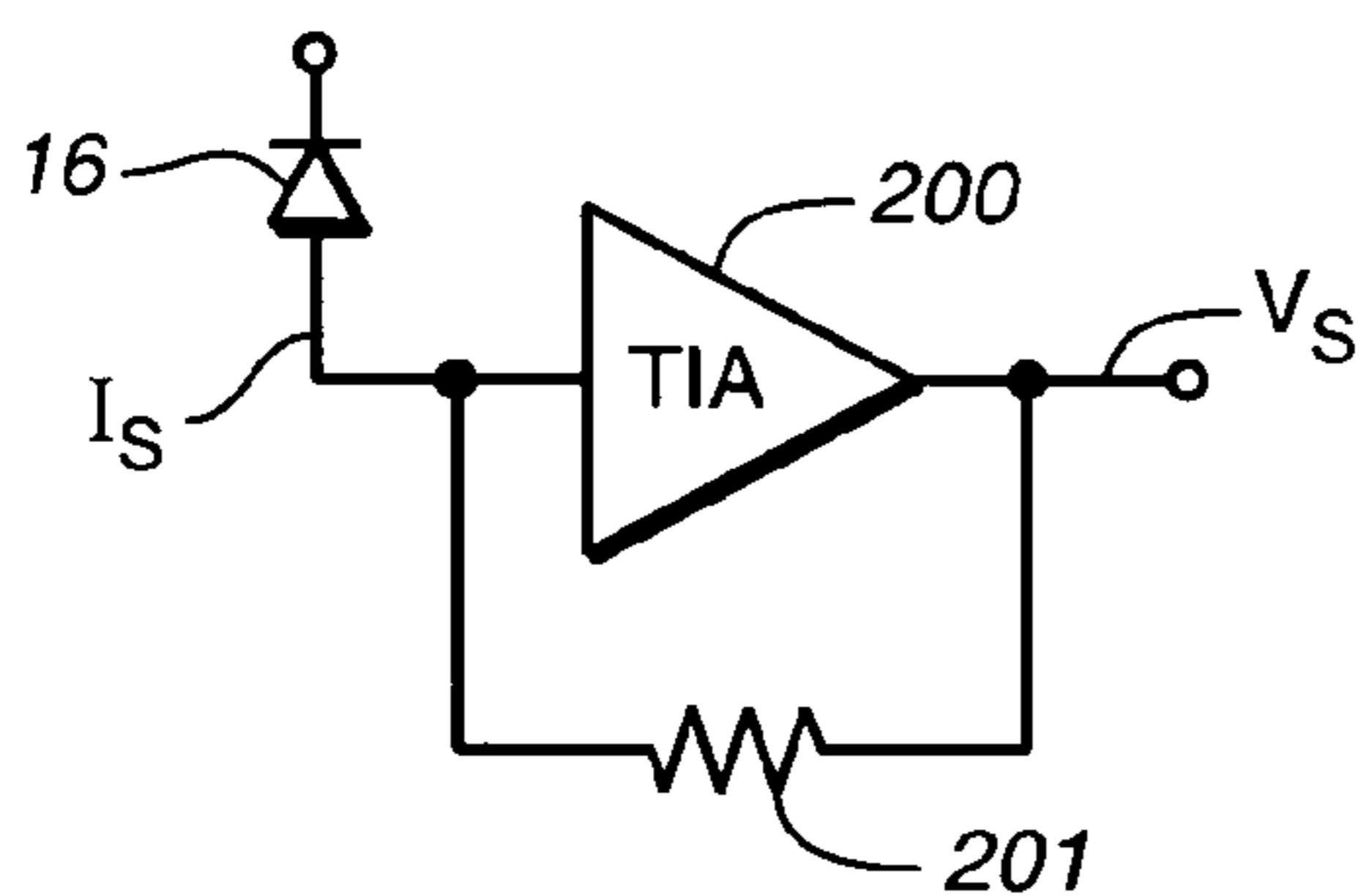
FIG. 48 (PRIOR ART)
