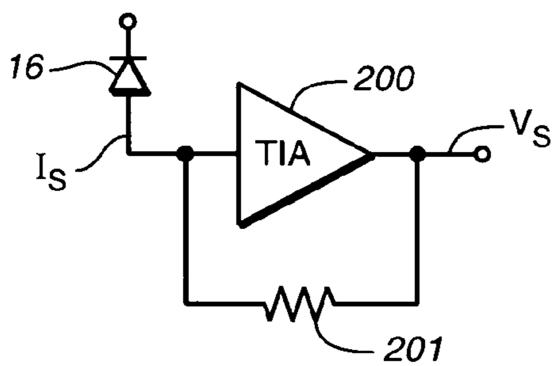
FIG. 48 (PRIOR ART)
