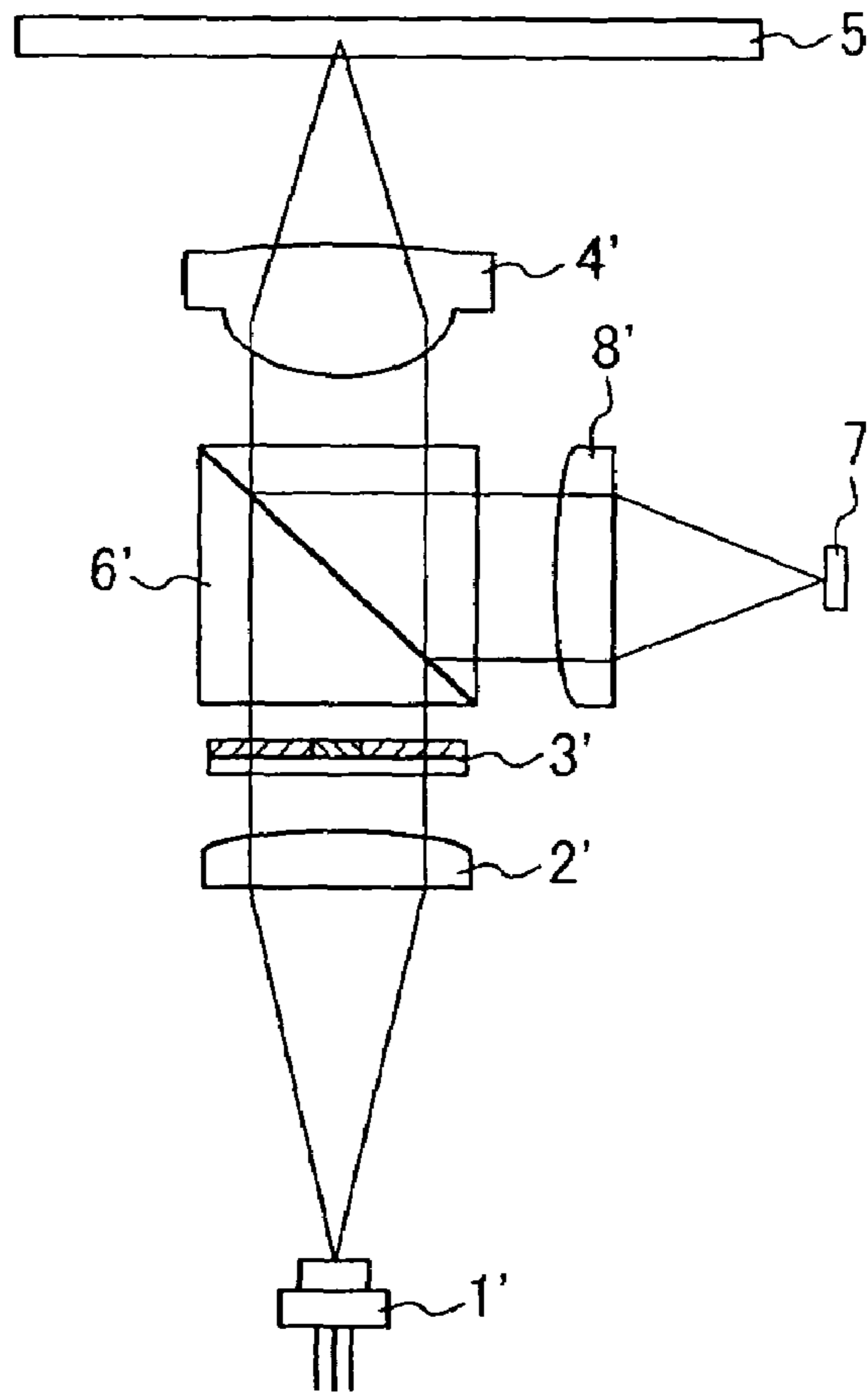
FIG. 13A (PRIOR ART)
