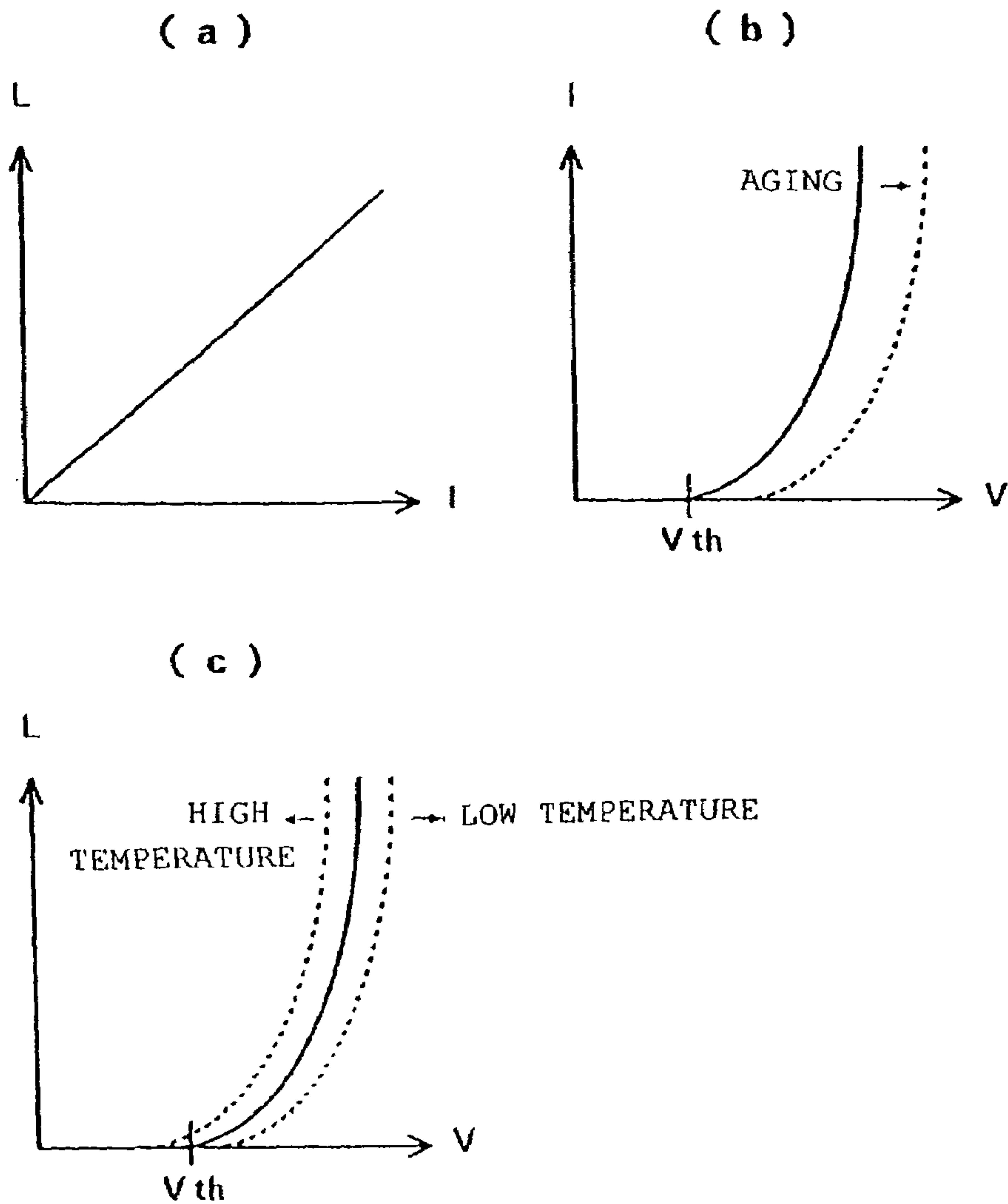
FIG. 2 (Prior Art)
