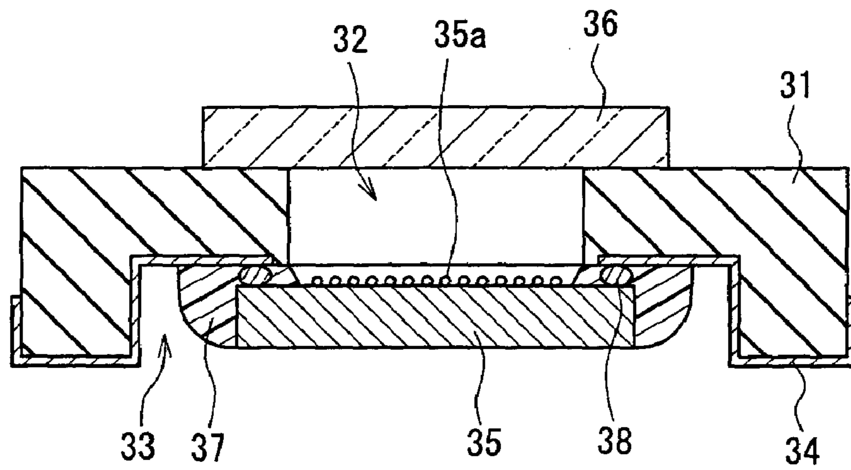
FIG. 7 PRIOR ART
