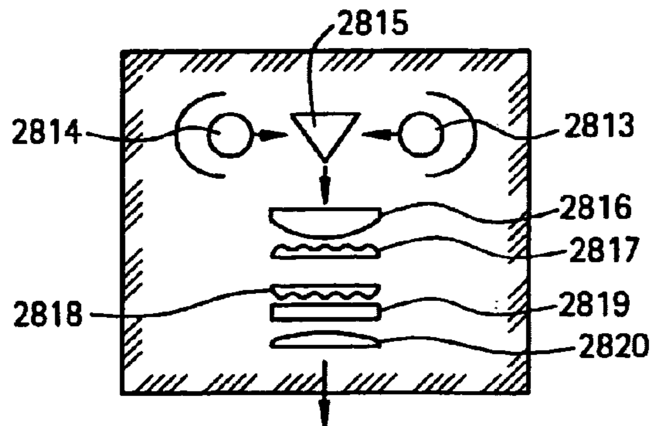
LIGHT SOURCE OPTICAL SYSTEM
