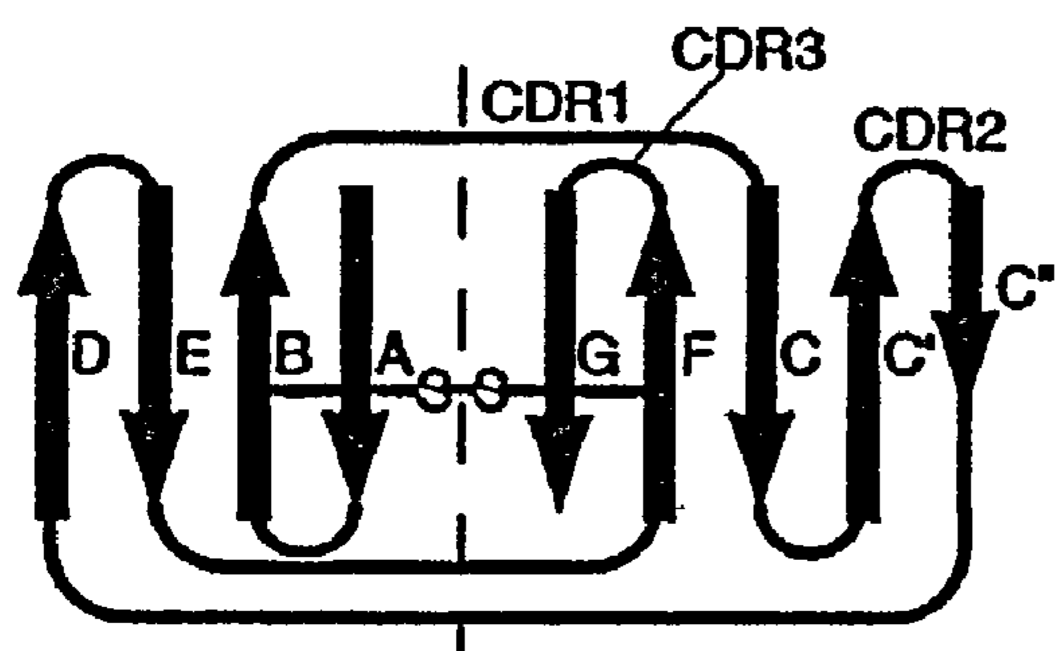
Immunoglobulin VH
