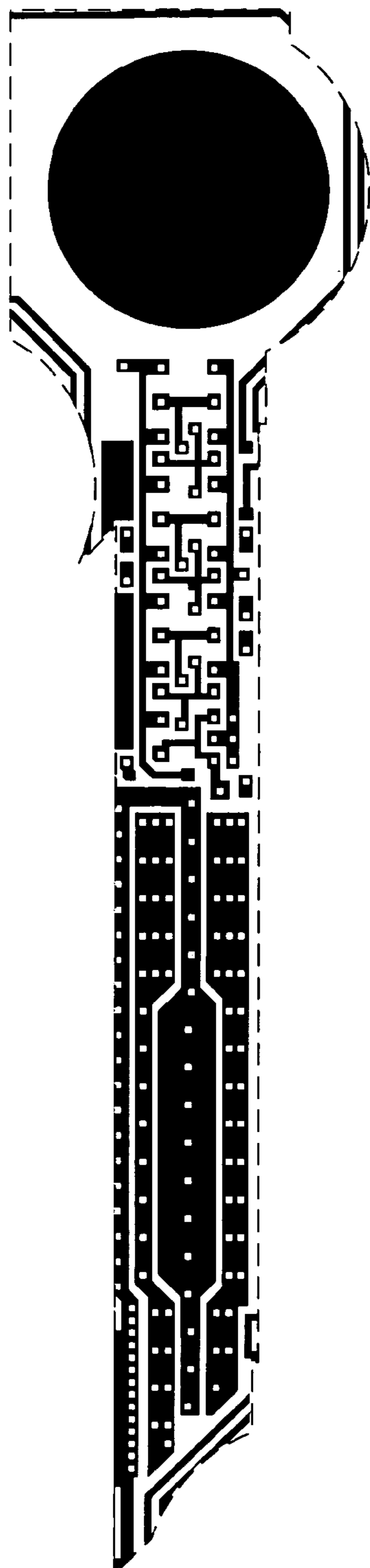
Metal 1 mask
