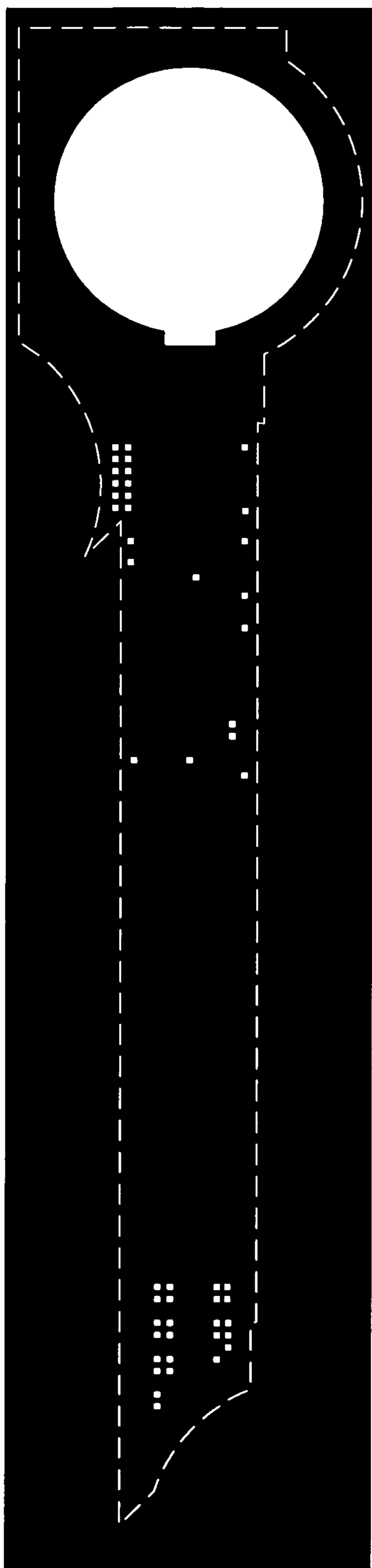
Via 1 mask
