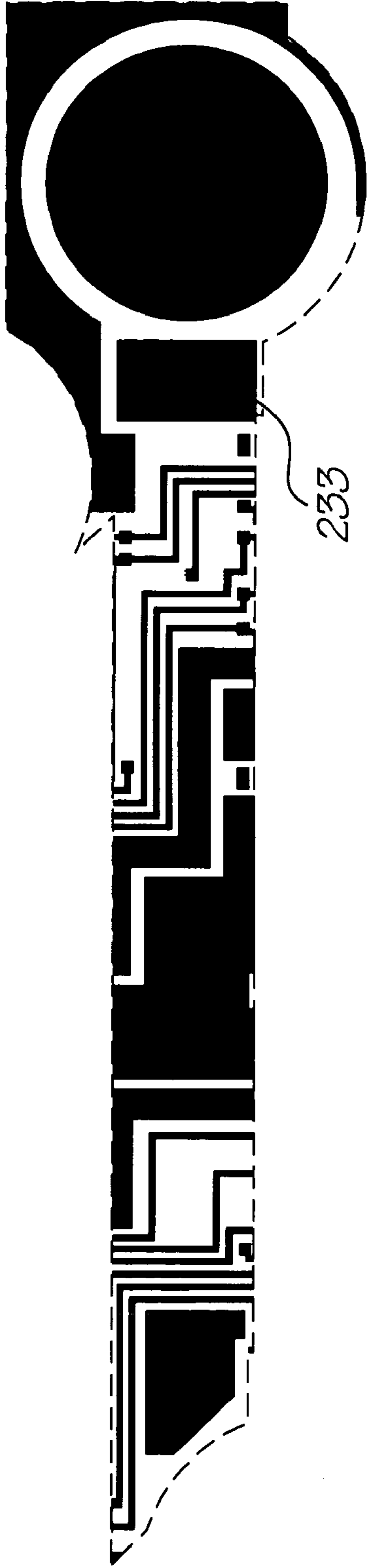
Metal 2 mask
