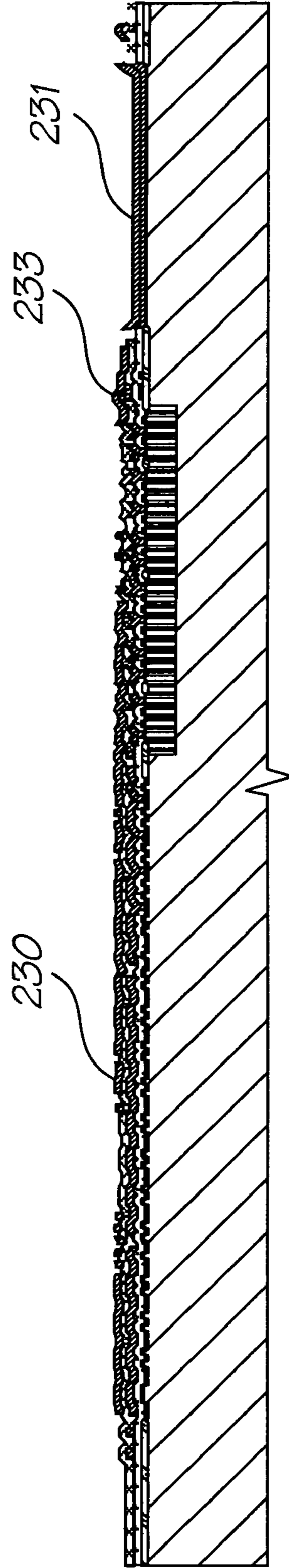
Deposit metal 2
