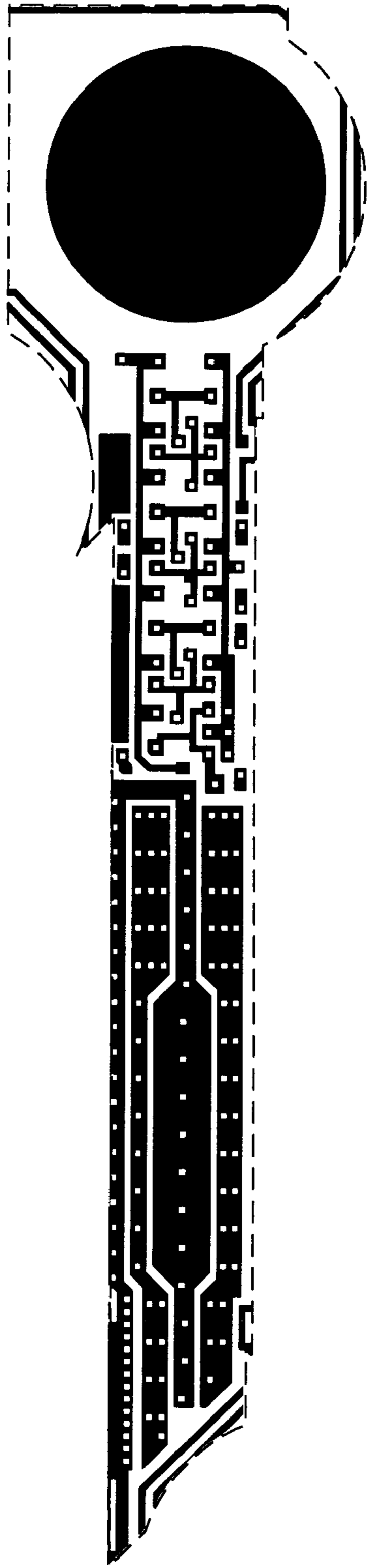
Metal 1 mask
