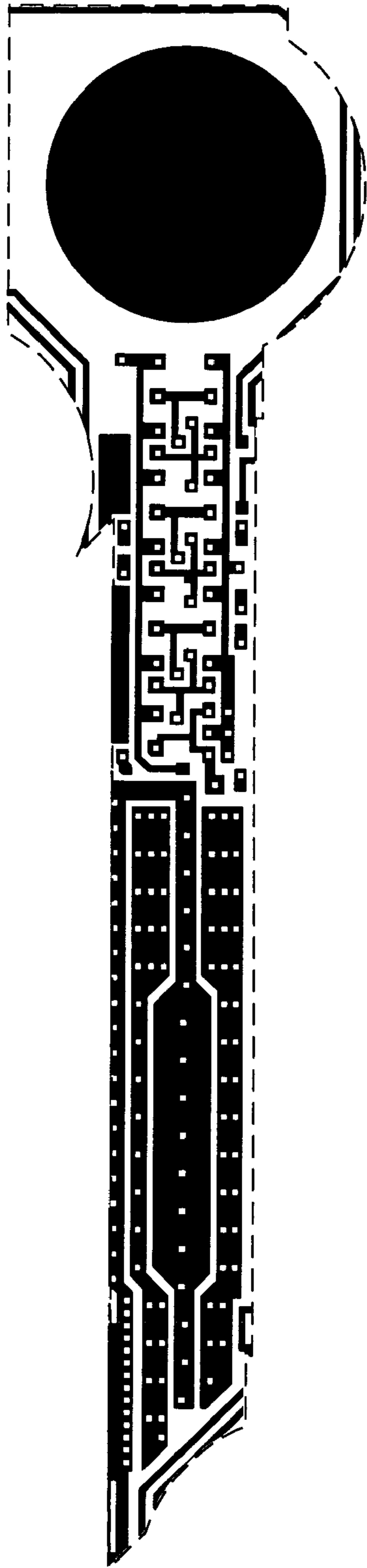
Metal 1 mask
