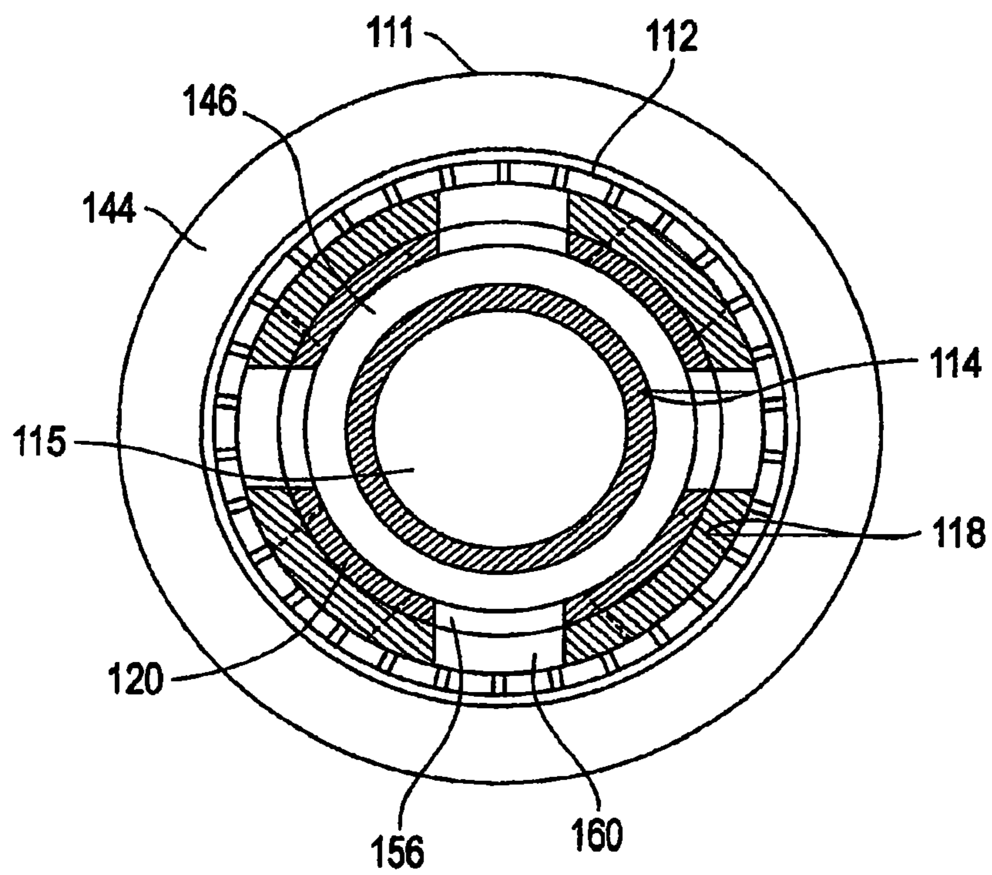
SECTION 'A-A'
