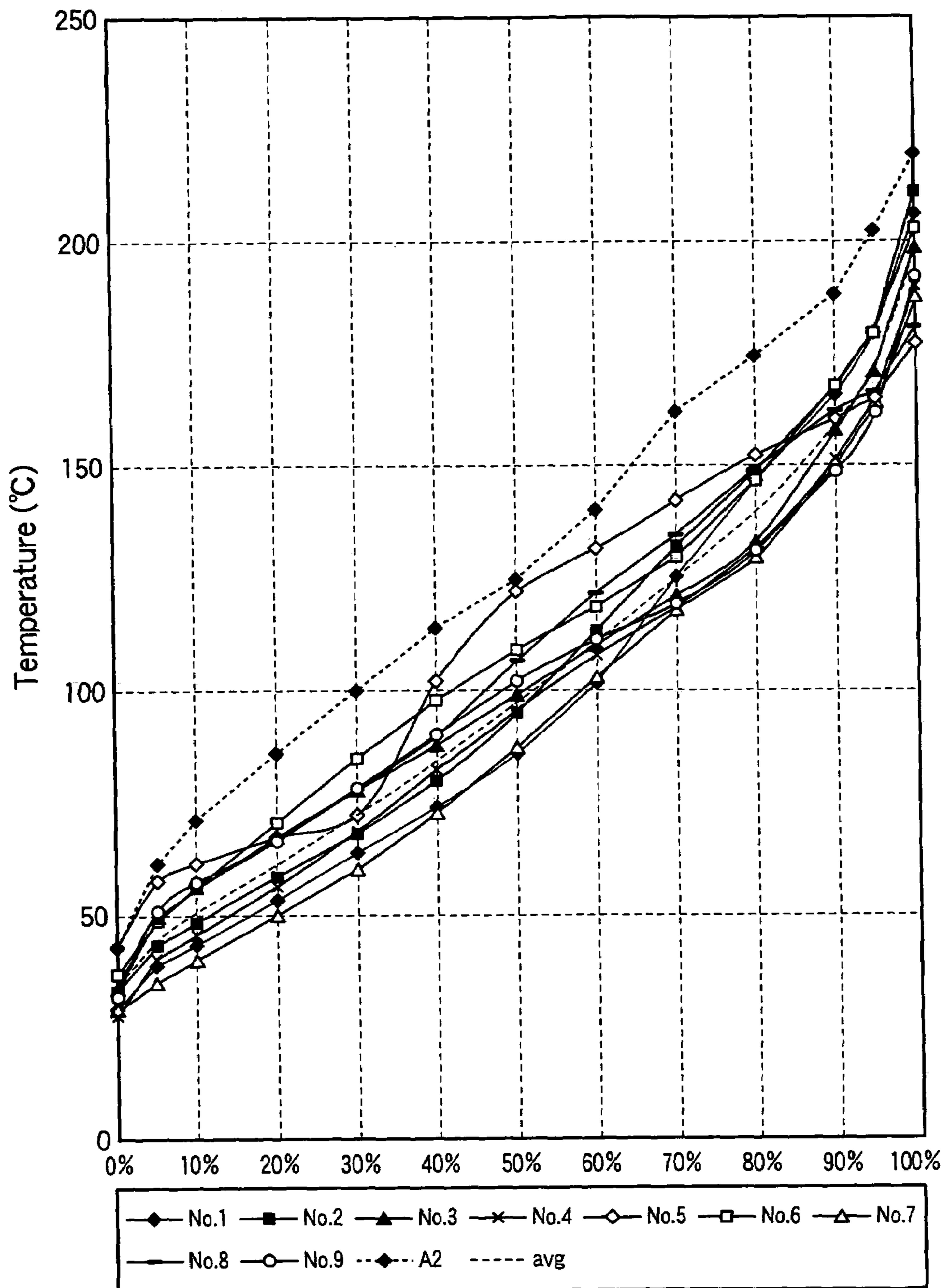
Distillation characteristics
