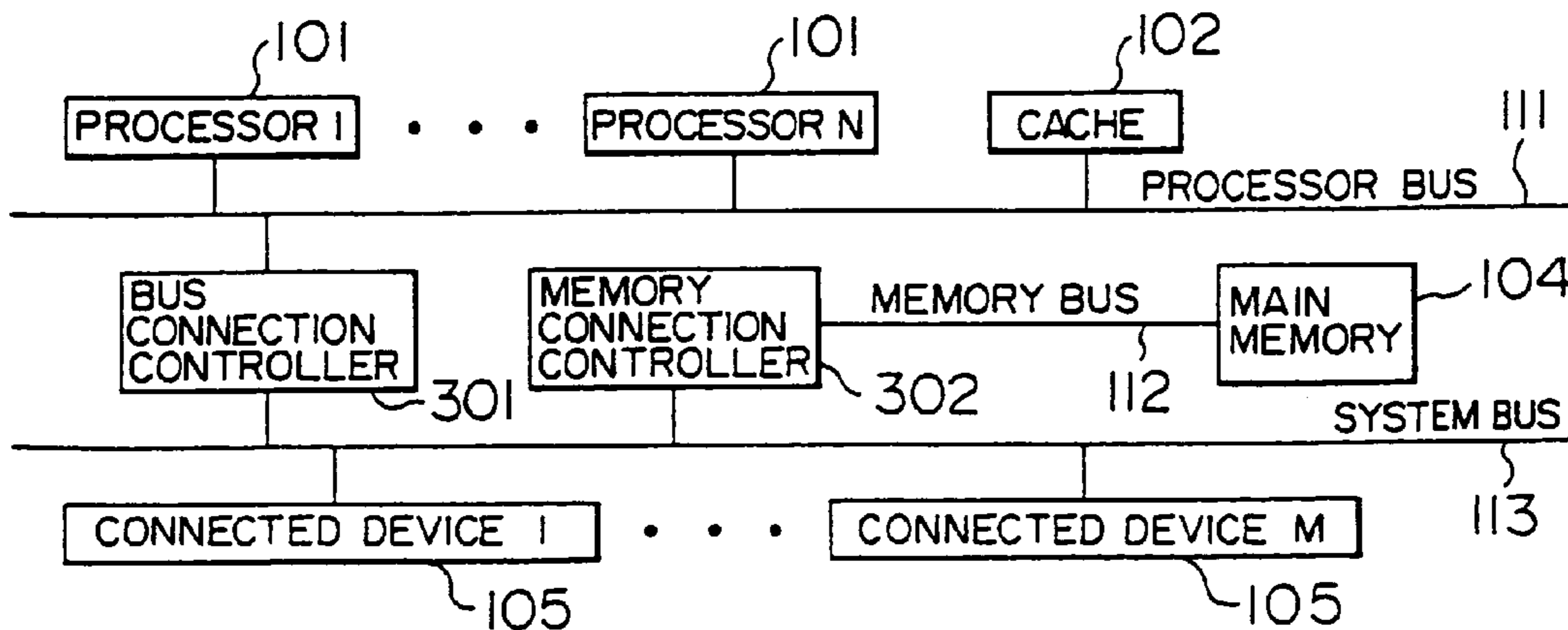
FIG. 3 PRIOR ART
