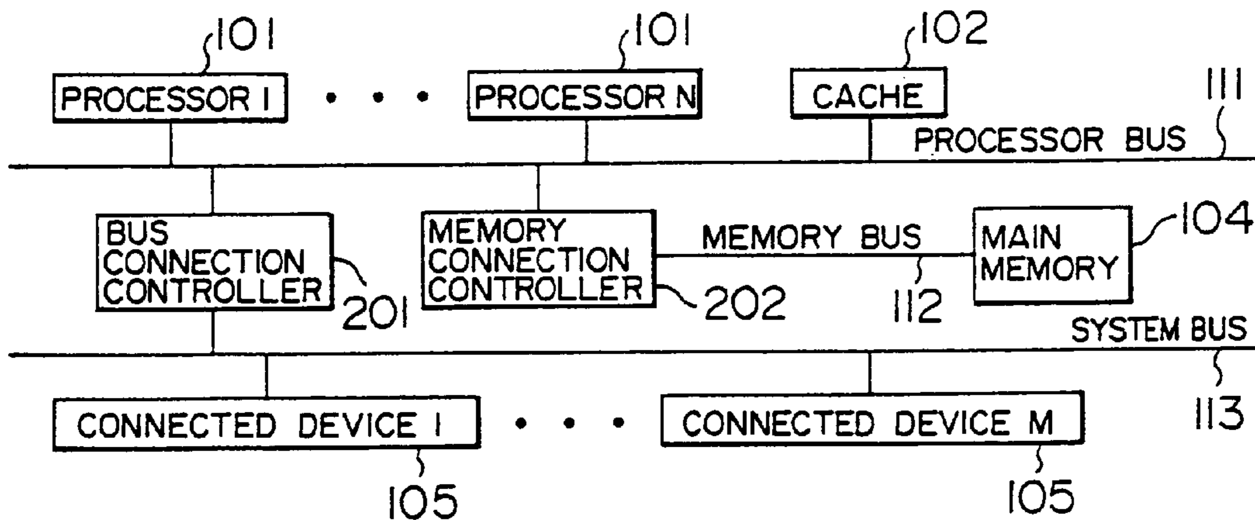
FIG. 3 PRIOR ART
