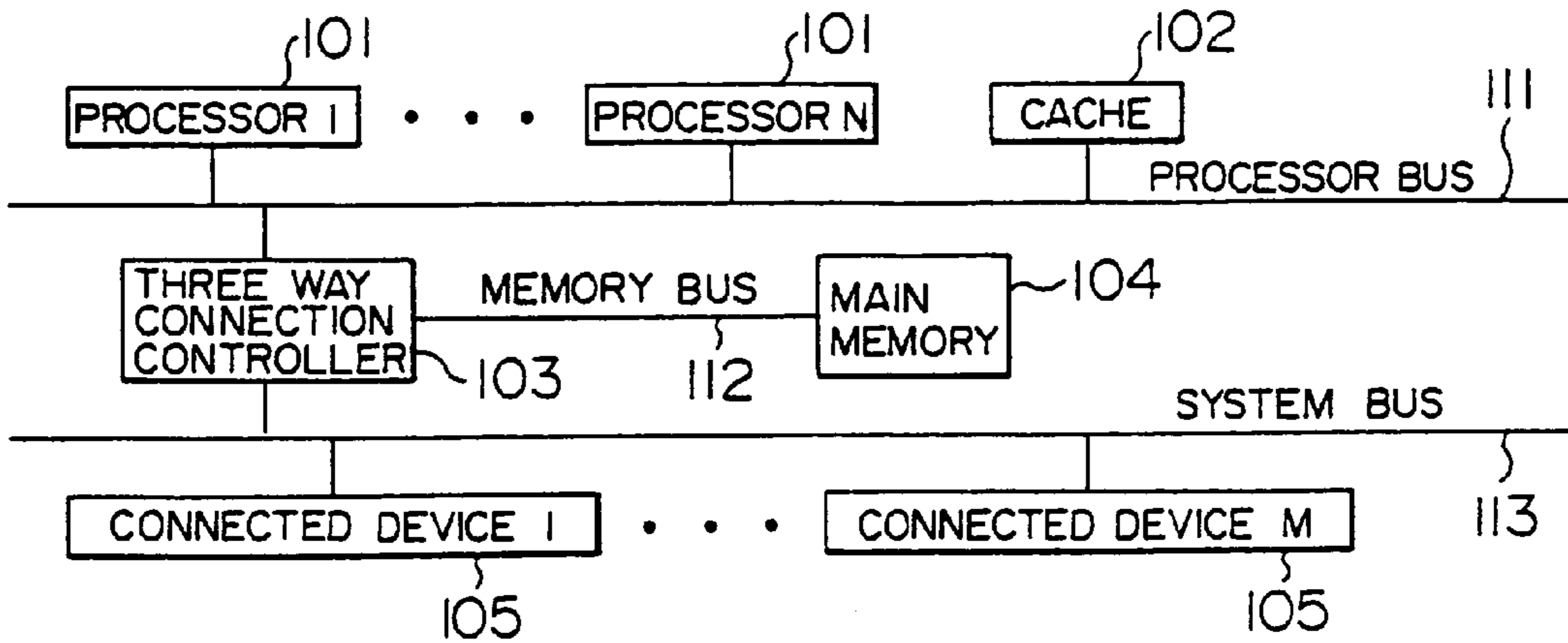
FIG. 2 PRIOR ART
