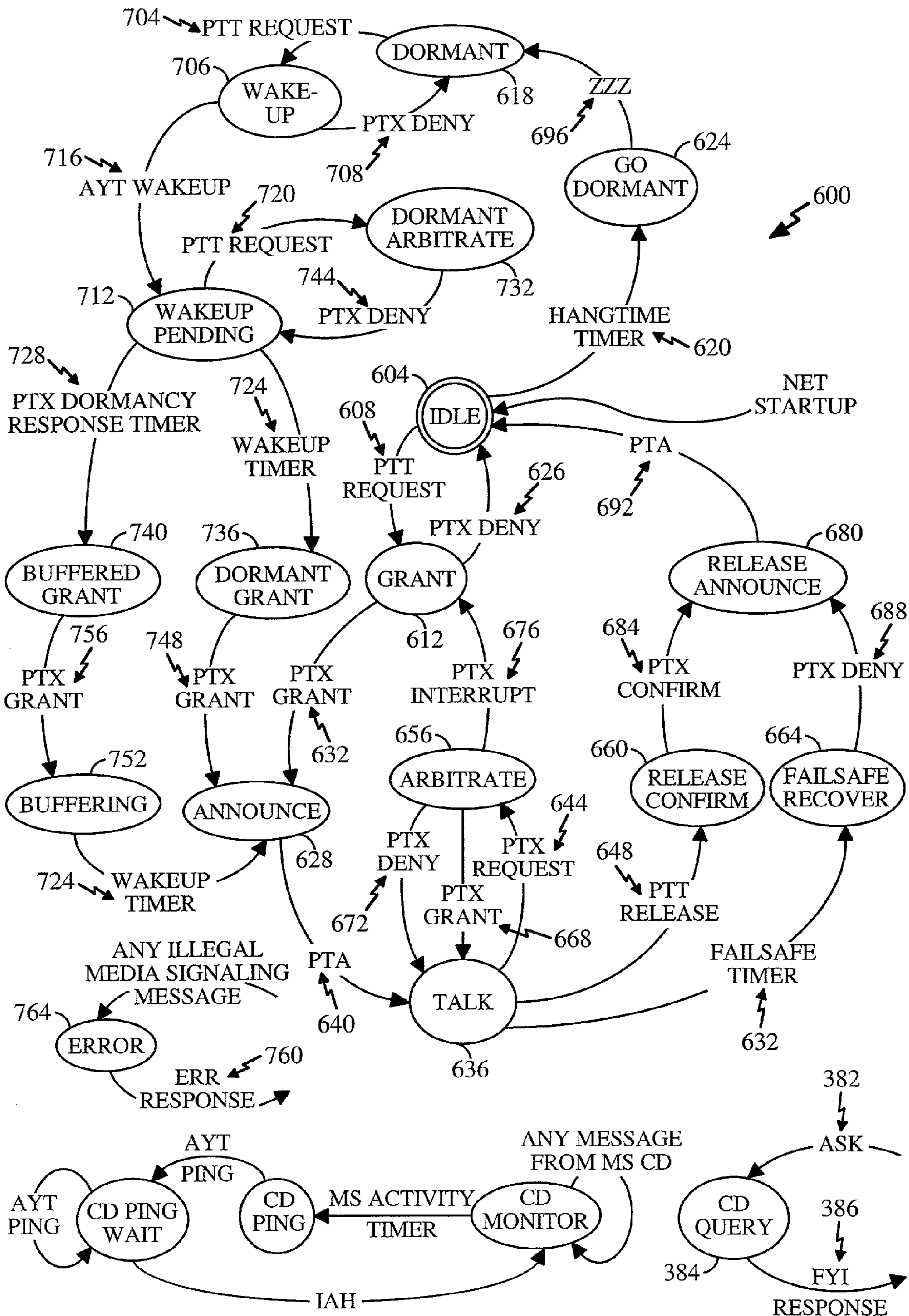
FIG. 15 MEDIA SIGNALING STATE DIAGRAM
