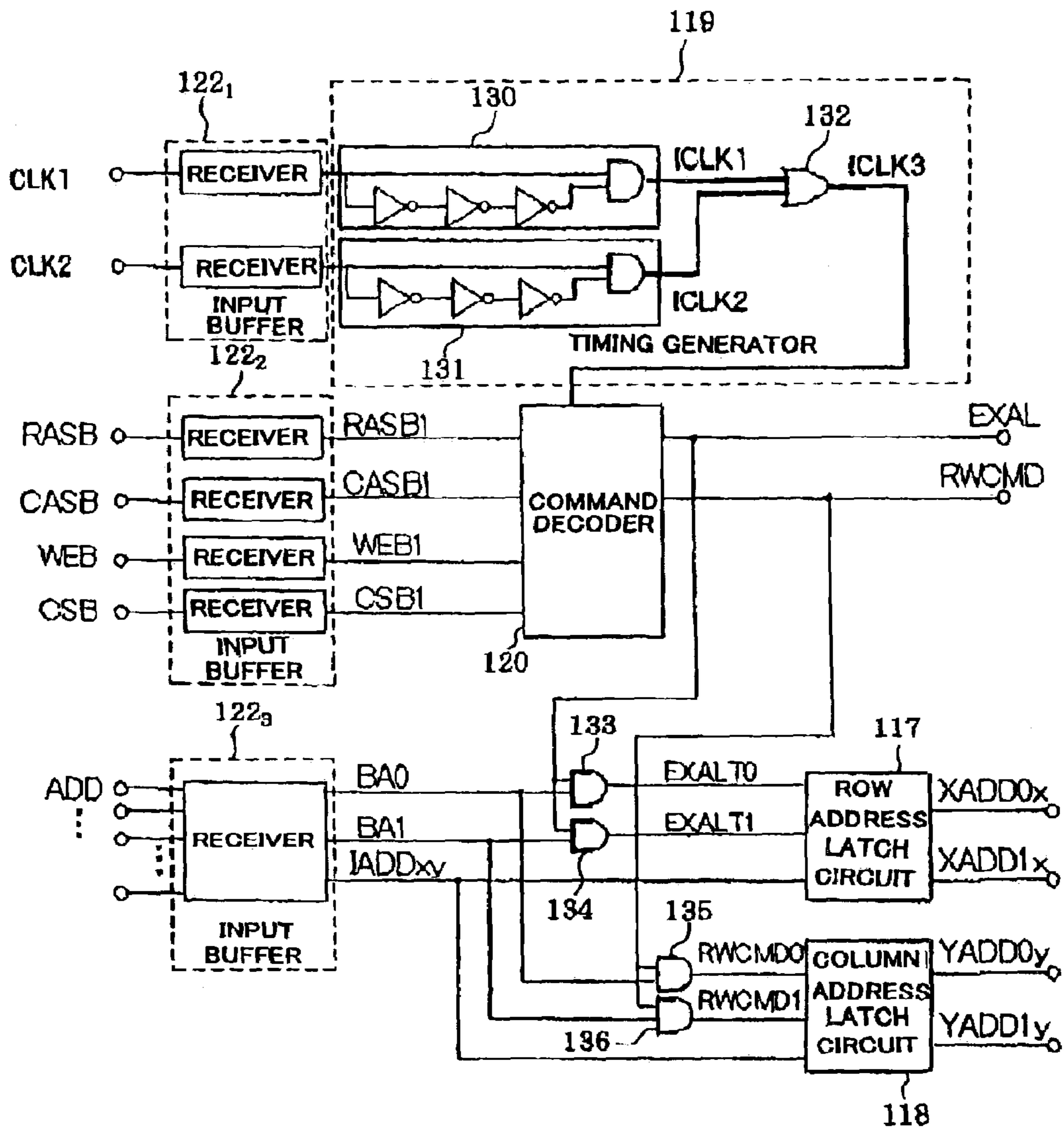
FIG. 2 (PRIOR ART)
