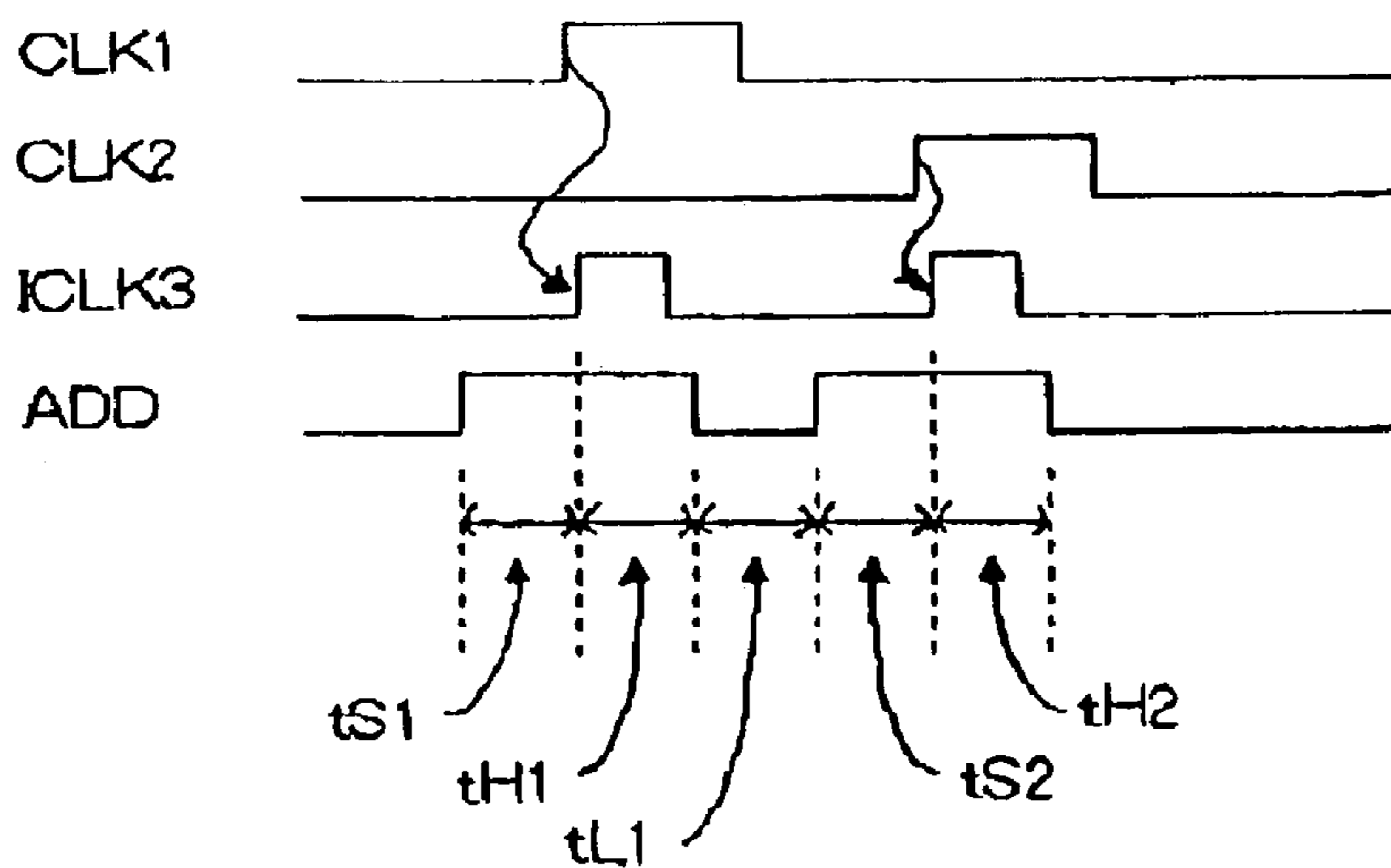
FIG. 4 (PRIOR ART)
