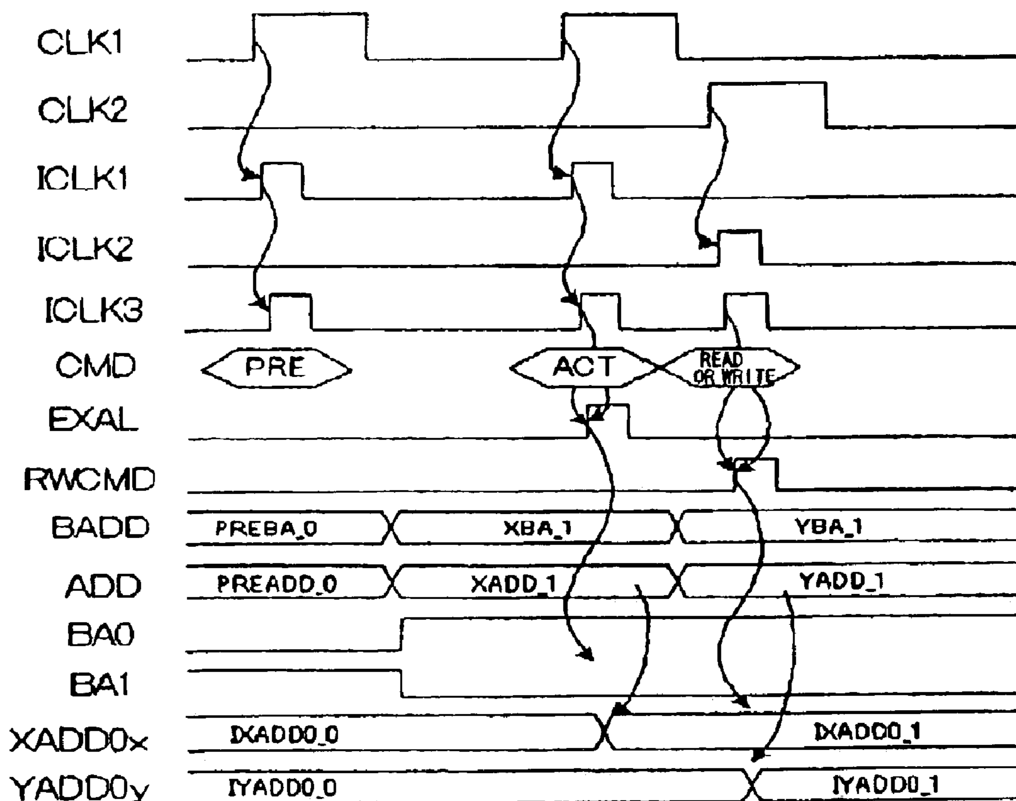
FIG. 3 (PRIOR ART)
