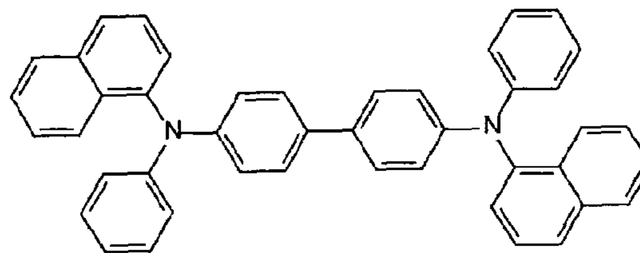
α-NPD
