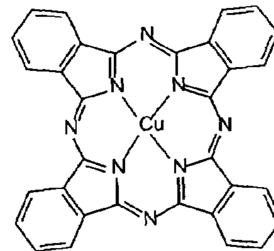
CuPc
