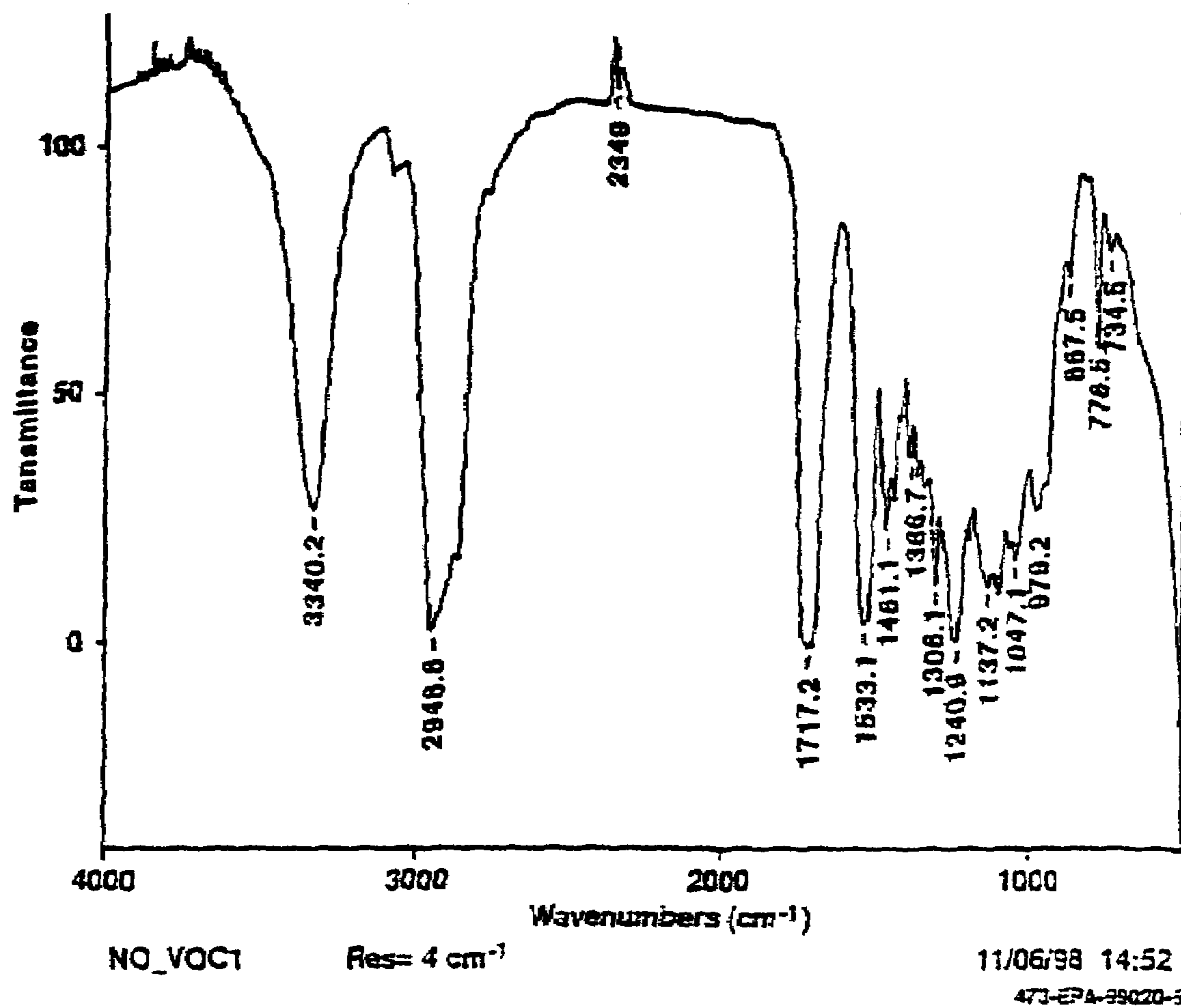
IR spectra of PCLVD synthesis
