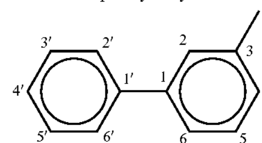
biphenyl-4-yl-
