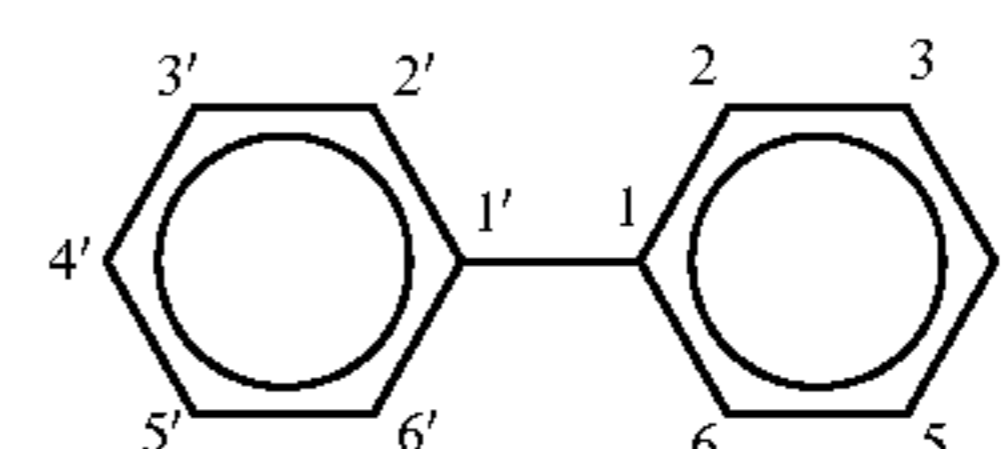
biphenyl-4-yl-
