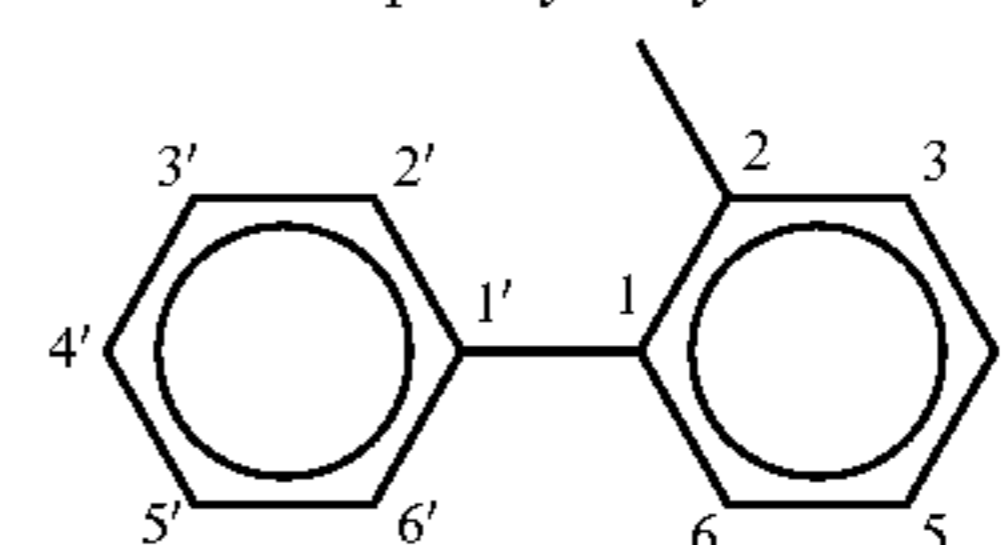
biphenyl-3-yl-
