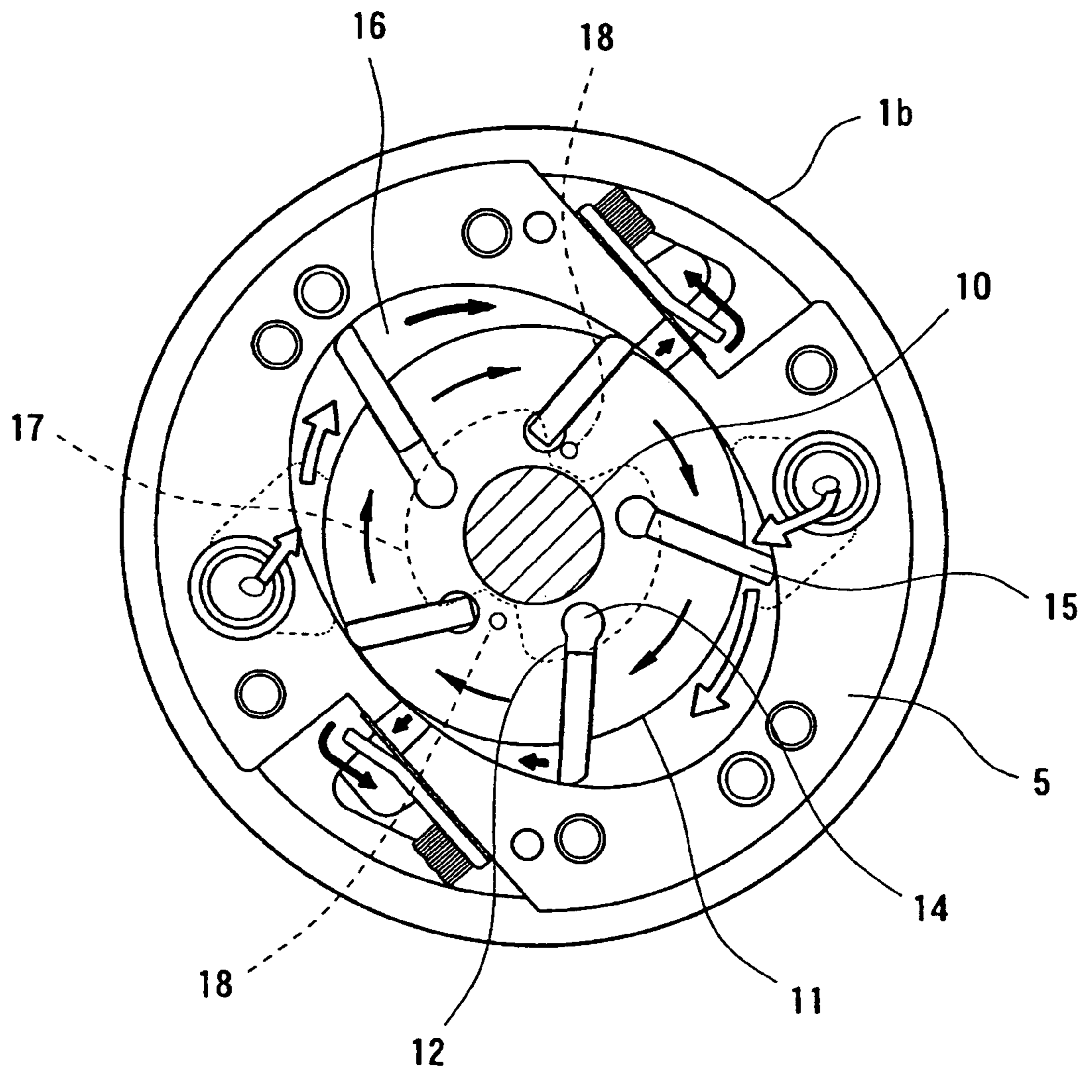
FIG. 11 PRIOR ART
