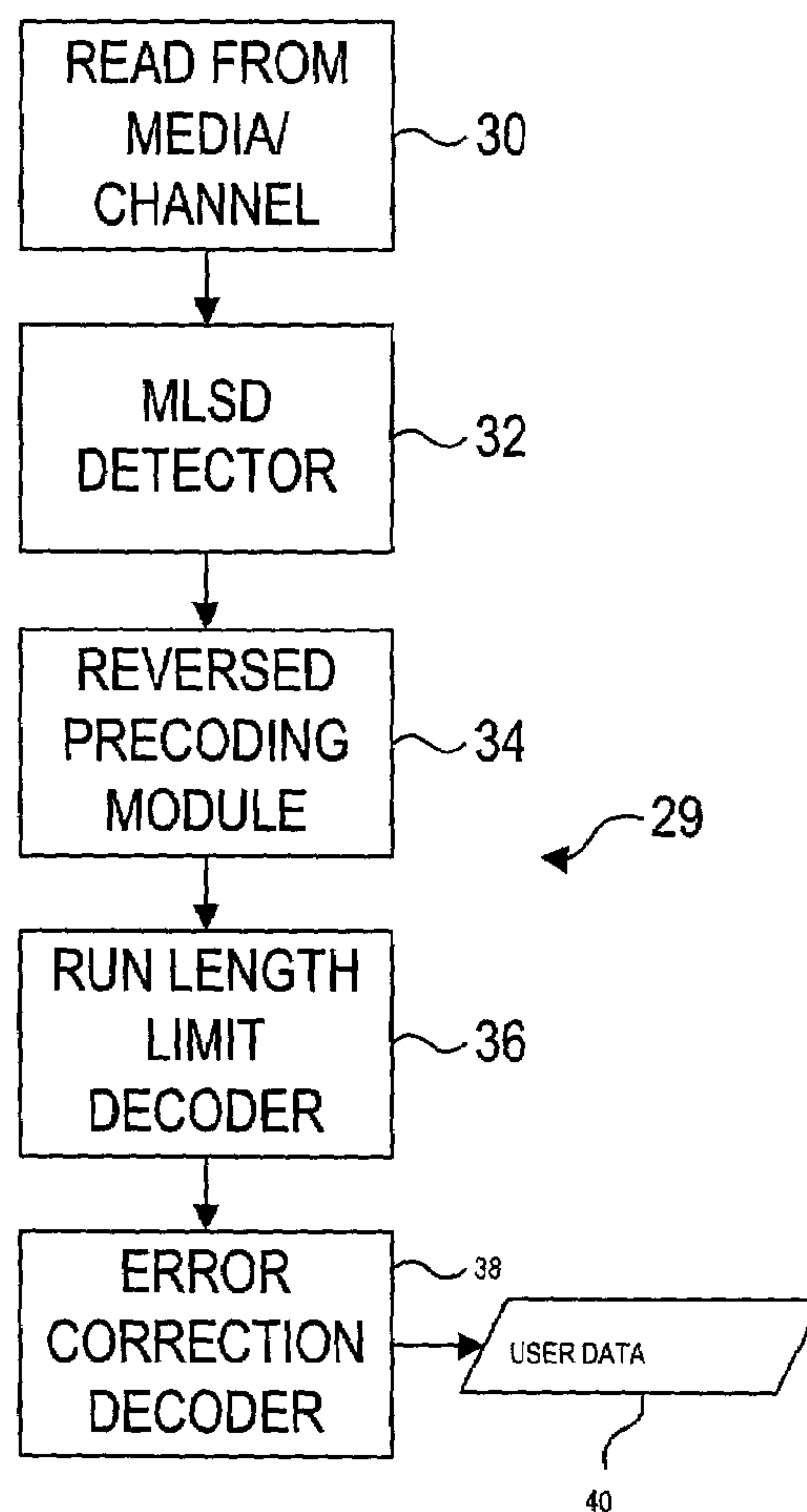
FIG. 2 (Prior Art)
