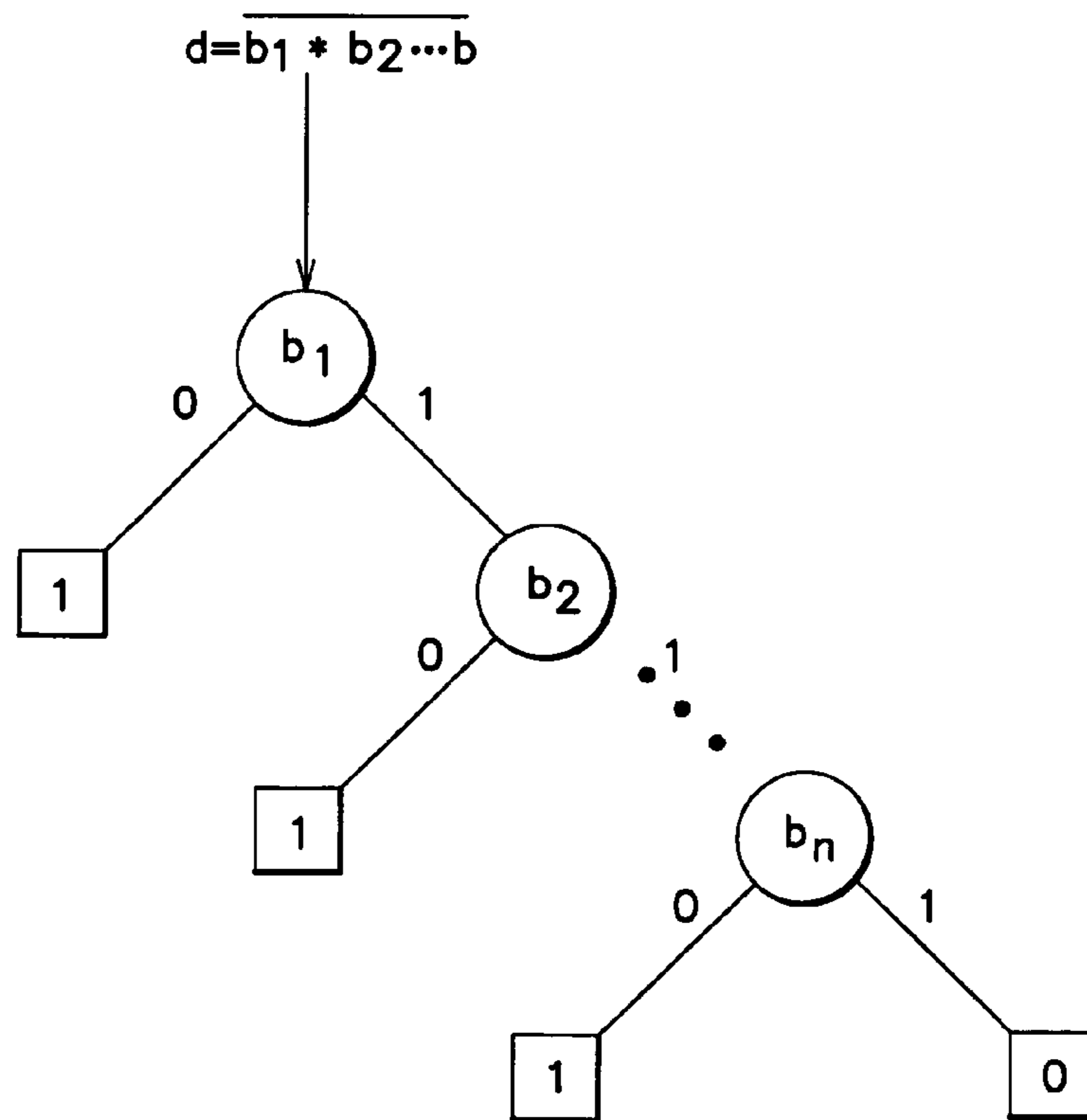
FIG. 4 (Prior Art)
