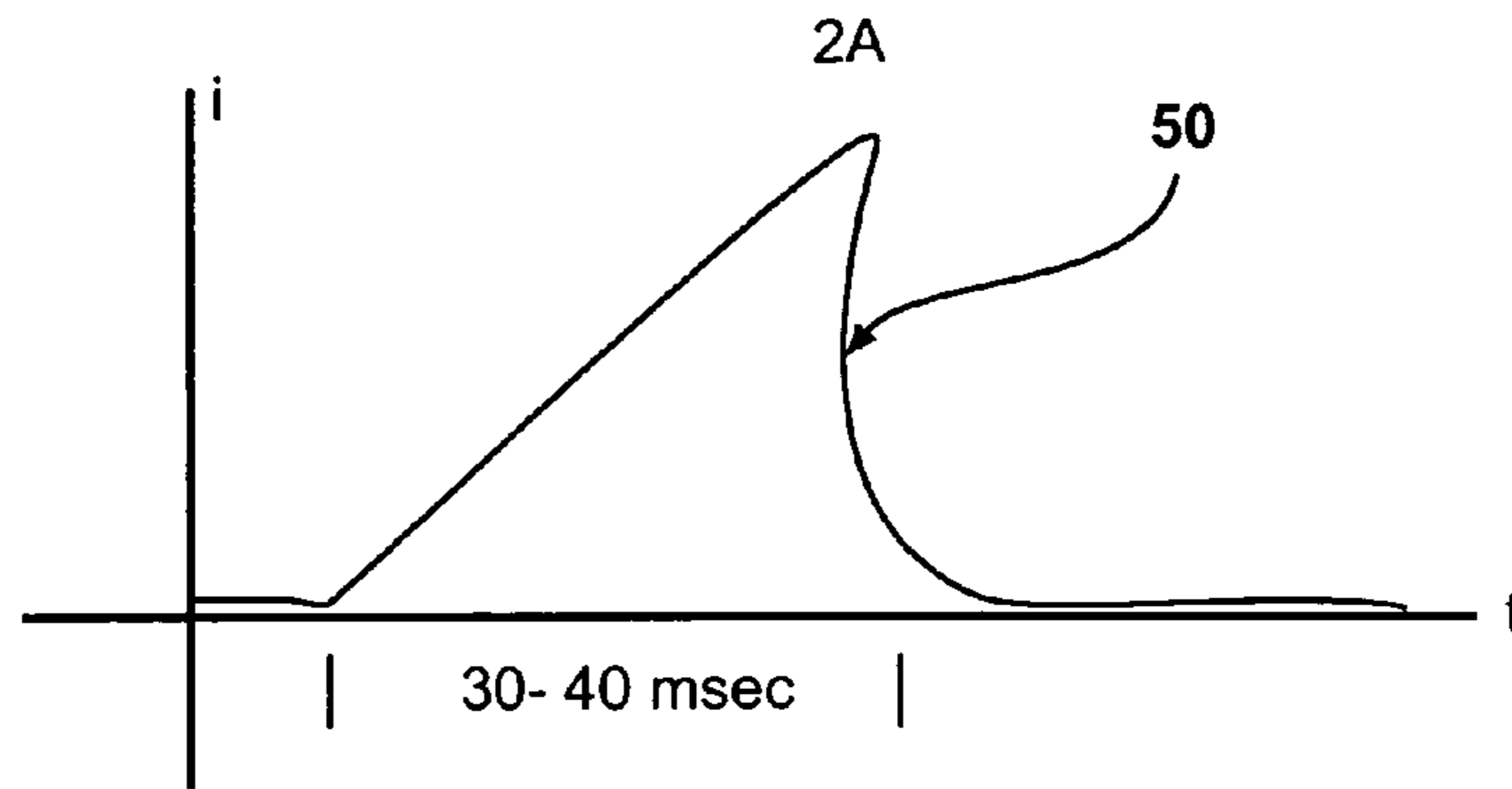
FIG - 3A Drive Coil Current
