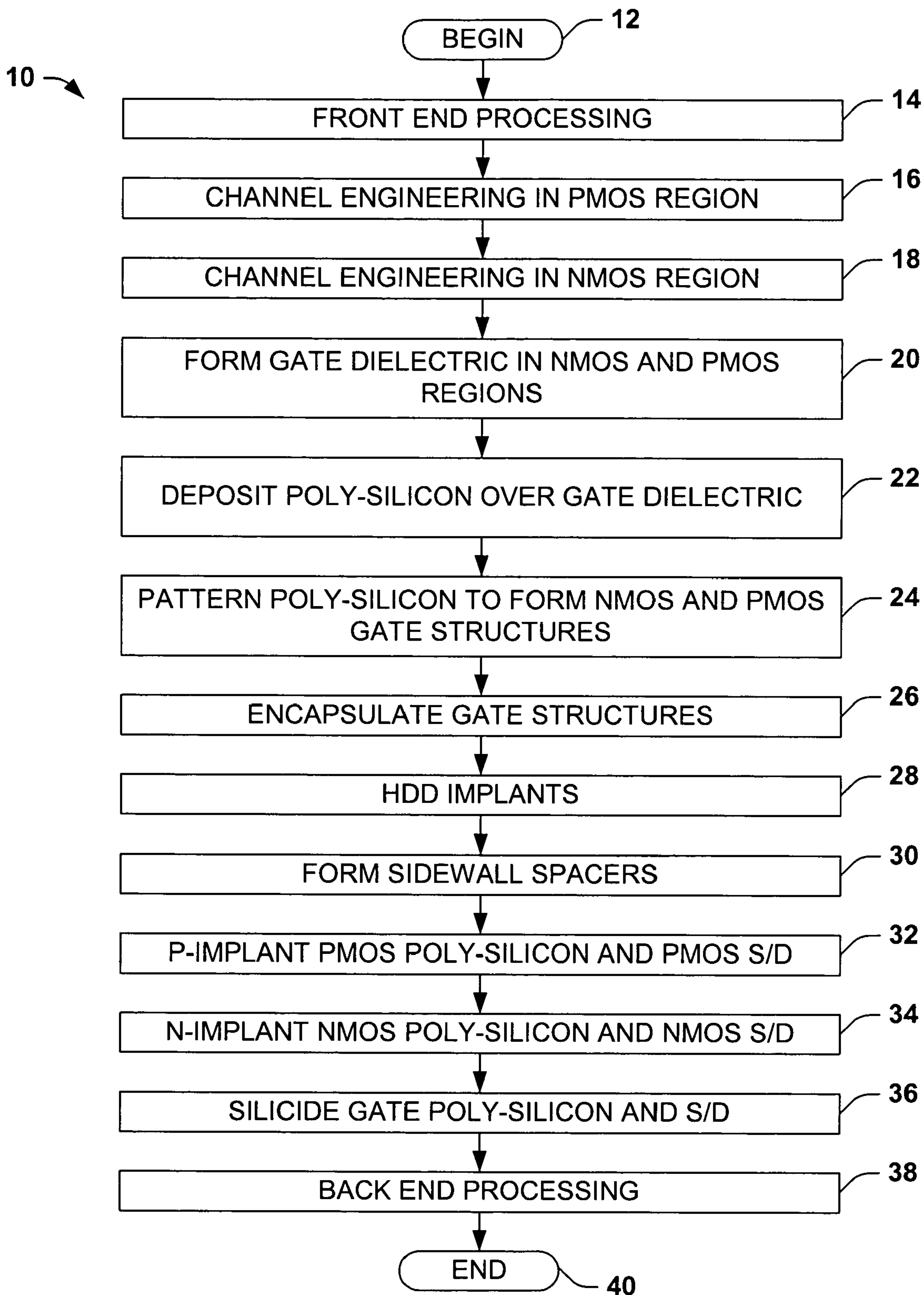
FIG. 1 (PRIOR ART)
