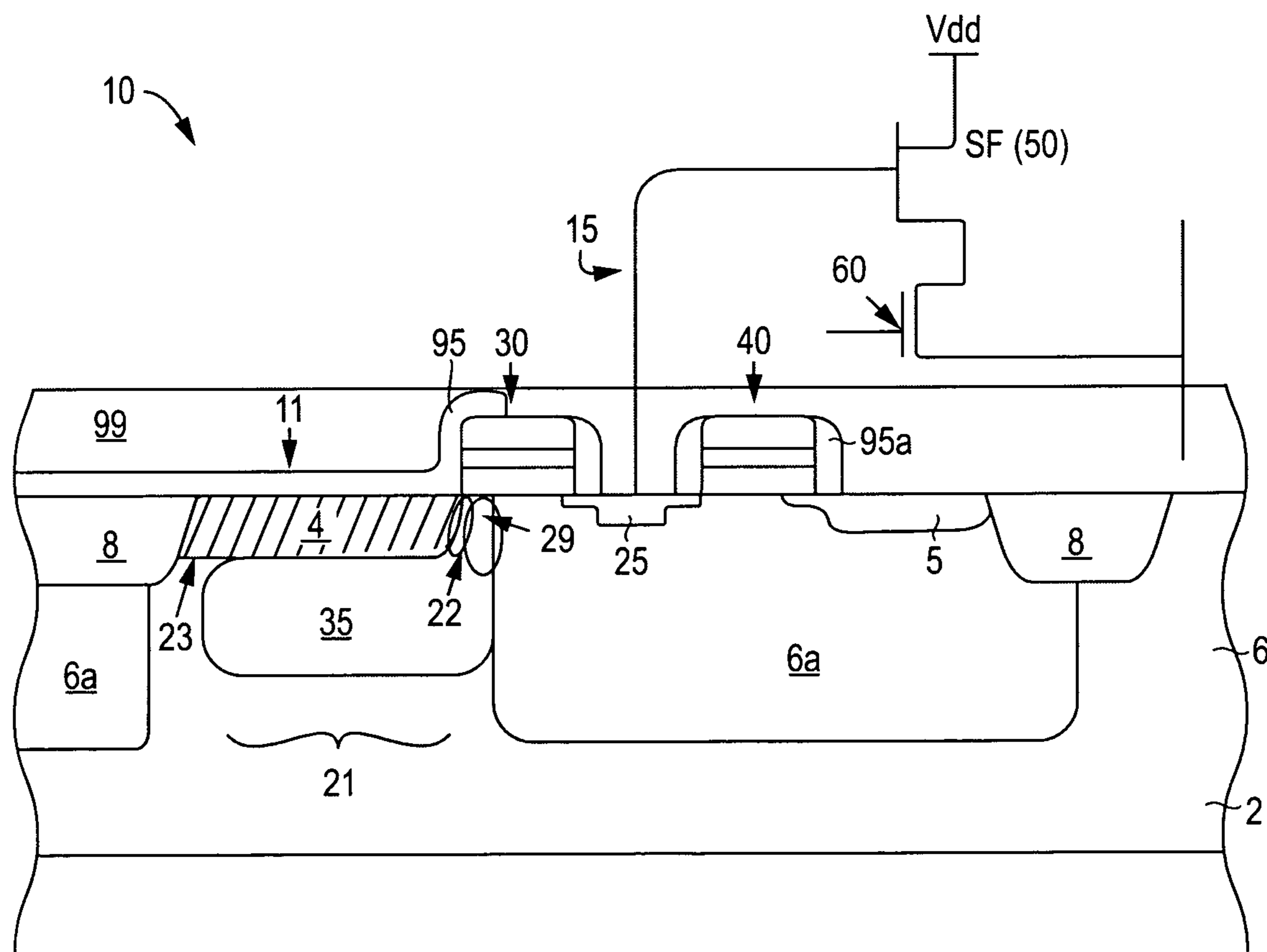
FIG. 2 PRIOR ART
