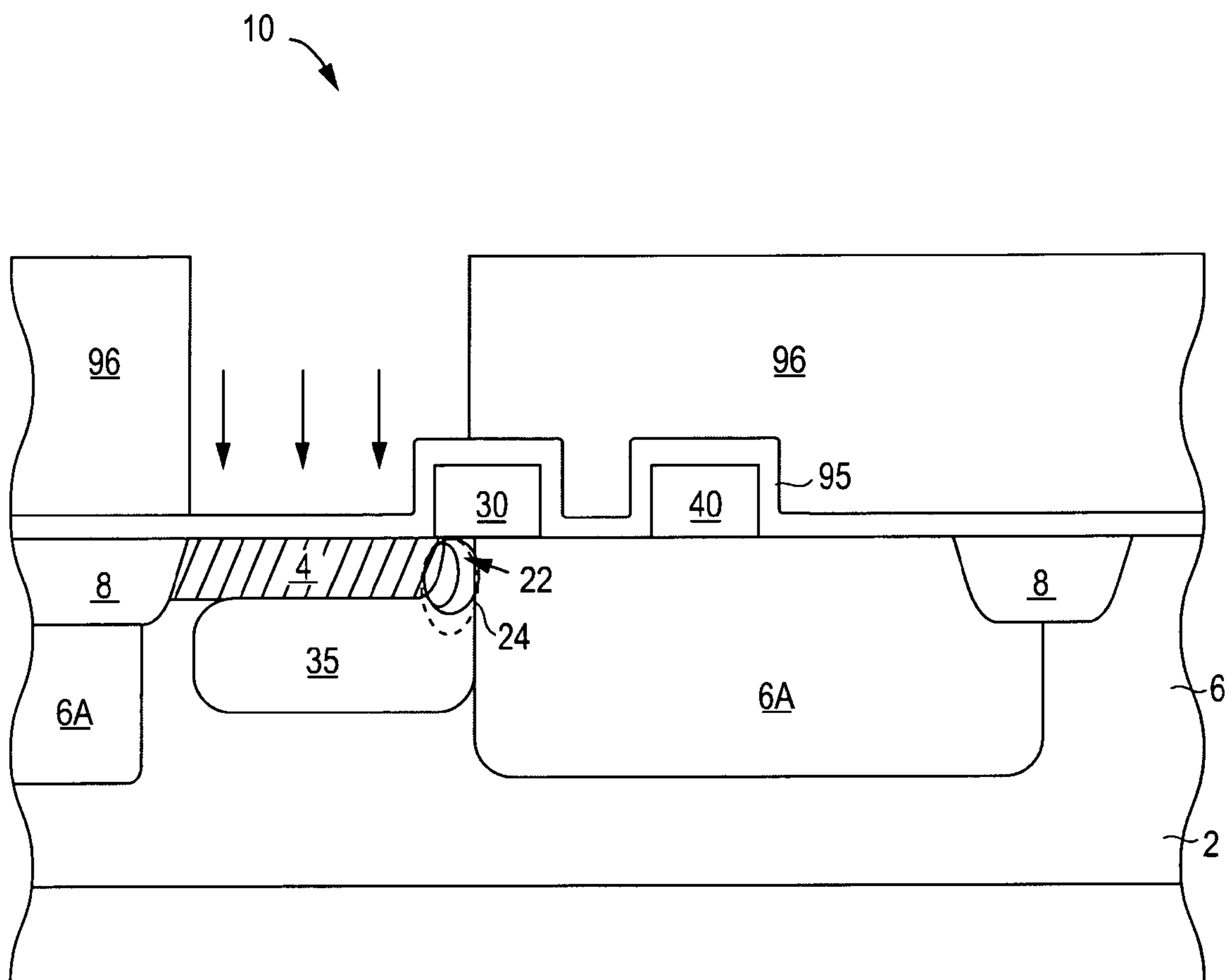
FIG. 3 PRIOR ART
