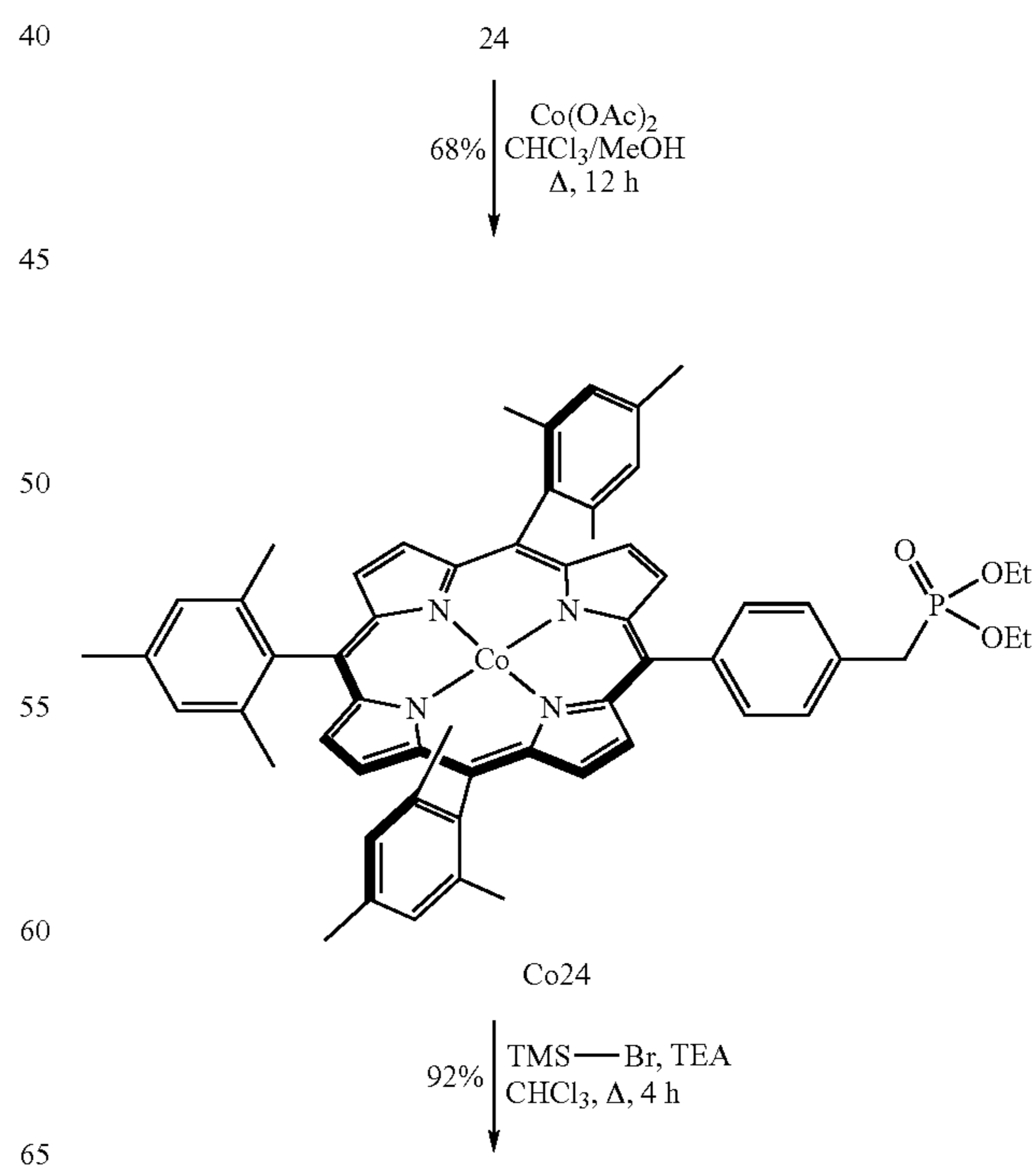
Scheme 14
