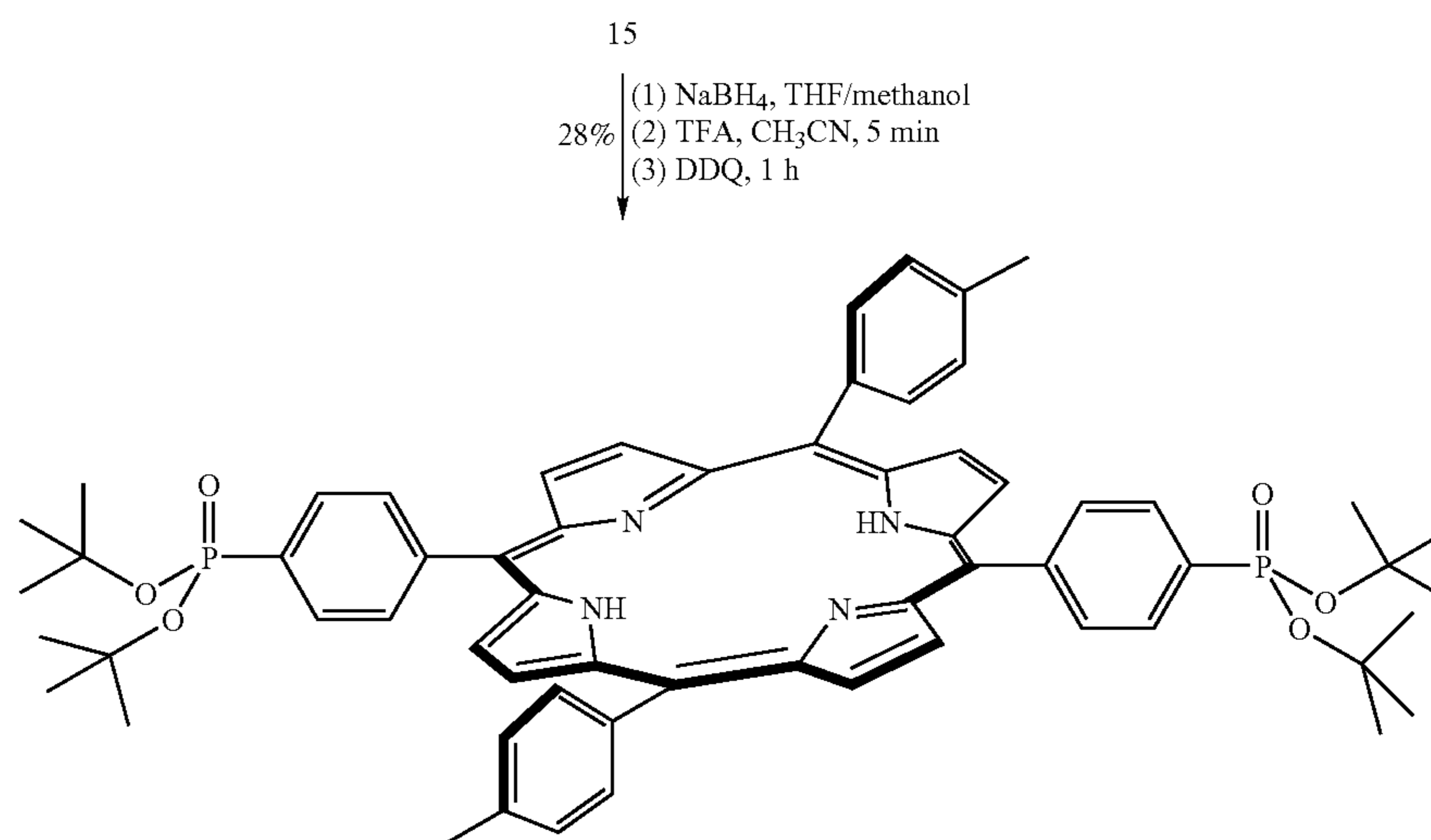
Scheme 7
