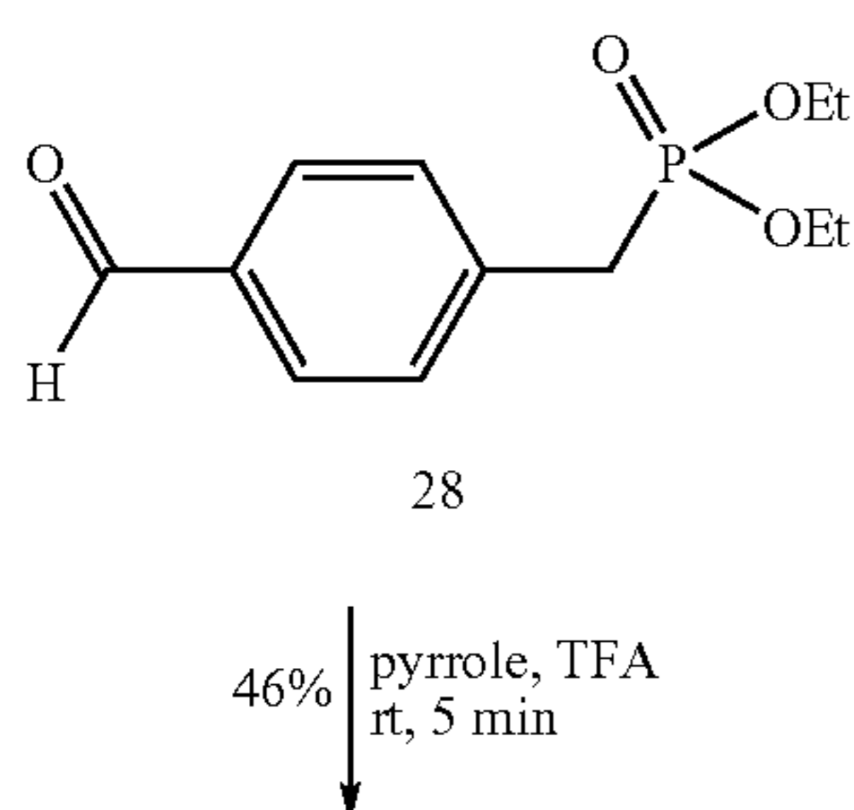
Scheme 12
