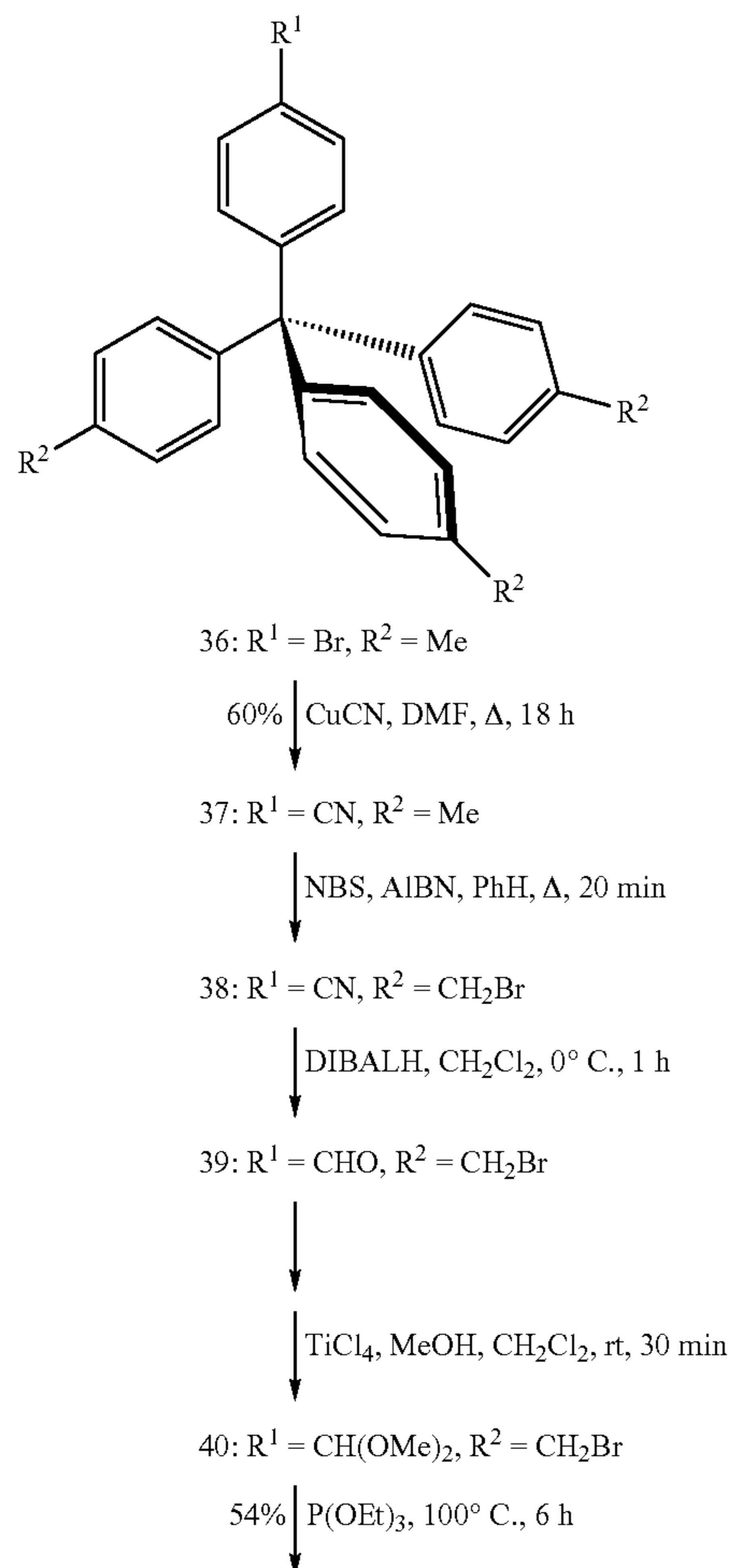
Scheme 15
