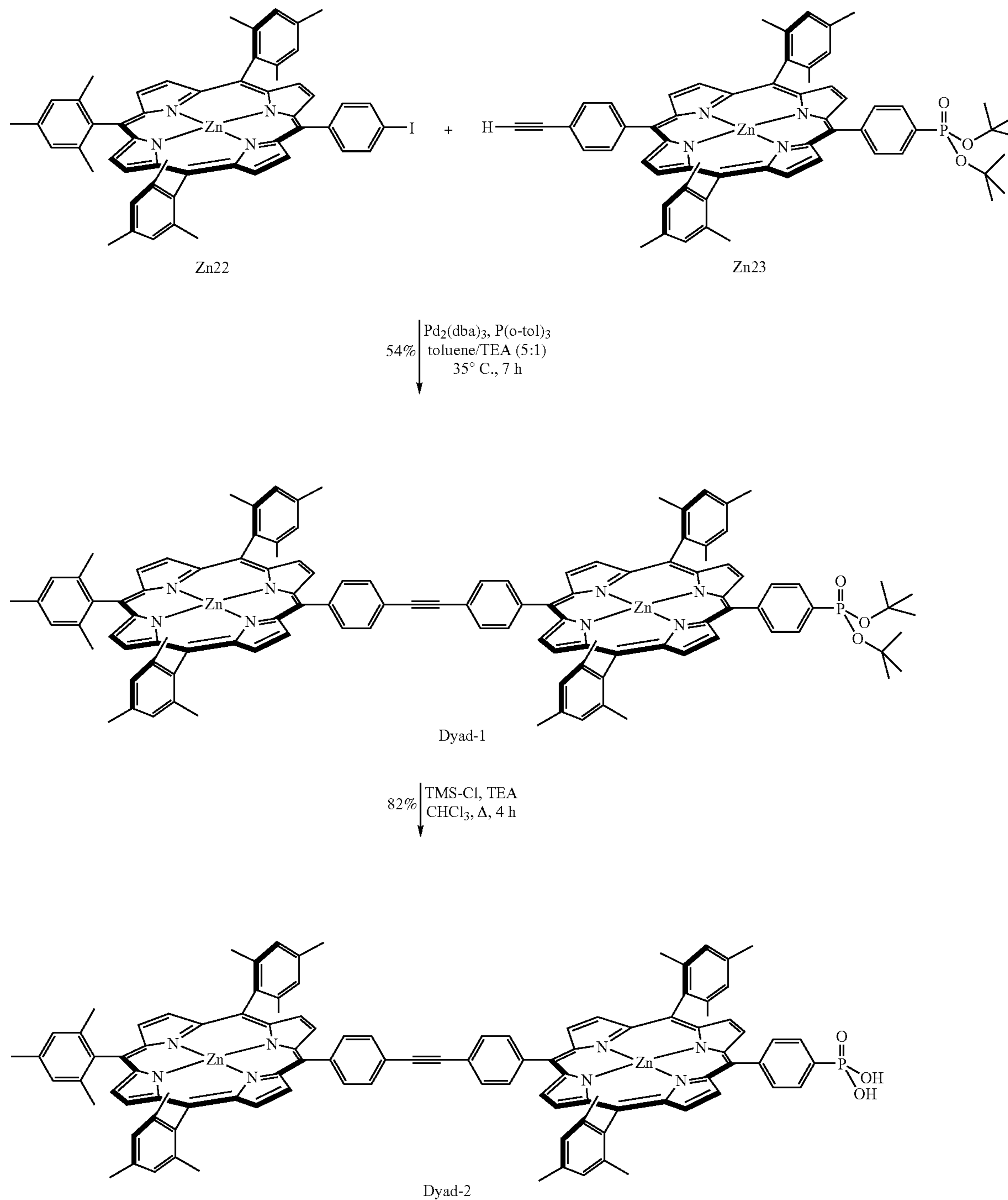
Scheme 9
