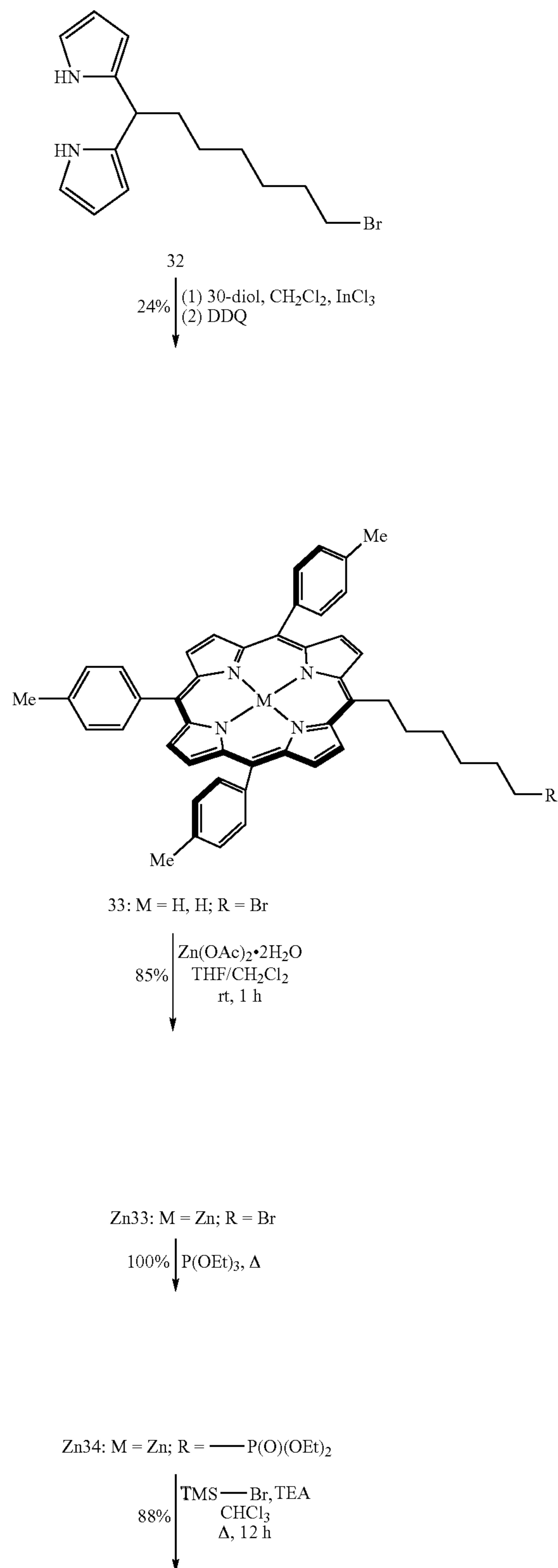
Scheme 13
