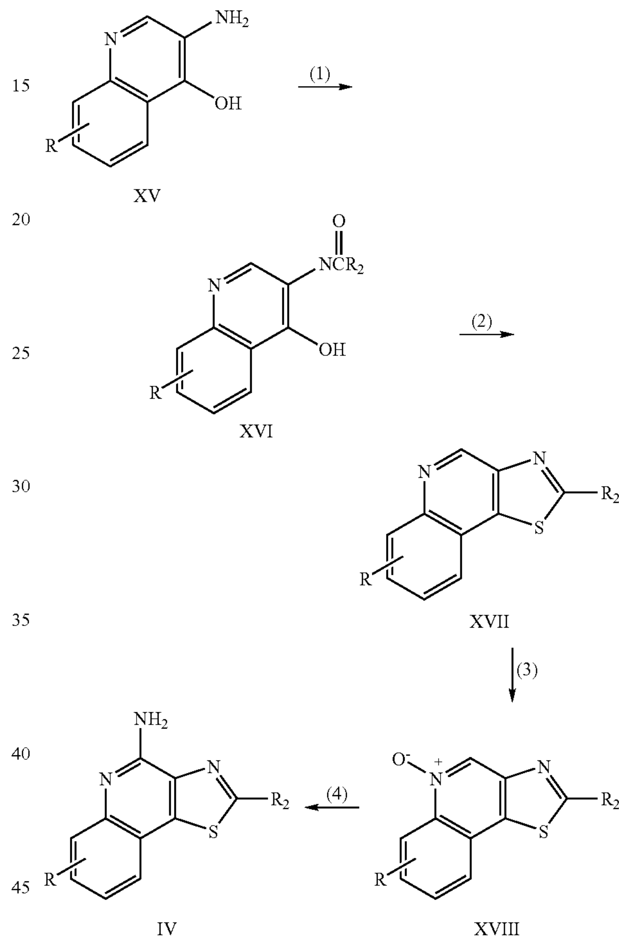
Reaction Scheme IV
