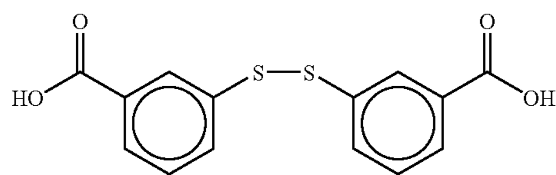
dithiosalicylic acid
