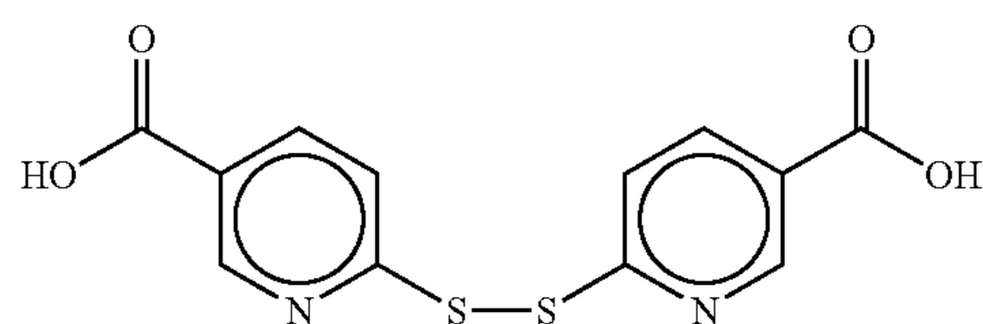
Dithionicotinic acid
