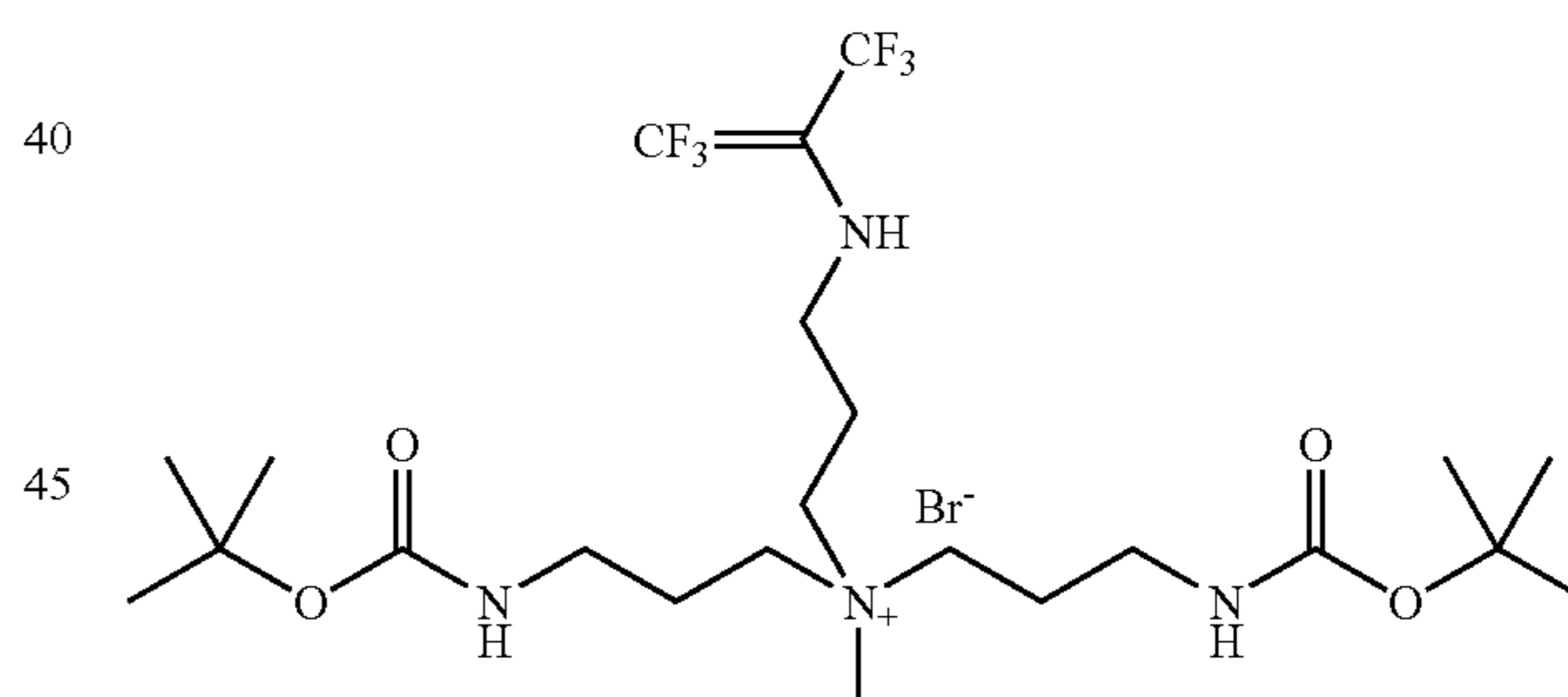
Compound 13
