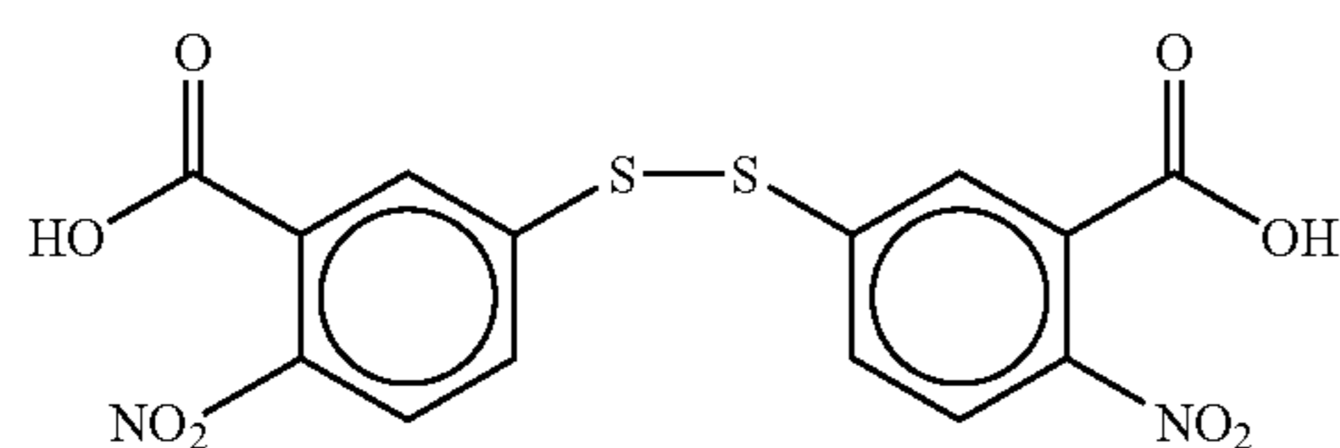
Ellman's reagent
