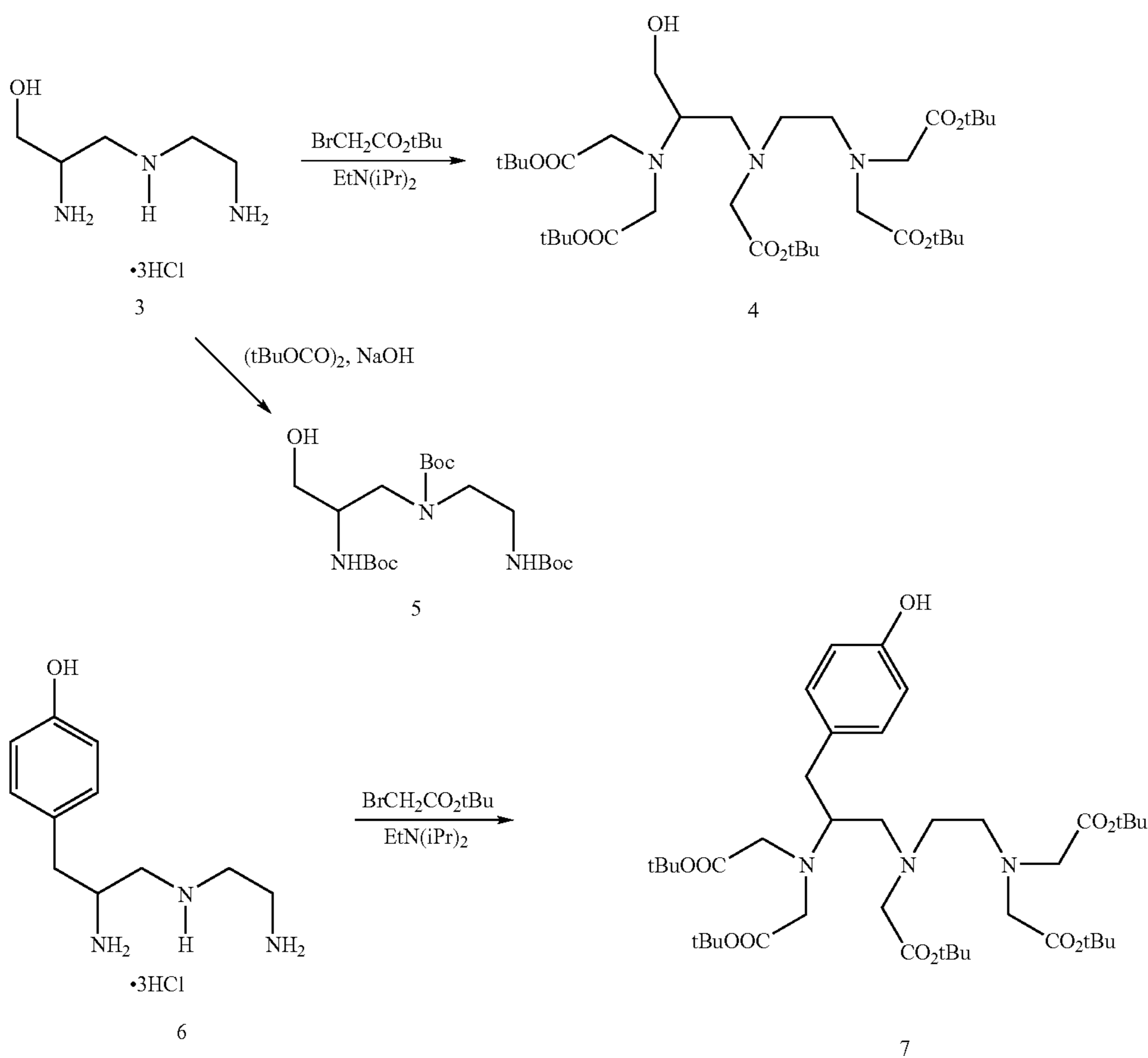
Scheme 1: Synthetic Intermediates
