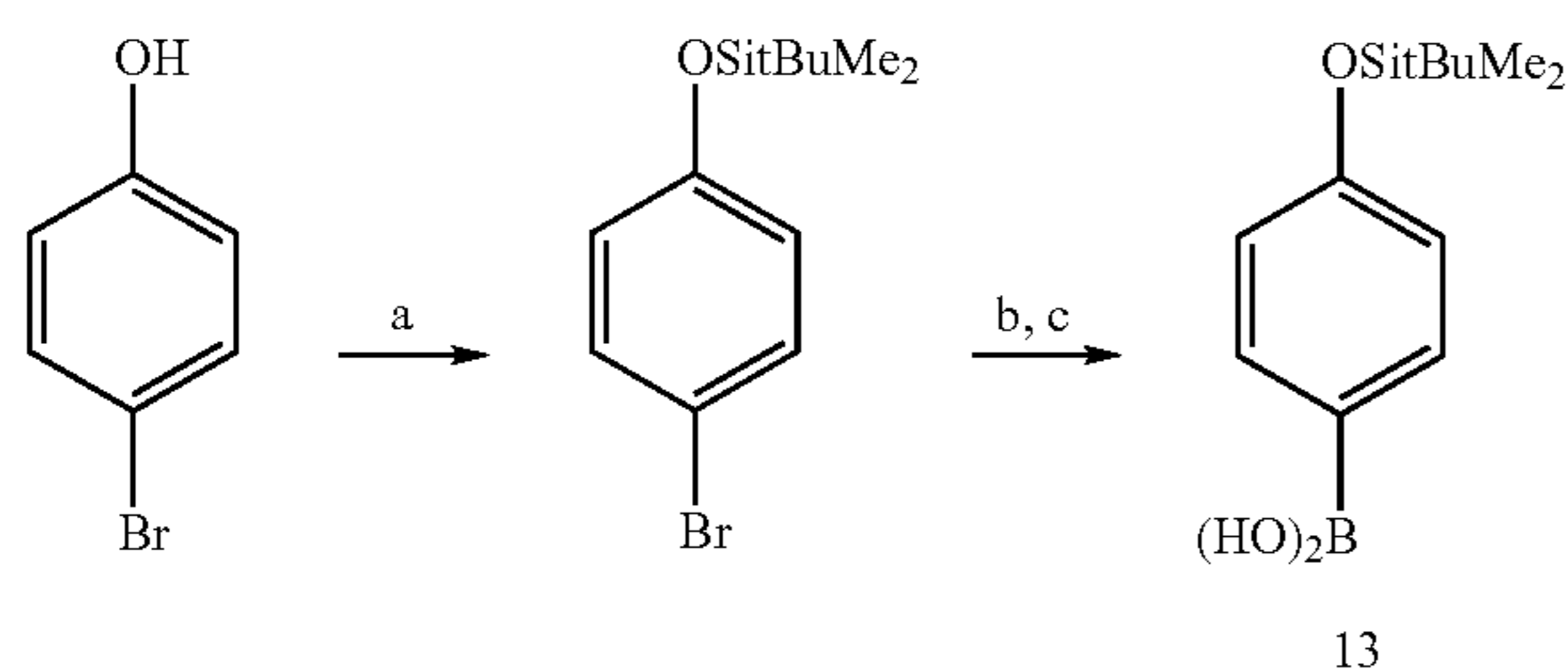
Scheme 2a: Synthesis of boronic acid 13
