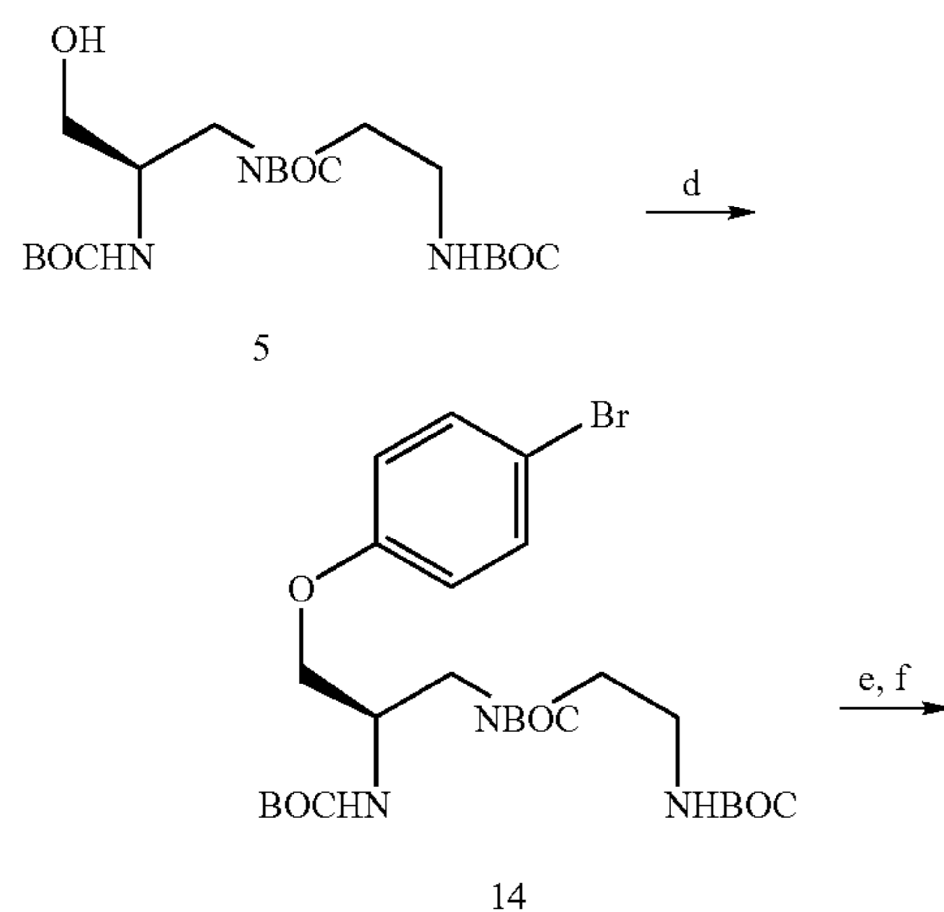
Scheme 2b: More Preferred Synthesis of Gd Complex 1
