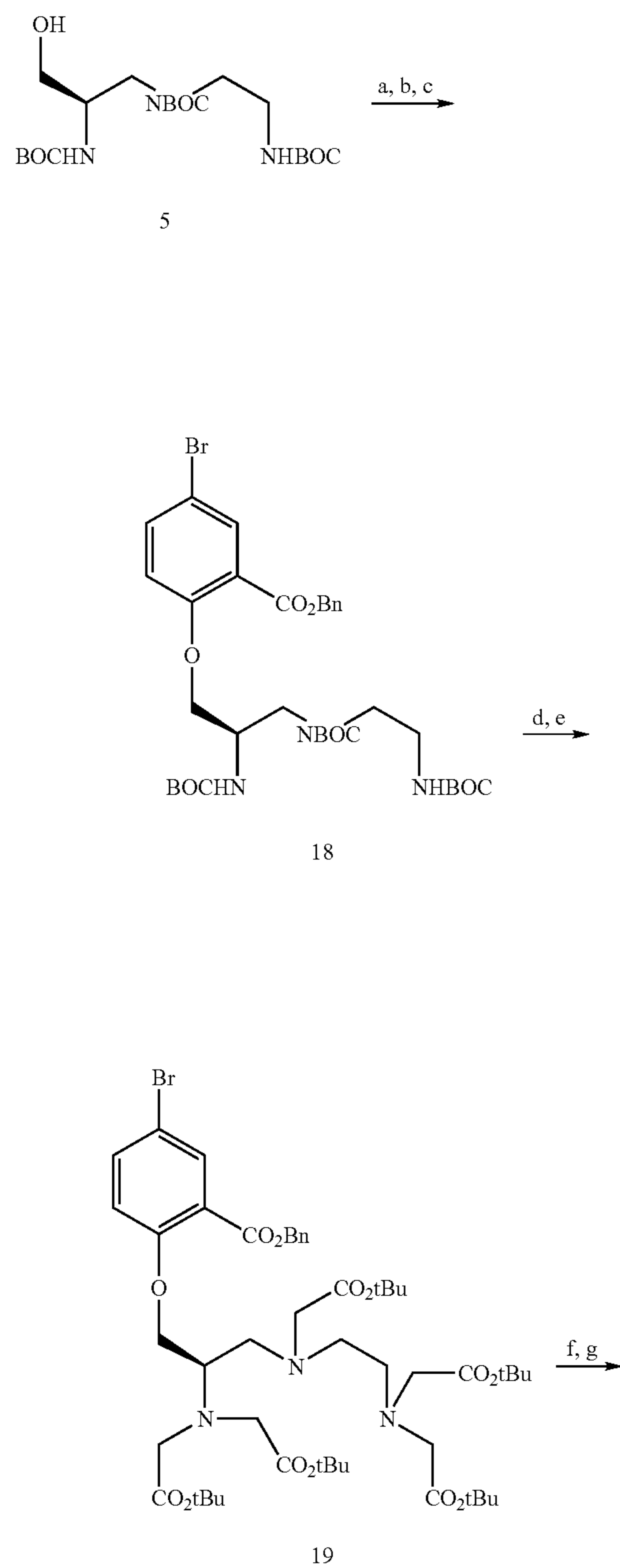
Scheme 3b: More Preferred Synthesis of Gd Complex 2
