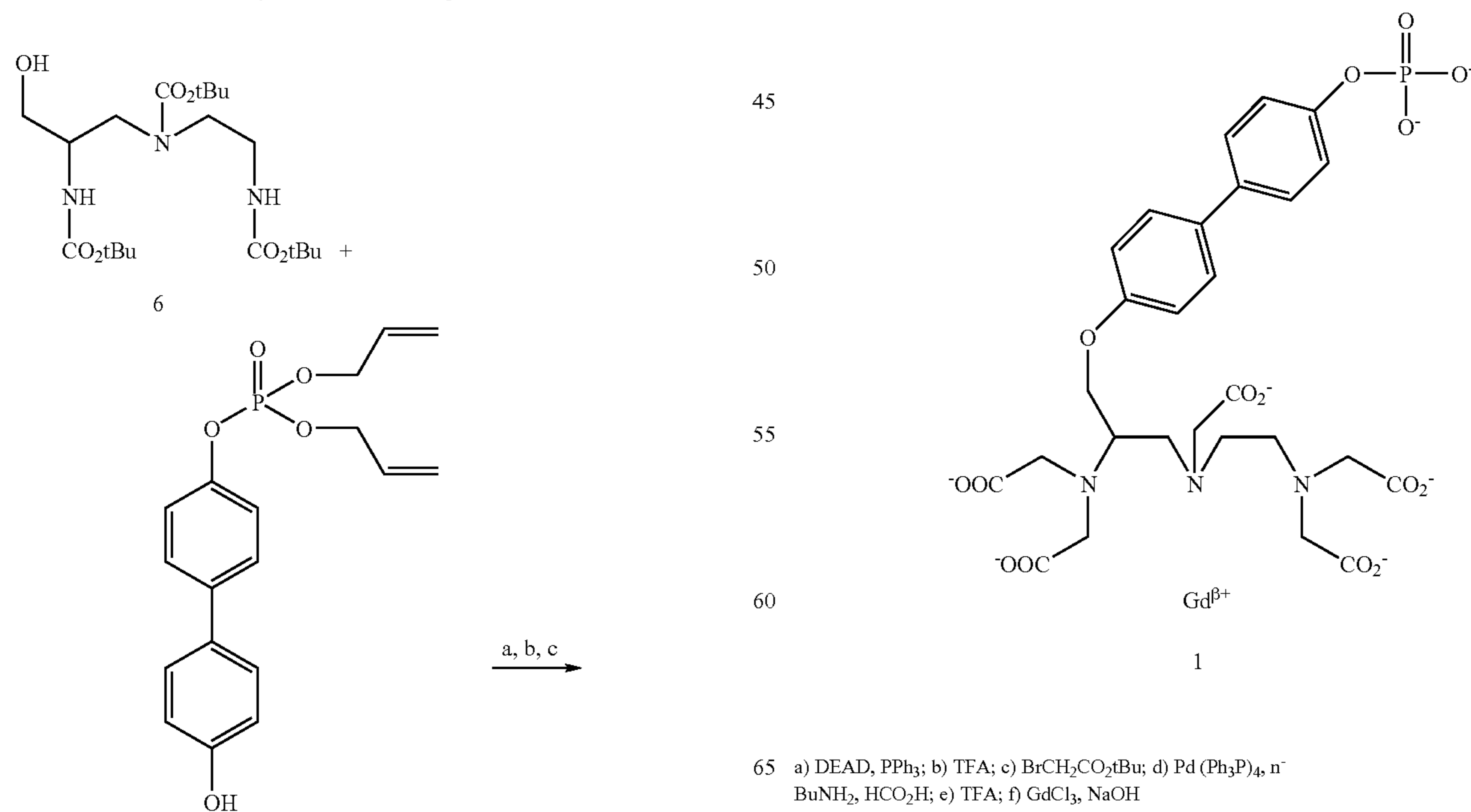
Scheme 2: Synthesis of Gd Complex 1
