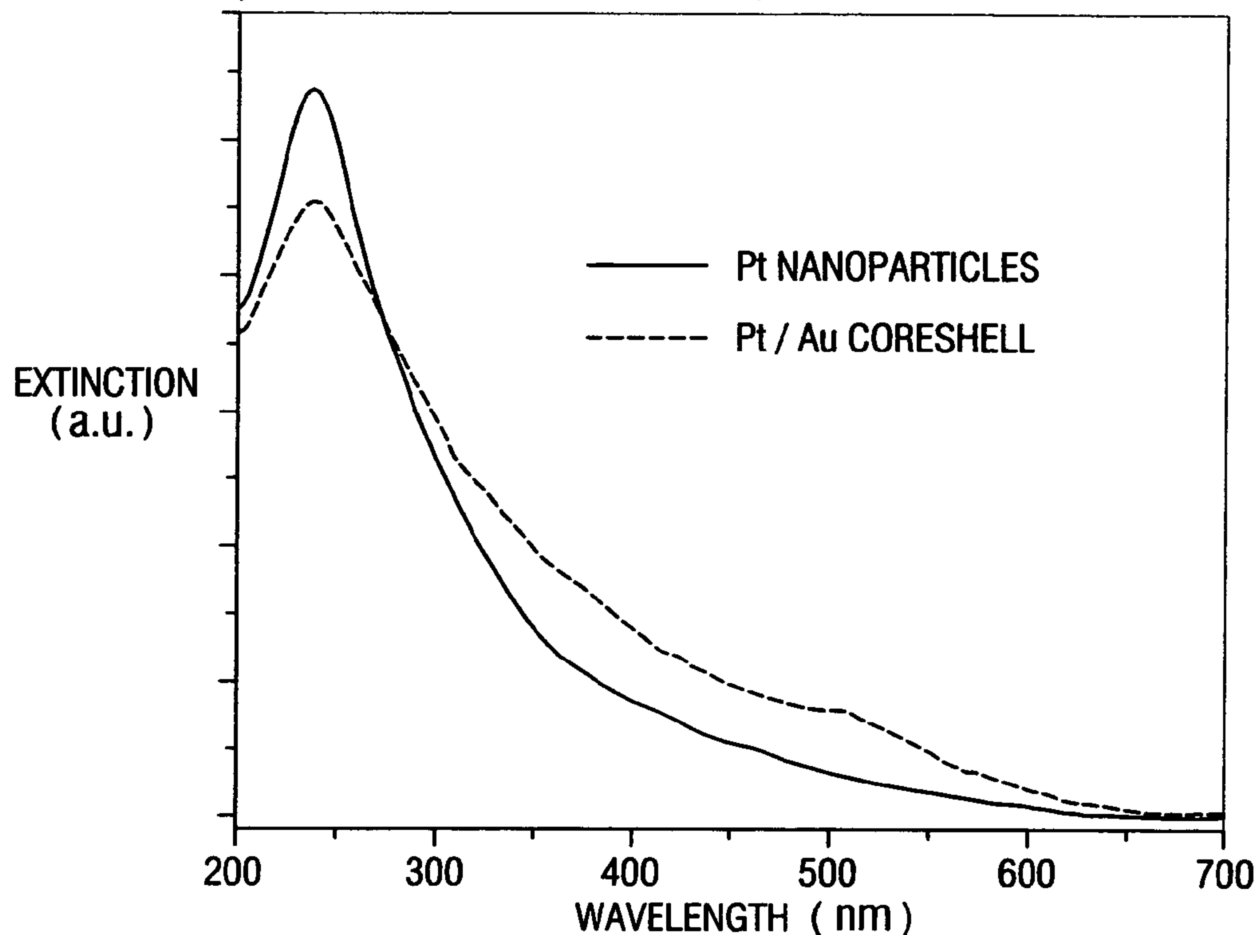
UV-VIS SPECTRA OF Pt AND Pt / Au CORESHELL NANOPARTICLES
