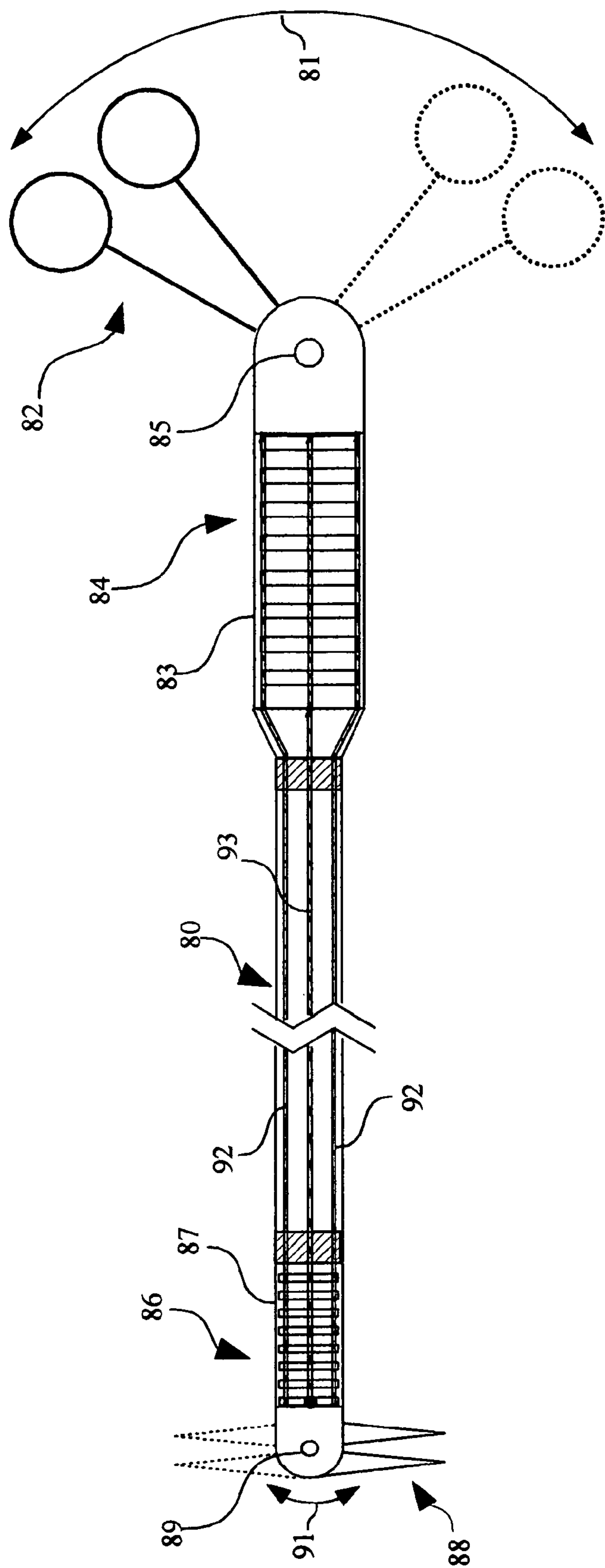
Figure 11A
