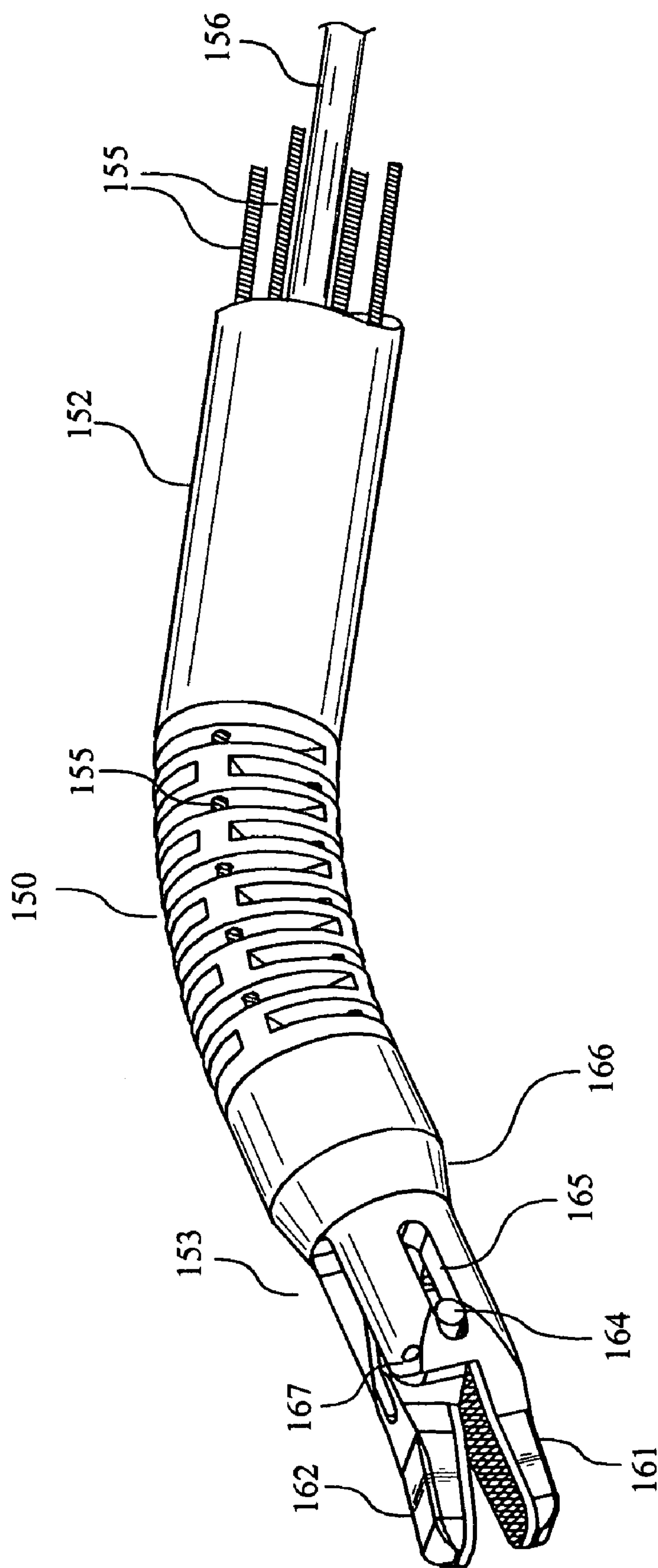
Figure 22A
