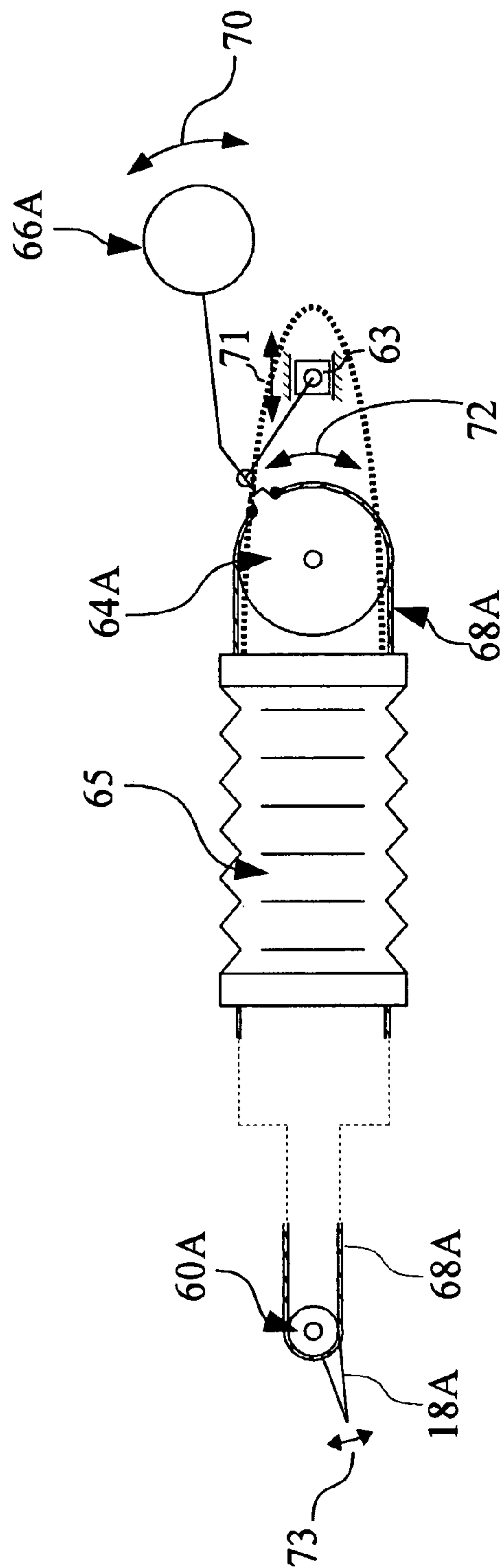
Figure 10B
