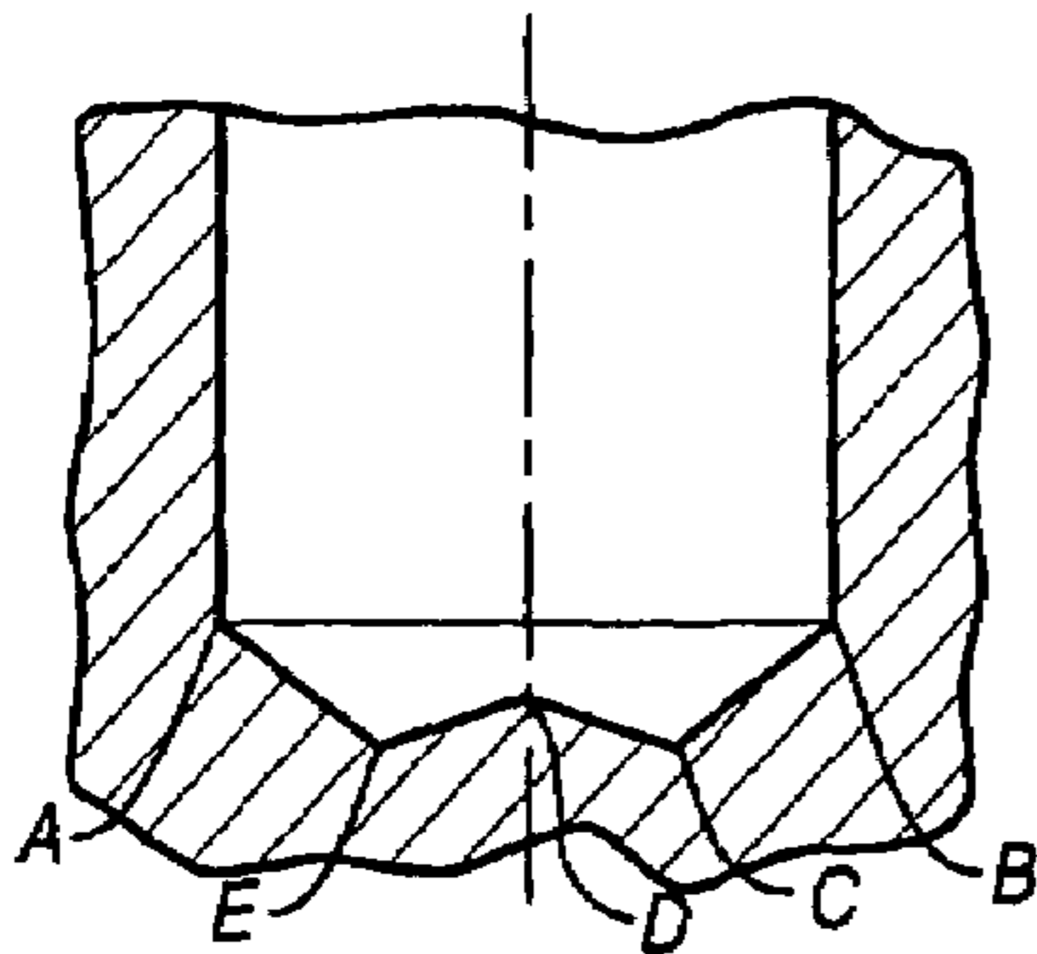
FIGURE 11A TYPICAL PRIOR ART
