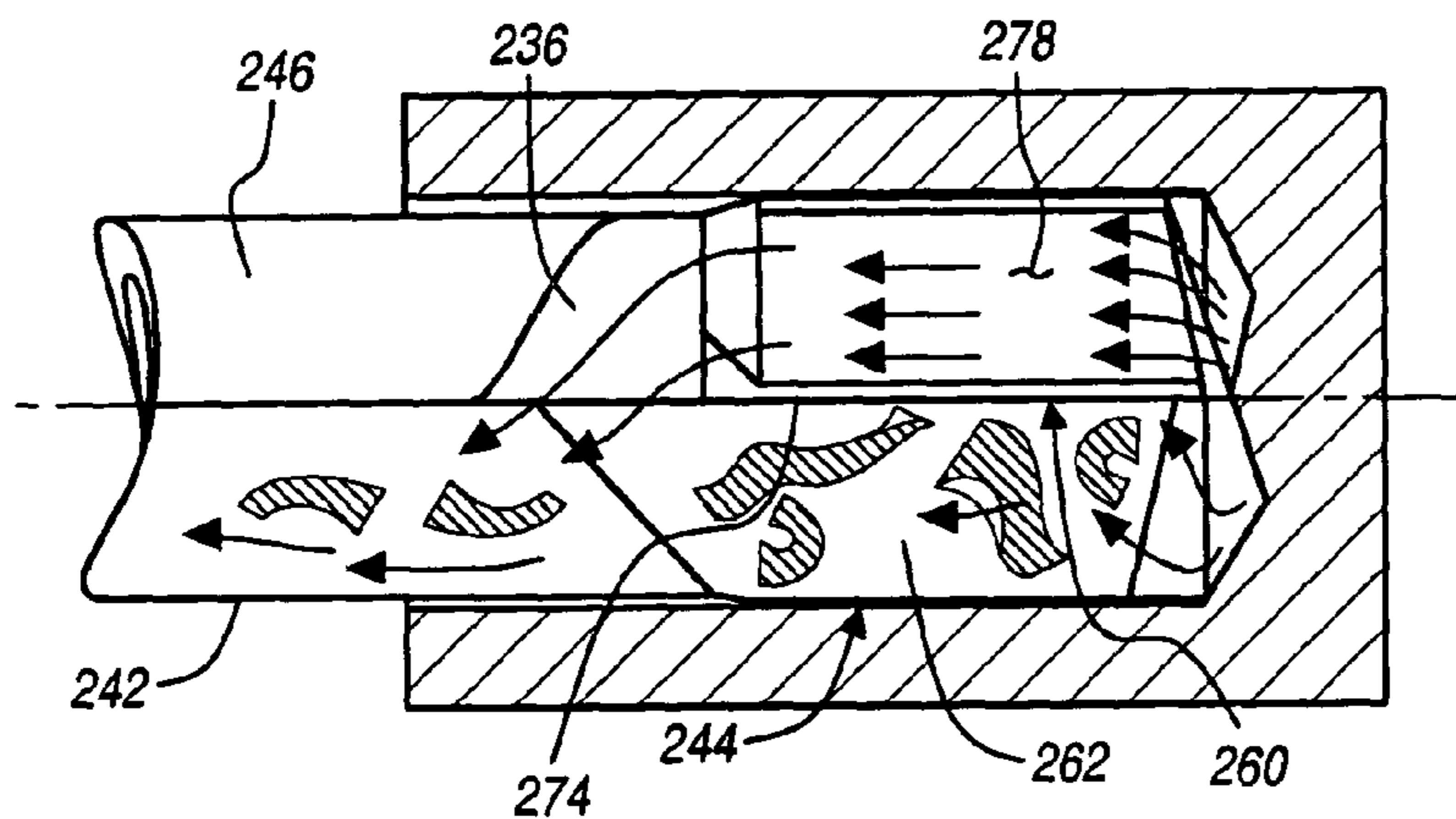
FIGURE 36 VIEW Z
