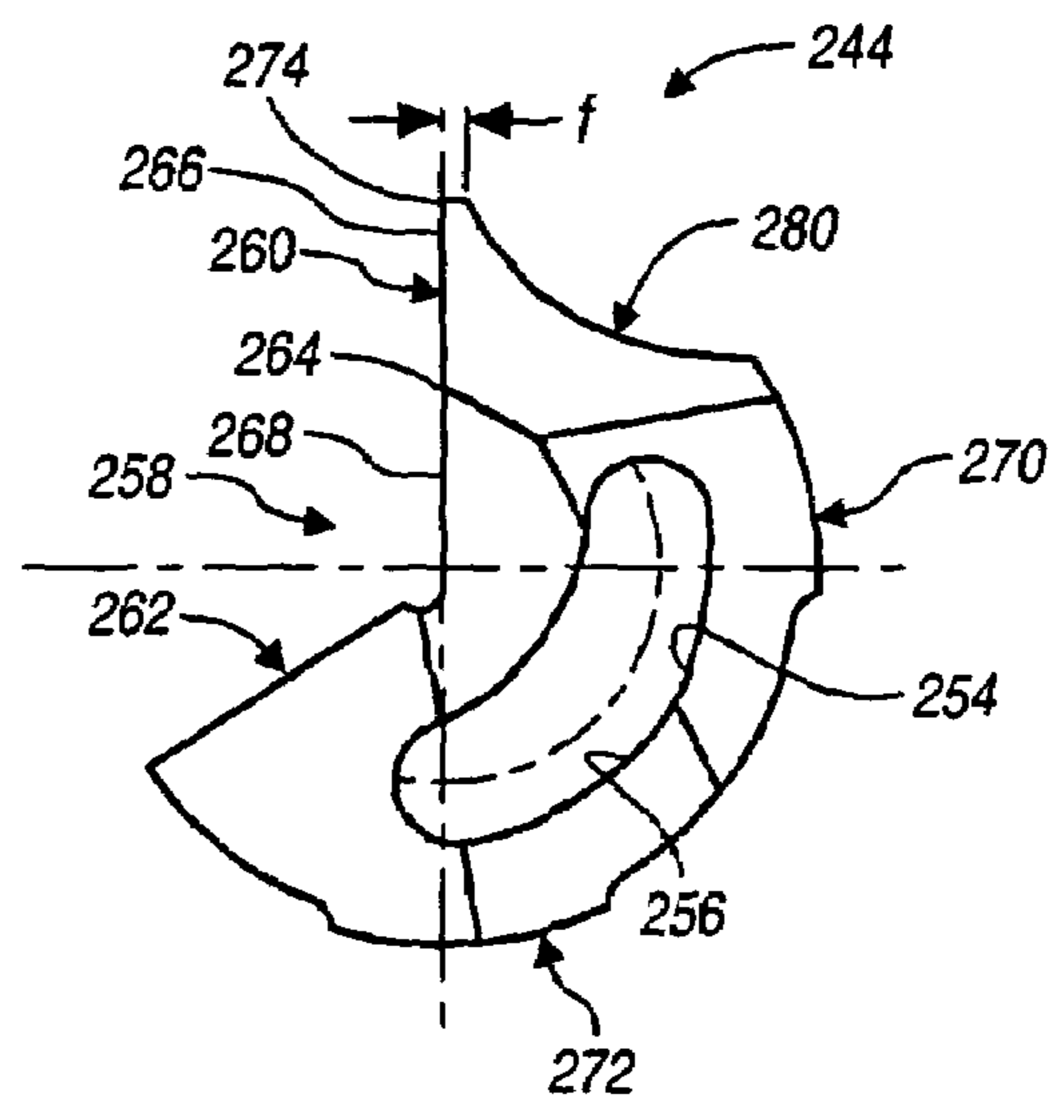
FIGURE 31 VIEW V2
