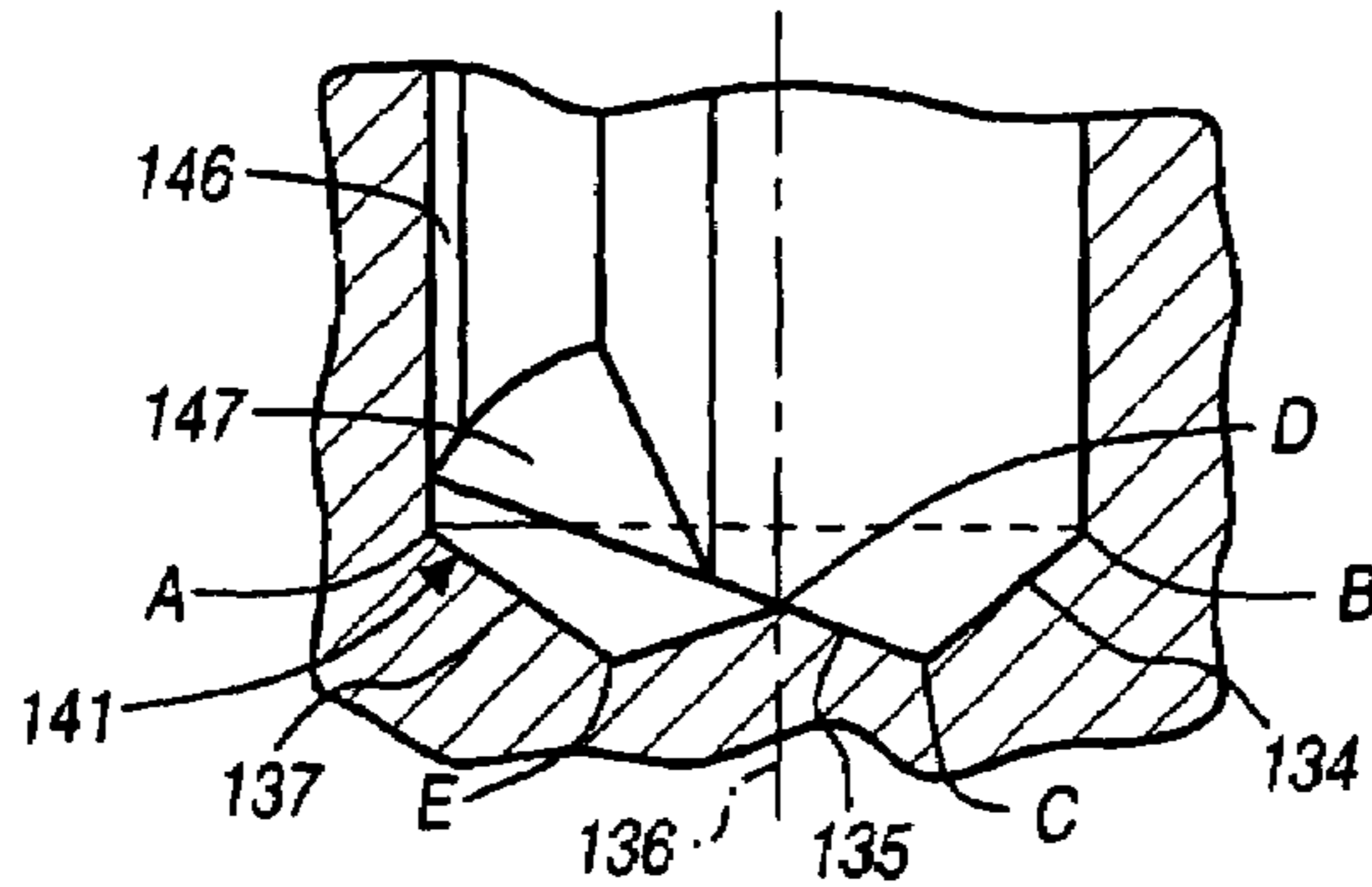
FIGURE 11 PRIOR ART
