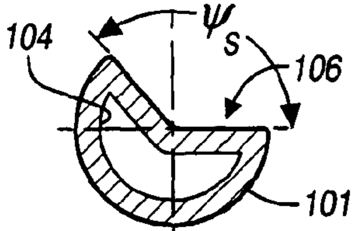
FIGURE 2 SECTION A-A PRIOR ART
