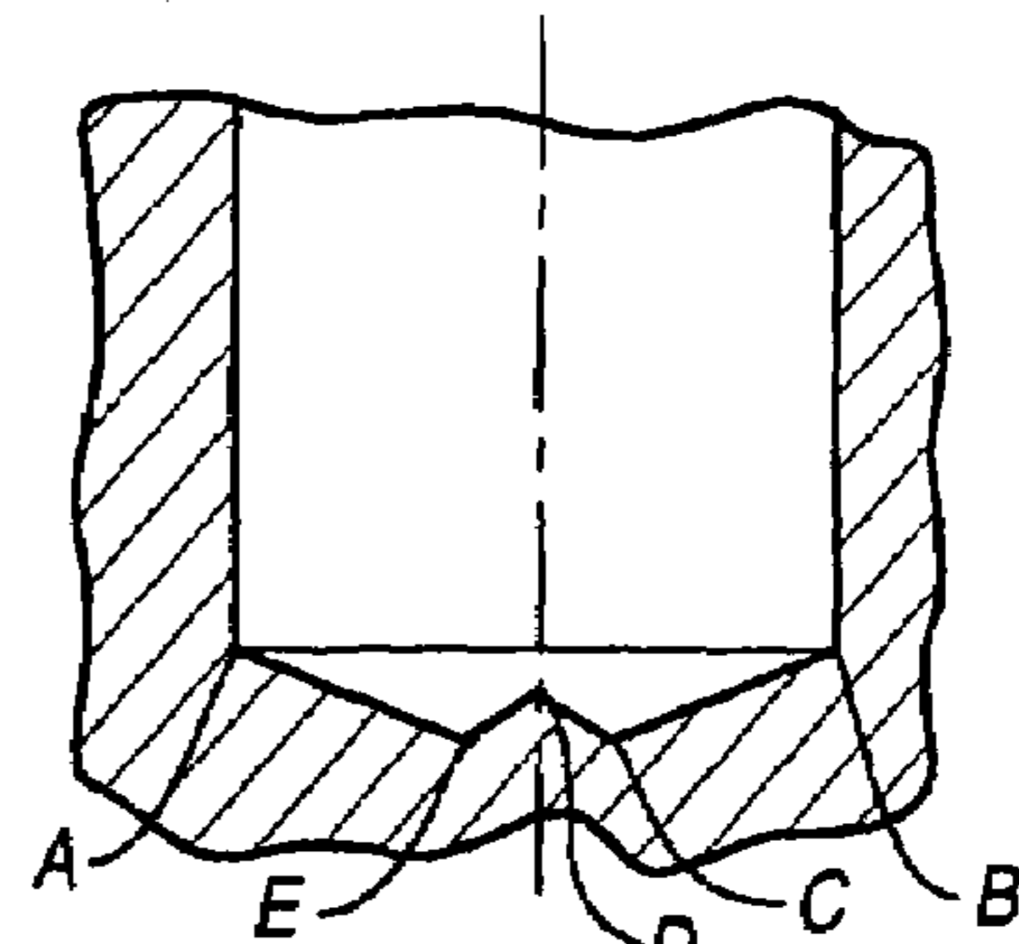
FIGURE 11C BRITTLE PRIOR ART
