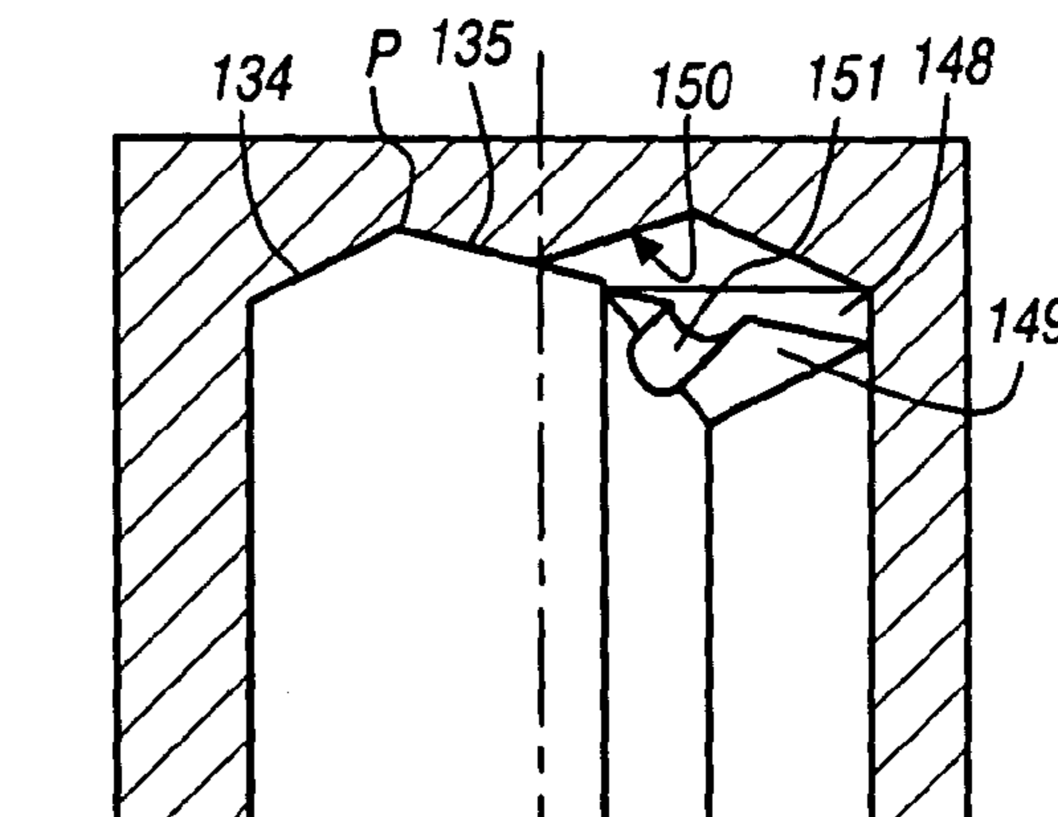
FIGURE 16 PRIOR ART
