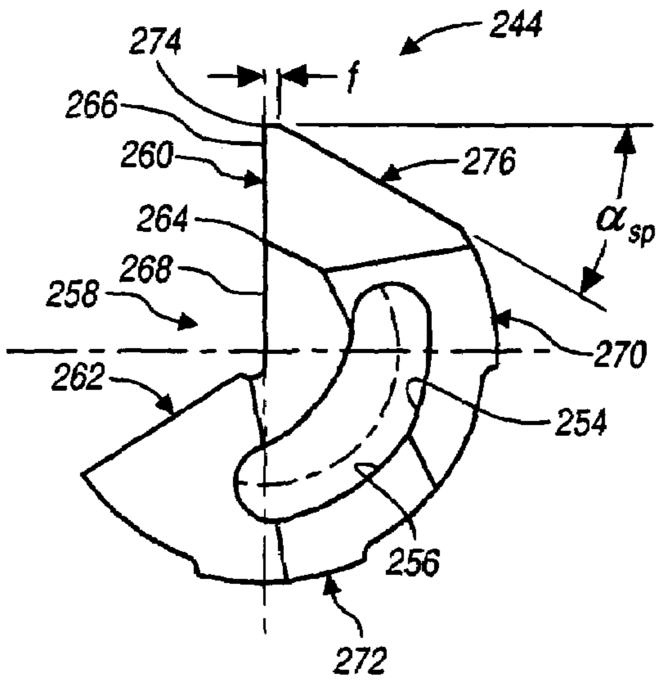
FIGURE 30 VIEW V1
