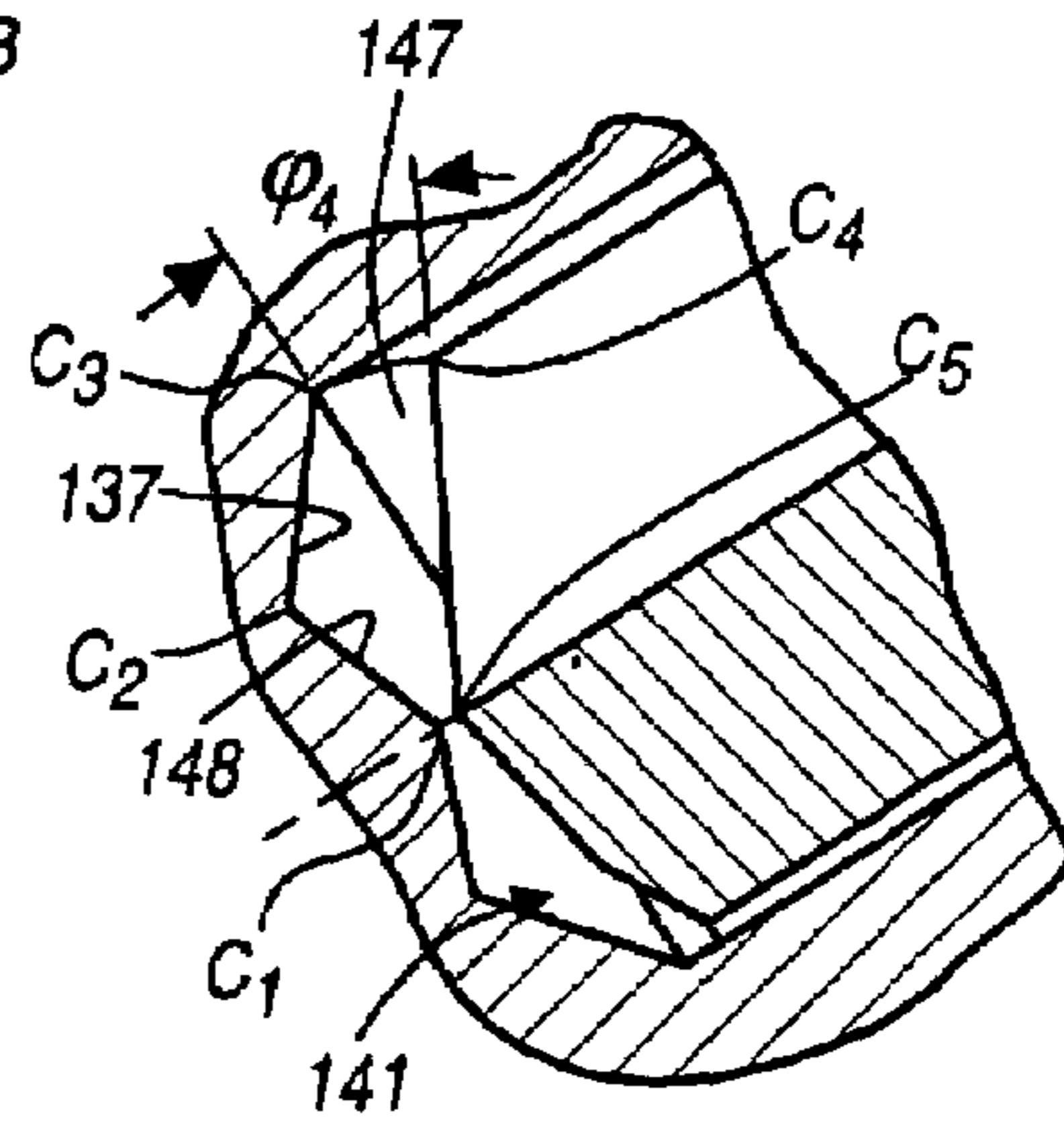
FIGURE 13 SECTION Q2-Q2 PRIOR ART
