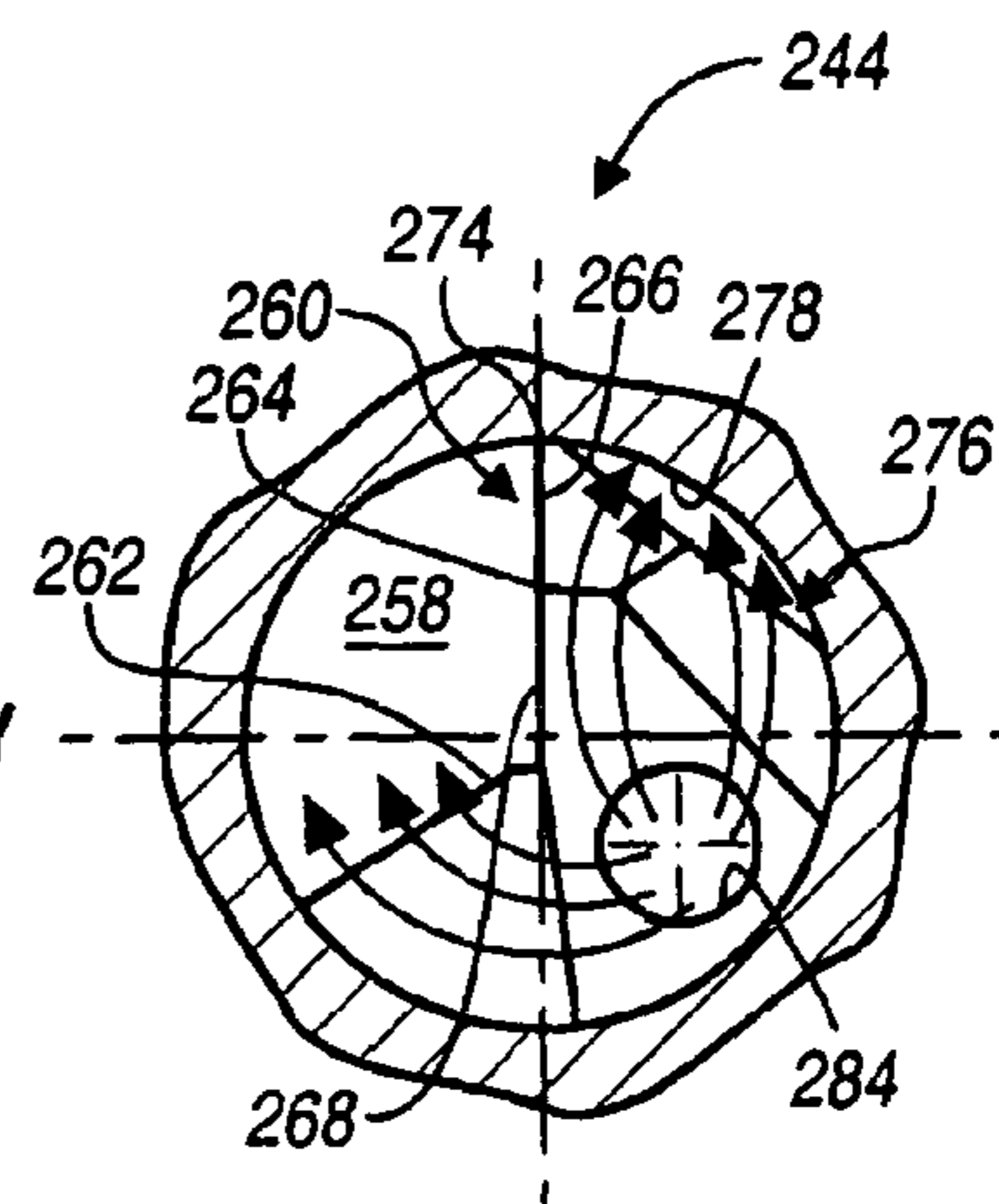
FIGURE 35 VIEW Y
