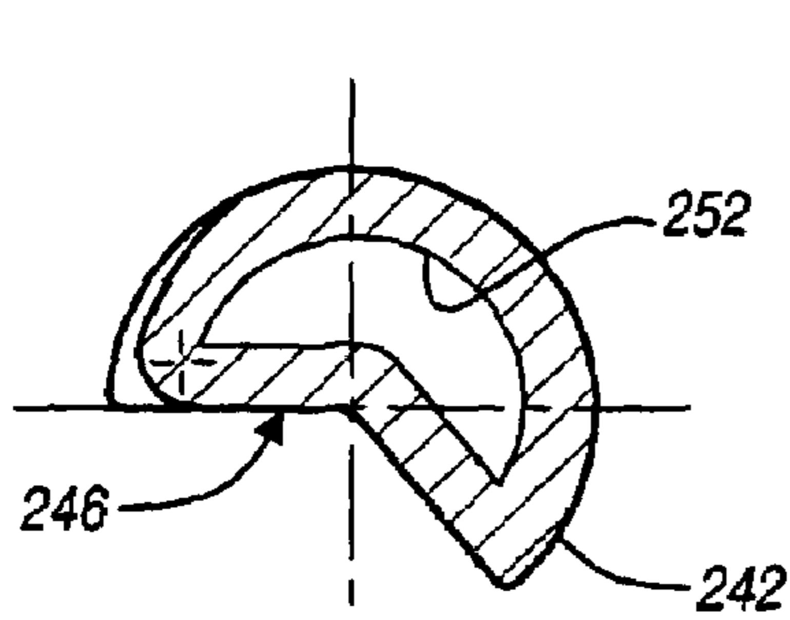
FIGURE 33 SECTION X-X
