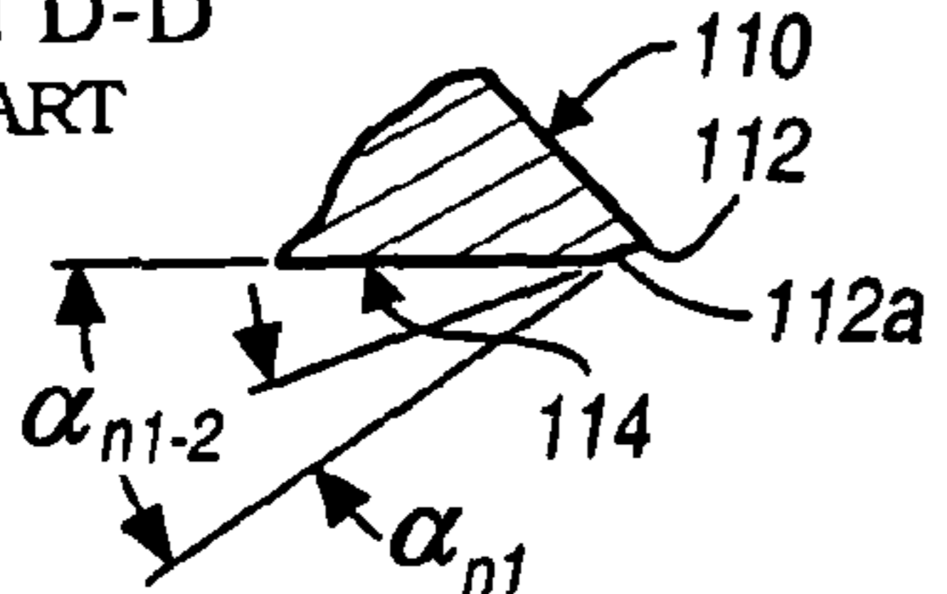
FIGURE 4 SECTION E-E PRIOR ART
