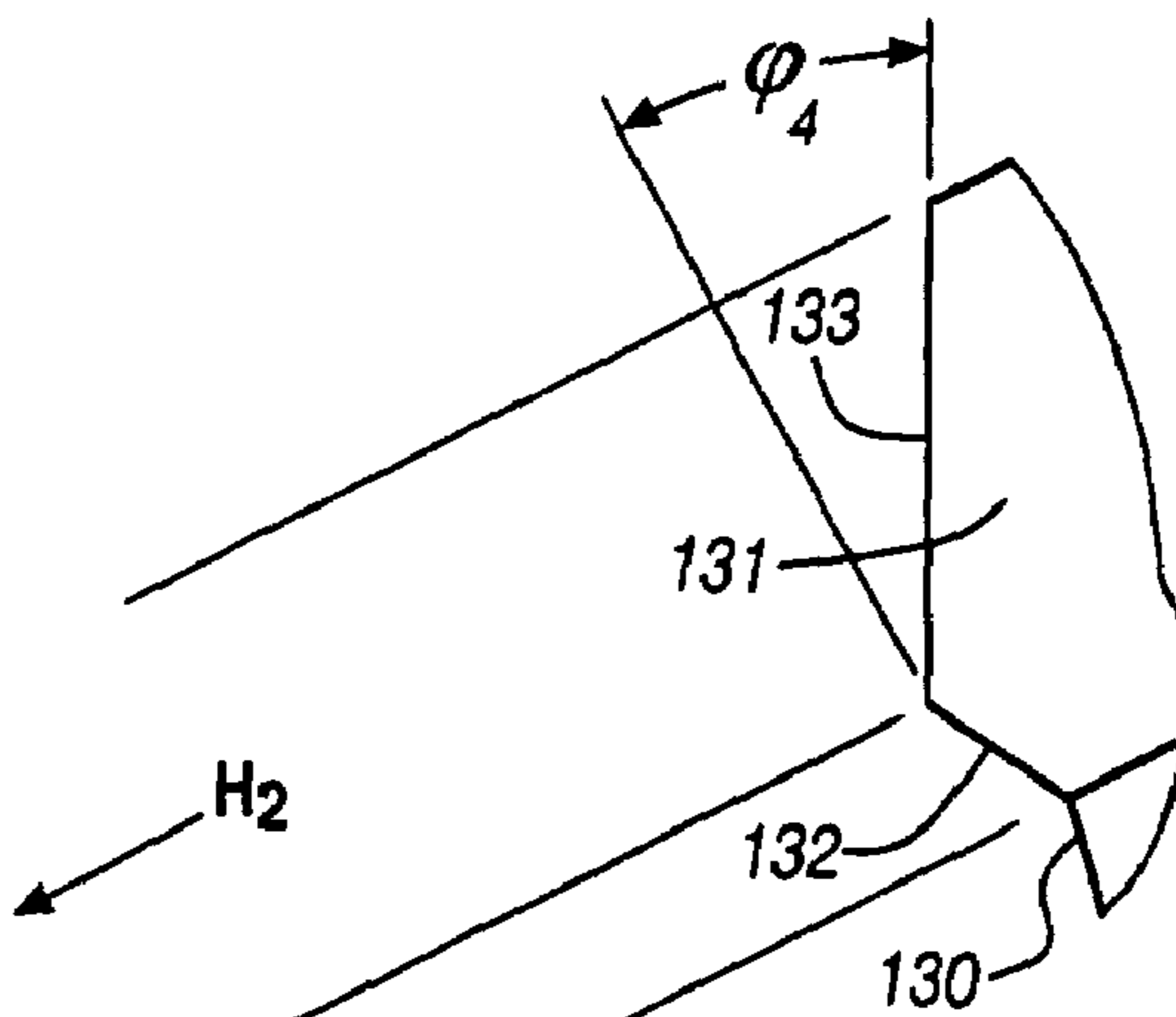
FIGURE 10 VIEW H2 PRIOR ART
