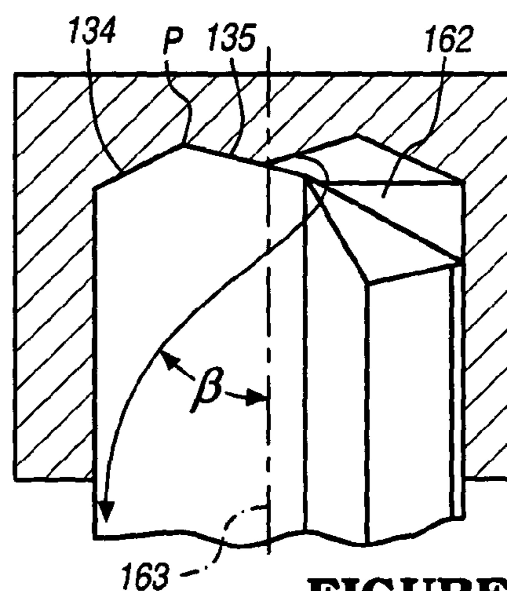
FIGURE 18 PRIOR ART
