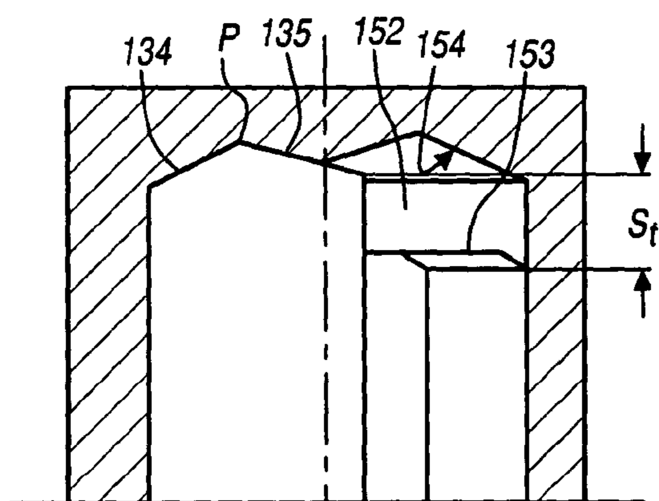
FIGURE 17 PRIOR ART
