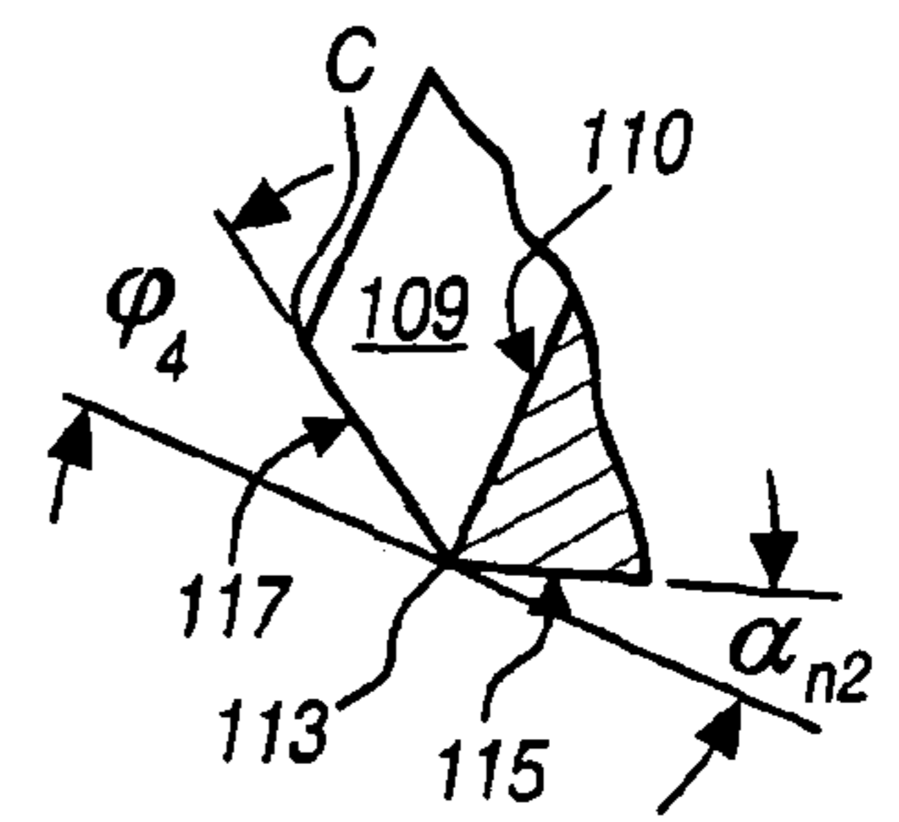
FIGURE 5 SECTION D-D PRIOR ART
