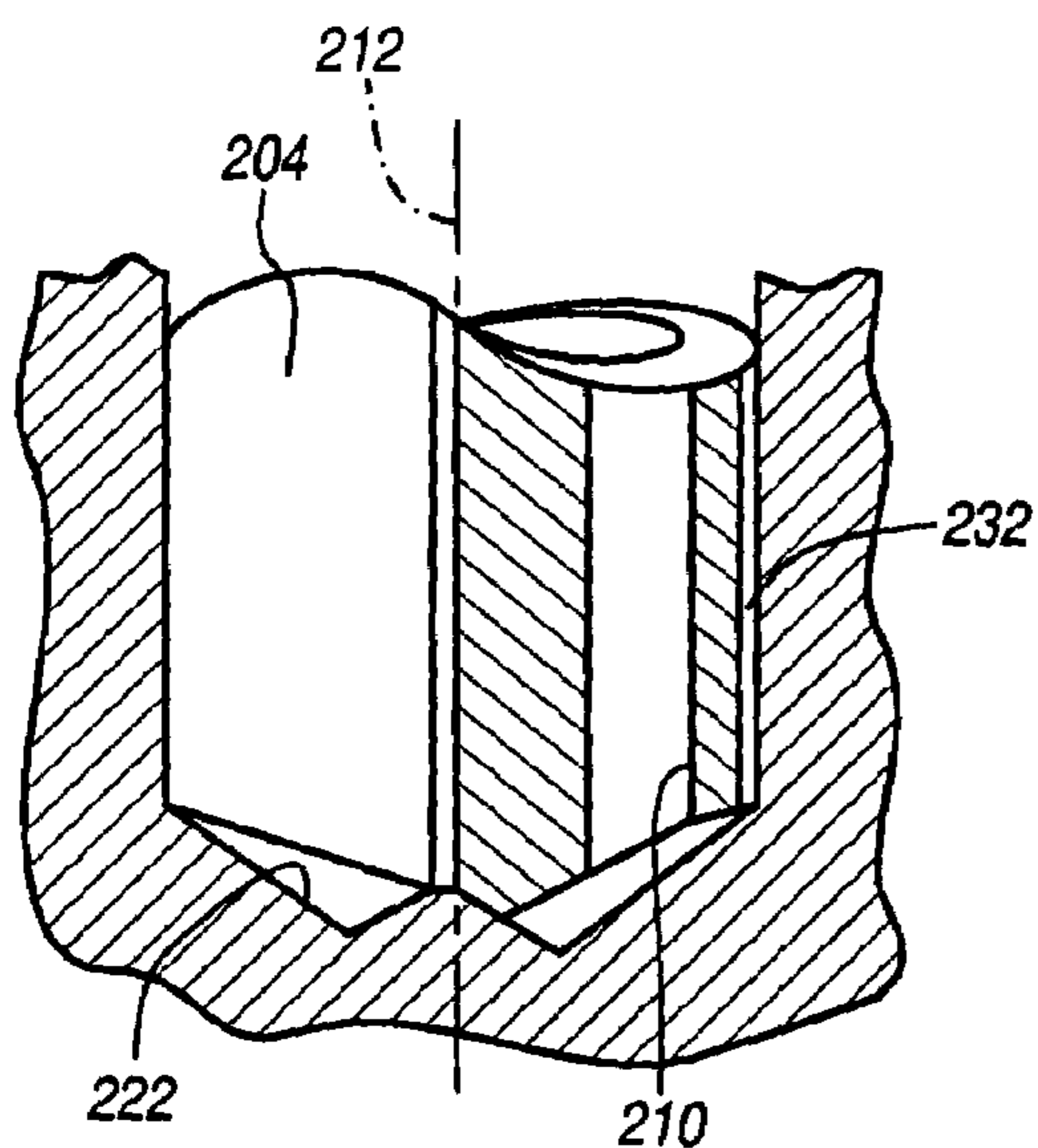
FIGURE 28 SECTION U-U
