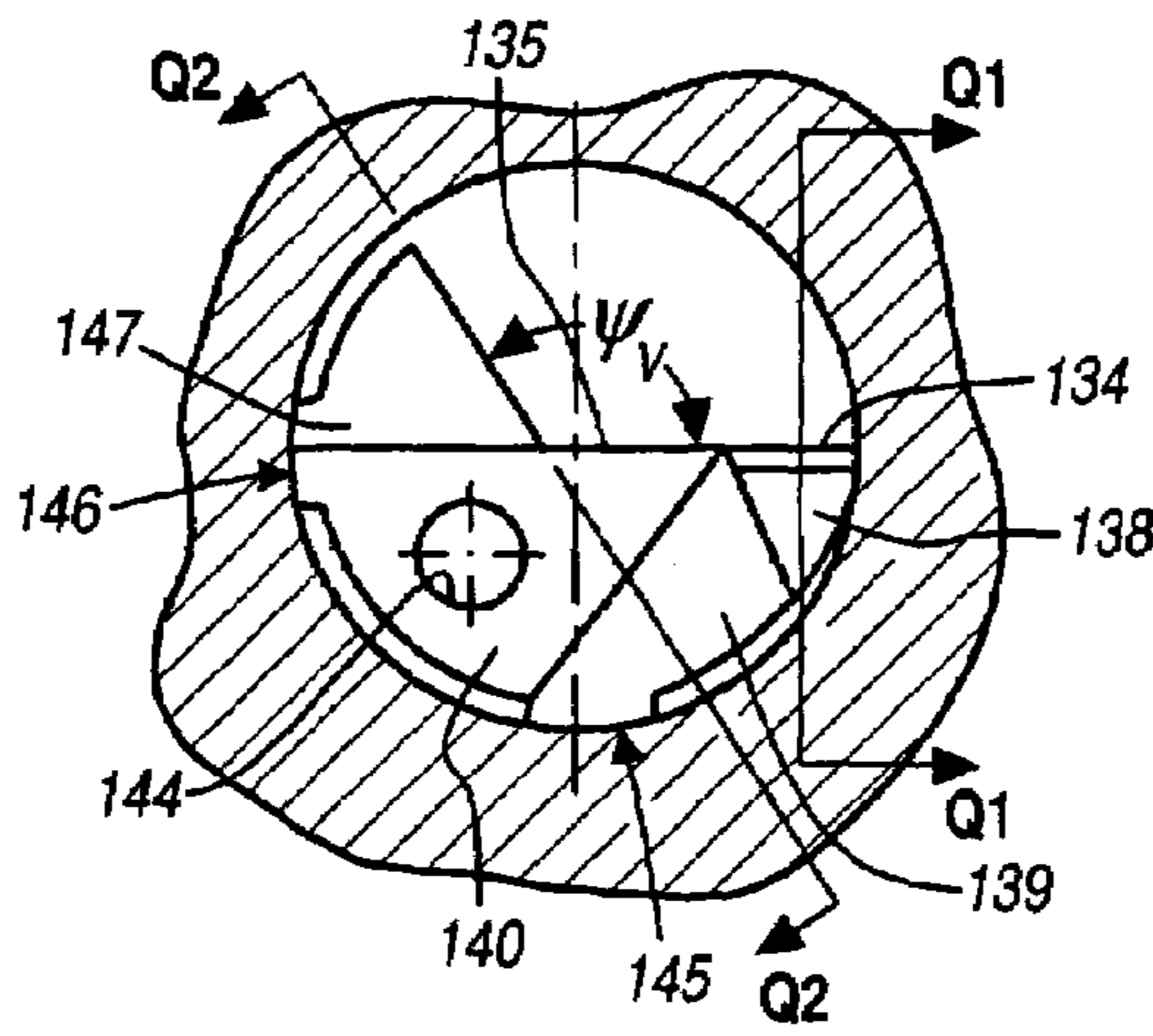
FIGURE 12 PRIOR ART
