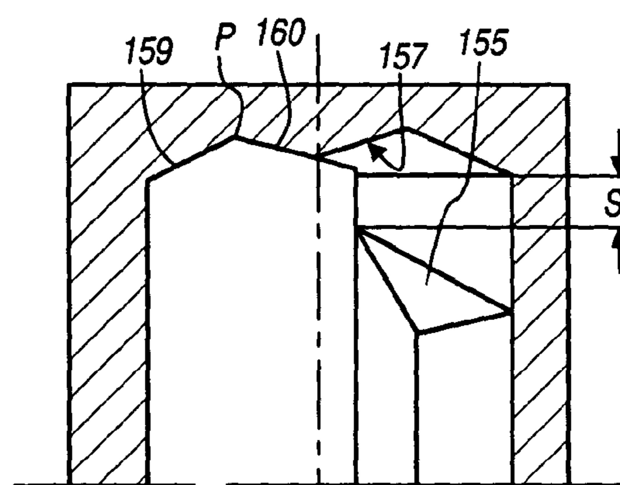
FIGURE 18 PRIOR ART
