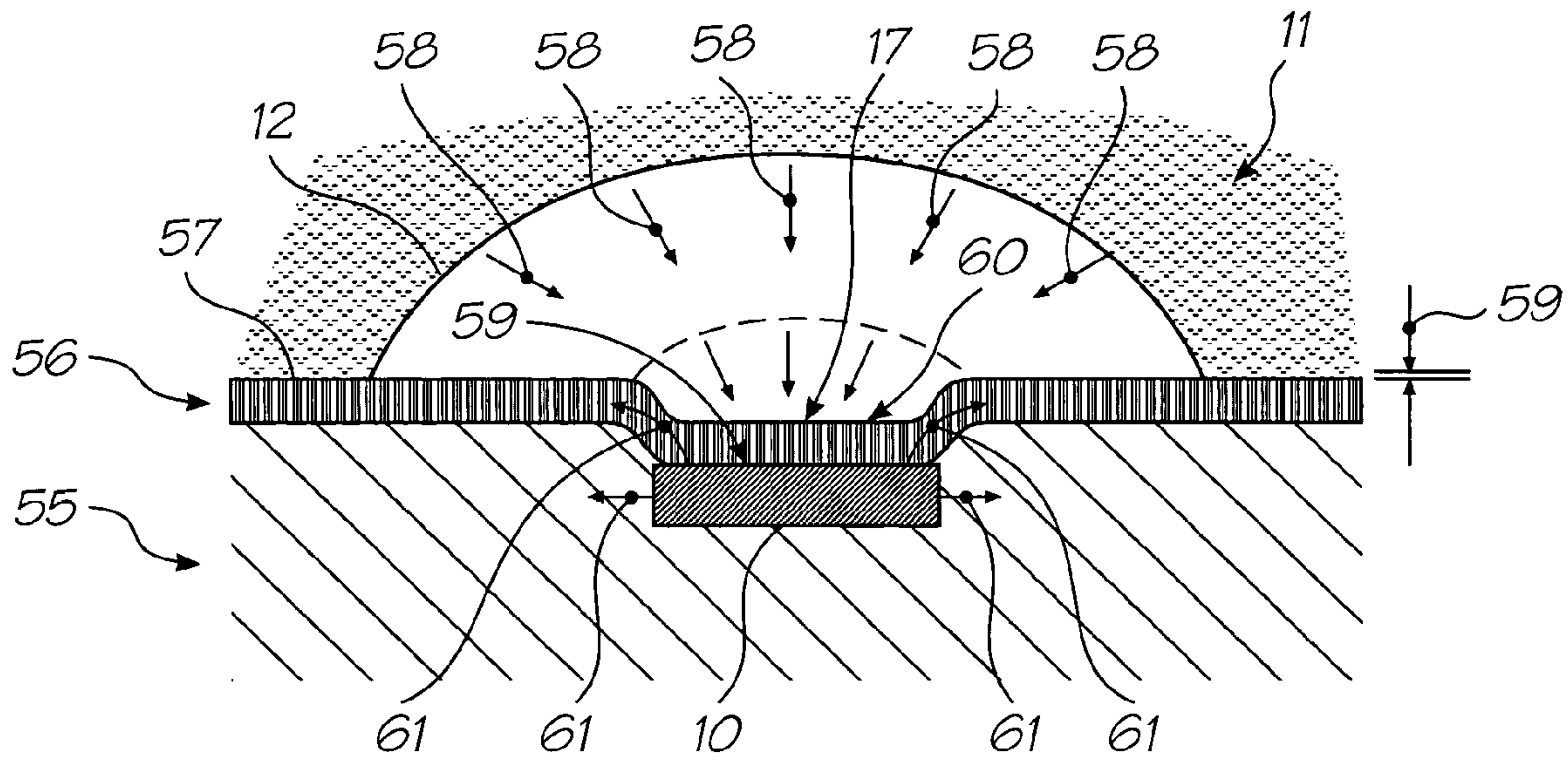
FIG. 57 (PRIOR ART)
