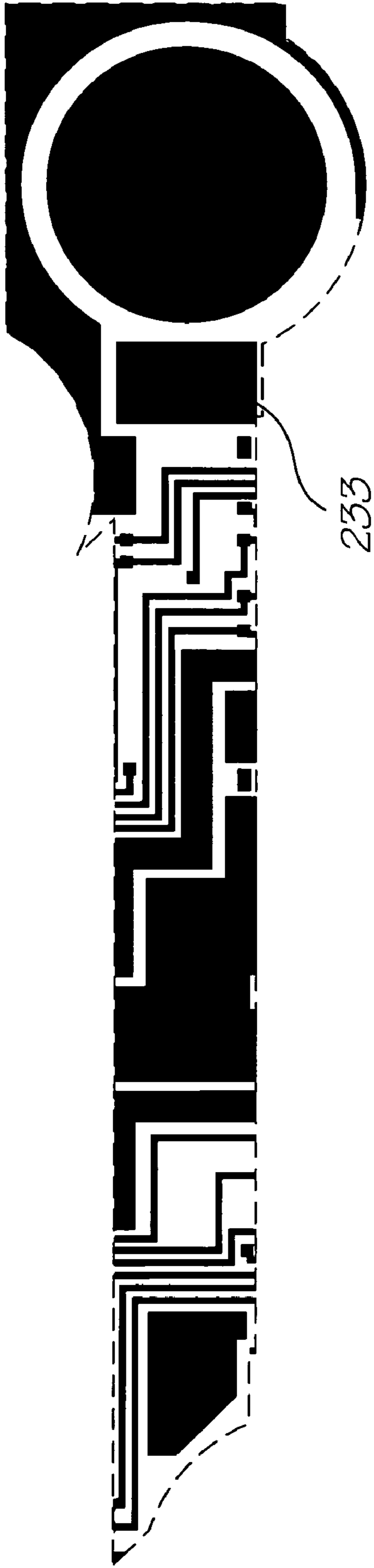
Metal 2 mask
