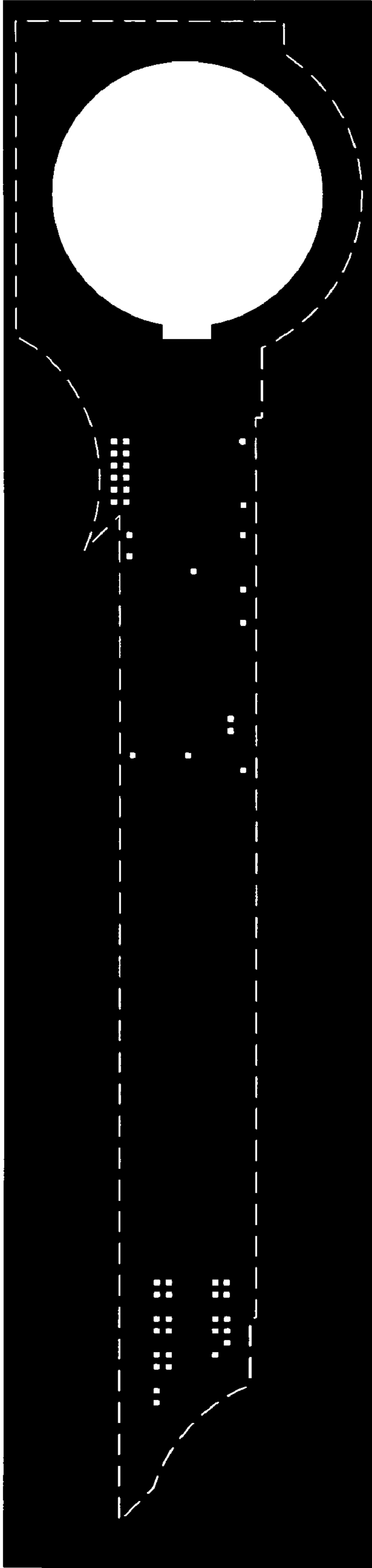
Via 1 mask
